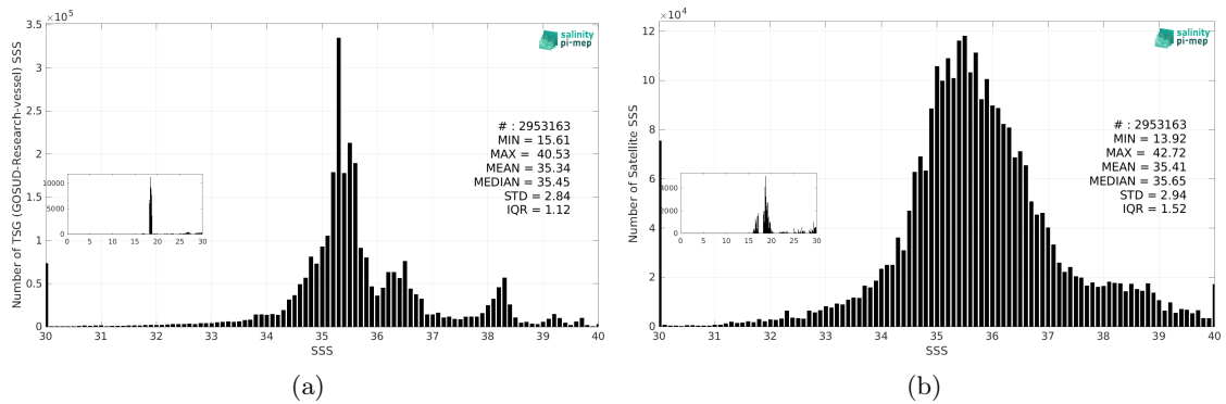
Figure 3: Histograms of SSS from TSG (GOSUD-Research-vessel) (a) and SMAP SSS L2 v5.3 (RSS) (b) considering all match-up pairs per bins of 0.1 over the SMOS coastal zone (<800km) 60N-60S Pi-MEP region and for the full satellite product period.
