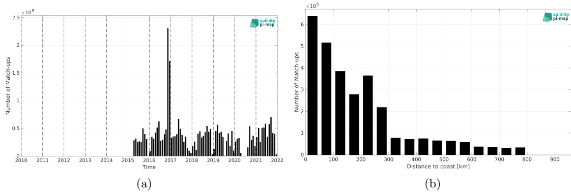
Figure 2: Number of match-ups between TSG (GOSUD-Research-vessel) and SMAP SSS L2 v5.3 (RSS) SSS as a function of time (a) and as function of the distance to coast (b) over the SMOS coastal zone (<800km) 60N-60S Pi-MEP region and for the full satellite product period.
