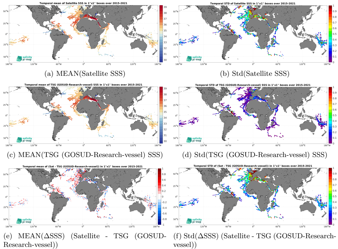
Figure 7: Temporal mean (left) and Std (right) of SSS from SMAP SSS L2 v5.3 (RSS) (top), TSG (GOSUD-Research-vessel) (middle), and of \Delta SSS (Satellite - TSG (GOSUD-Research-vessel)). Only match-up pairs are used to generate these maps.
