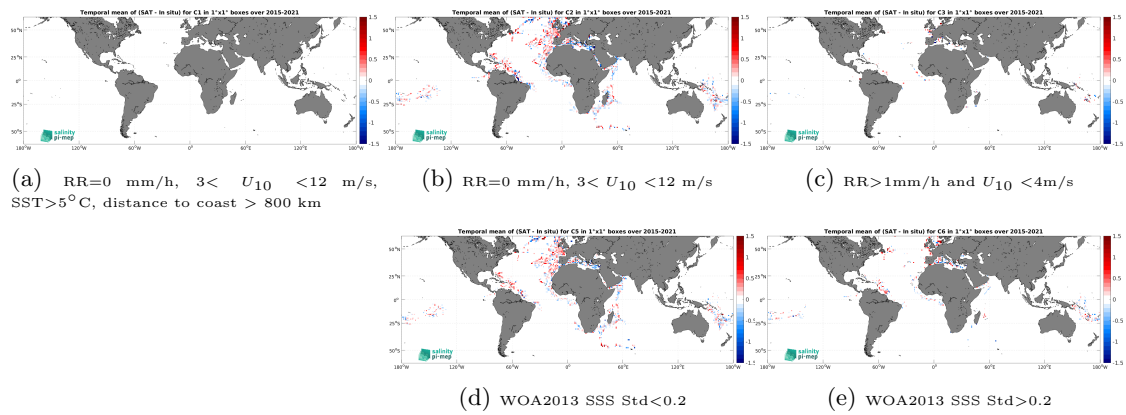
Figure 14: Temporal mean gridded over spatial boxes of size 1^\circ \times 1^\circ of \Delta SSS (SMAP SSS L2 v5.3 (RSS) - TSG (GOSUD-Research-vessel)) for 5 different subdatasets corresponding to:RR=0 mm/h, 3 < U_{10} < 12 m/s, SST > 5^\circ\text{C} , distance to coast > 800 km (a), RR=0 mm/h, 3 < U_{10} < 12 m/s (b), RR > 1 mm/h and U_{10} < 4 m/s (c), WOA2013 SSS Std < 0.2 (d), WOA2013 SSS Std > 0.2 (e).
