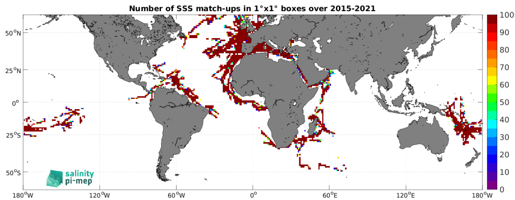
Figure 5: Number of SSS match-ups between TSG (GOSUD-Research-vessel) SSS and the SMAP SSS L2 v5.3 (RSS) SSS product for the SMOS coastal zone (<800km) 60N-60S Pi-MEP region over 1^\circ \times 1^\circ boxes and for the full satellite product period.
