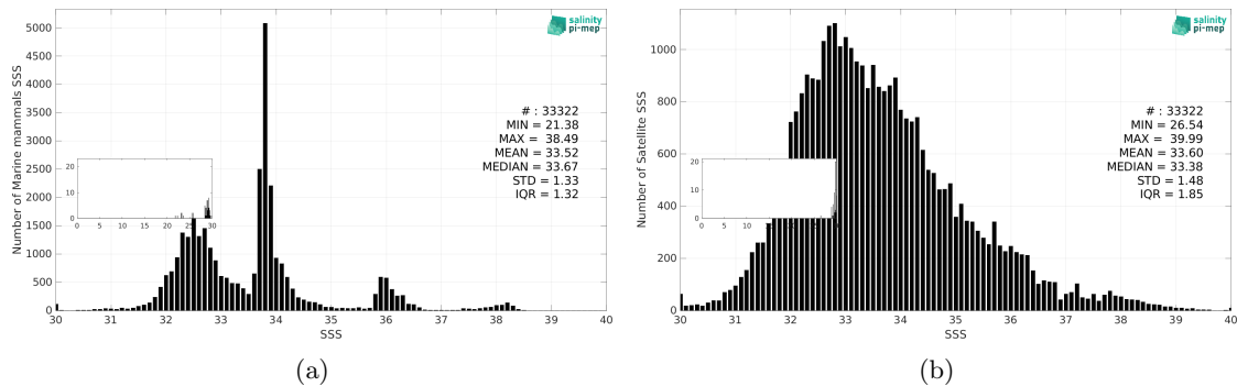
Figure 3: Histograms of SSS from Marine mammals (a) and SMAP SSS L2 v5.3 (RSS) (b) considering all match-up pairs per bins of 0.1 over the SMOS coastal zone (<800km) 60N-60S Pi-MEP region and for the full satellite product period.
