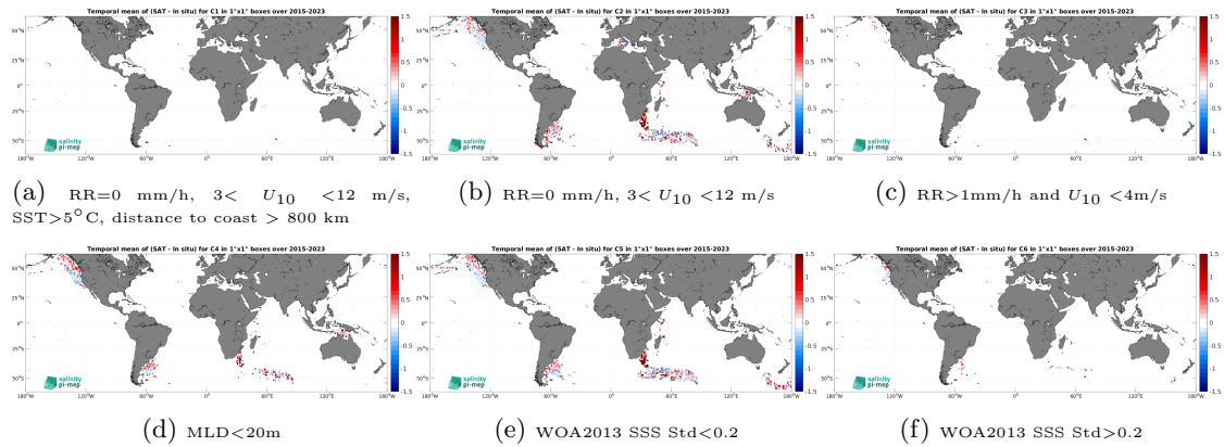
Figure 14: Temporal mean gridded over spatial boxes of size 1^\circ \times 1^\circ of \Delta SSS (SMAP SSS L2 v5.3 (RSS) - Marine mammals) for 6 different subdatasets corresponding to:RR=0 mm/h, 3 < U_{10} < 12 m/s, SST >5^\circ C, distance to coast > 800 km (a), RR=0 mm/h, 3 < U_{10} < 12 m/s (b), RR >1 mm/h and U_{10} < 4 m/s (c),MLD <20 m (d),WOA2013 SSS Std <0.2 (e),WOA2013 SSS Std >0.2 (f).
