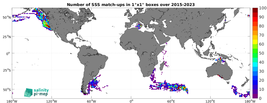
Figure 5: Number of SSS match-ups between Marine mammals SSS and the SMAP SSS L2 v5.3 (RSS) SSS product for the SMOS coastal zone (<800km) 60N-60S Pi-MEP region over 1^\circ \times 1^\circ boxes and for the full satellite product period.
