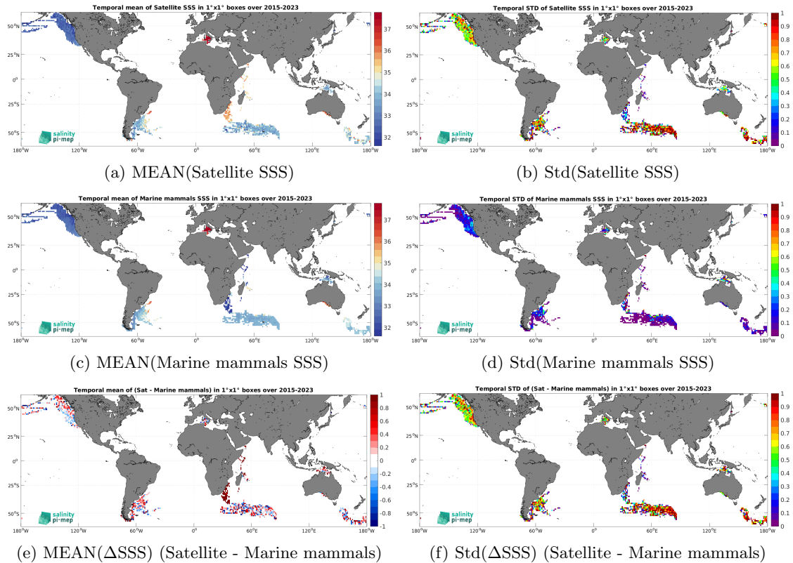
Figure 7: Temporal mean (left) and Std (right) of SSS from SMAP SSS L2 v5.3 (RSS) (top), Marine mammals (middle), and of \Delta SSS (Satellite - Marine mammals). Only match-up pairs are used to generate these maps.
