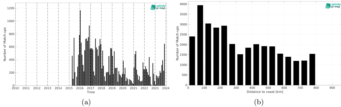
Figure 2: Number of match-ups between Marine mammals and SMAP SSS L2 v5.3 (RSS) SSS as a function of time (a) and as function of the distance to coast (b) over the SMOS coastal zone (<800km) 60N-60S Pi-MEP region and for the full satellite product period.
