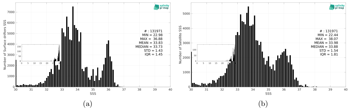
Figure 3: Histograms of SSS from Surface drifters (a) and SMAP SSS L2 v5.3 (RSS) (b) considering all match-up pairs per bins of 0.1 over the SMOS coastal zone (<800km) 60N-60S Pi-MEP region and for the full satellite product period.
