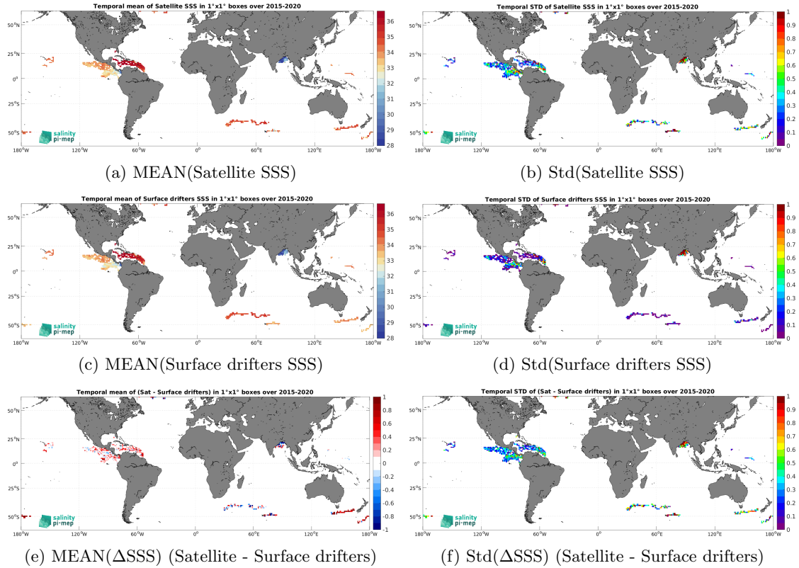
Figure 6: Temporal mean (left) and Std (right) of SSS from SMAP SSS L2 v5.3 (RSS) (top), Surface drifters (middle), and of \Delta SSS (Satellite - Surface drifters). Only match-up pairs are used to generate these maps.
