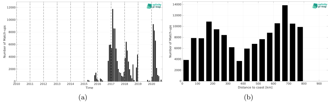
Figure 2: Number of match-ups between Surface drifters and SMAP SSS L2 v5.3 (RSS) SSS as a function of time (a) and as function of the distance to coast (b) over the SMOS coastal zone (<800km) 60N-60S Pi-MEP region and for the full satellite product period.
