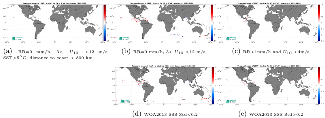
Figure 13: Temporal mean gridded over spatial boxes of size 1^\circ \times 1^\circ of \Delta SSS (SMAP SSS L2 v5.3 (RSS) - Surface drifters) for 5 different subdatasets corresponding to:RR=0 mm/h, 3 < U_{10} < 12 m/s, SST >5^\circ\text{C} , distance to coast > 800 km (a), RR=0 mm/h, 3 < U_{10} < 12 m/s (b), RR >1 mm/h and U_{10} < 4 m/s (c), WOA2013 SSS Std <0.2 (d), WOA2013 SSS Std >0.2 (e).
