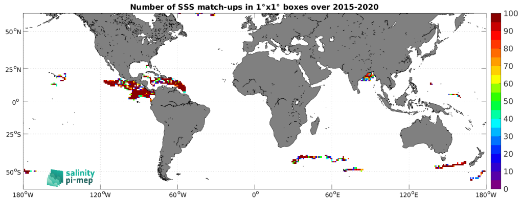
Figure 4: Number of SSS match-ups between Surface drifters SSS and the SMAP SSS L2 v5.3 (RSS) SSS product for the SMOS coastal zone (<800km) 60N-60S Pi-MEP region over 1^\circ \times 1^\circ boxes and for the full satellite product period.
