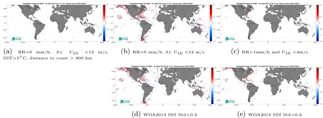
Figure 14: Temporal mean gridded over spatial boxes of size 1^\circ \times 1^\circ of \Delta\text{SSS} (SMAP SSS L2 v5.3 - 40 km (RSS) - TSG (SAMOS)) for 5 different subdatasets corresponding to:RR=0 mm/h, 3 < U_{10} < 12 m/s, SST>5°C, distance to coast > 800 km (a), RR=0 mm/h, 3 < U_{10} < 12 m/s (b), RR>1mm/h and U_{10} < 4 m/s (c), WOA2013 SSS Std<0.2 (d), WOA2013 SSS Std>0.2 (e).
