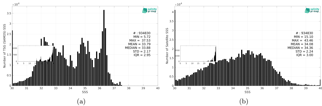
Figure 3: Histograms of SSS from TSG (SAMOS) (a) and SMAP SSS L2 v5.3 - 40 km (RSS) (b) considering all match-up pairs per bins of 0.1 over the SMOS coastal zone (<800km) 60N-60S Pi-MEP region and for the full satellite product period.
