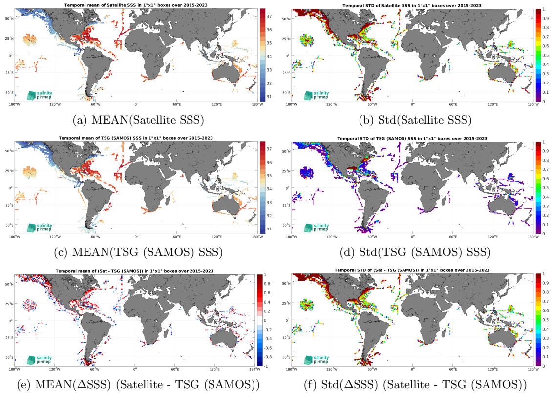
Figure 7: Temporal mean (left) and Std (right) of SSS from SMAP SSS L2 v5.3 - 40 km (RSS) (top), TSG (SAMOS) (middle), and of \Delta SSS (Satellite - TSG (SAMOS)). Only match-up pairs are used to generate these maps.
