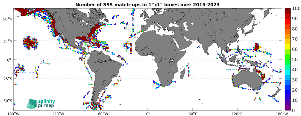
Figure 5: Number of SSS match-ups between TSG (SAMOS) SSS and the SMAP SSS L2 v5.3 - 40 km (RSS) SSS product for the SMOS coastal zone (<800km) 60N-60S Pi-MEP region over 1^\circ \times 1^\circ boxes and for the full satellite product period.
