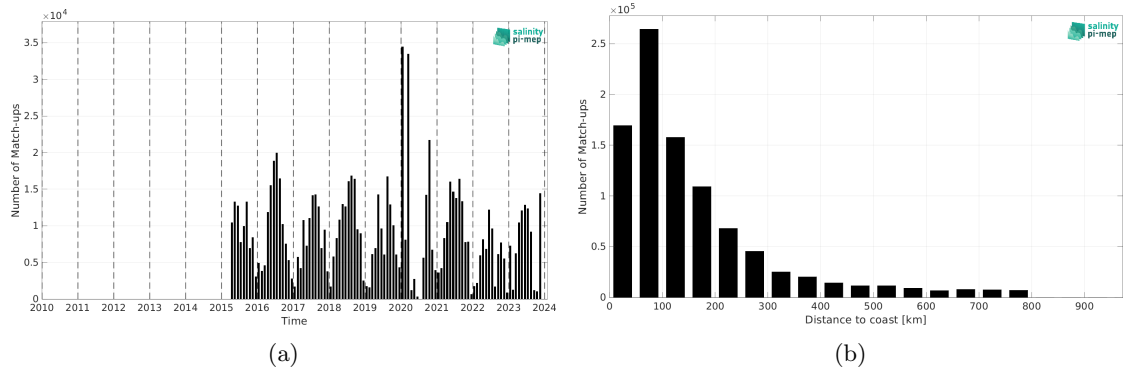
Figure 2: Number of match-ups between TSG (SAMOS) and SMAP SSS L2 v5.3 - 40 km (RSS) SSS as a function of time (a) and as function of the distance to coast (b) over the SMOS coastal zone (<800km) 60N-60S Pi-MEP region and for the full satellite product period.
