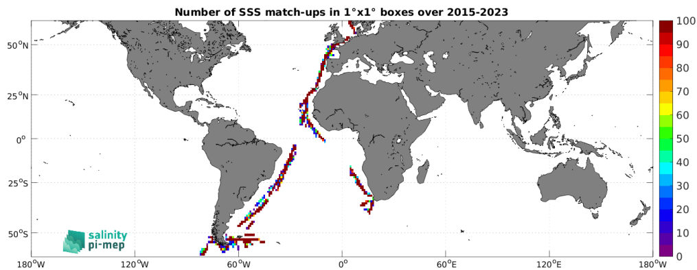
Figure 5: Number of SSS match-ups between TSG (Polarstern) SSS and the SMAP SSS L2 v5.3 - 40 km (RSS) SSS product for the SMOS coastal zone (<800km) 60N-60S Pi-MEP region over 1^\circ \times 1^\circ boxes and for the full satellite product period.
