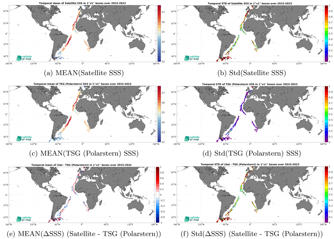
Figure 7: Temporal mean (left) and Std (right) of SSS from SMAP SSS L2 v5.3 - 40 km (RSS) (top), TSG (Polarstern) (middle), and of \Delta SSS (Satellite - TSG (Polarstern)). Only match-up pairs are used to generate these maps.
