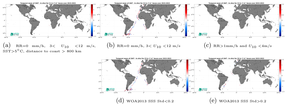
Figure 14: Temporal mean gridded over spatial boxes of size 1^\circ \times 1^\circ of \Delta\text{SSS} (SMAP SSS L2 v5.3 - 40 km (RSS) - TSG (Polarstern)) for 5 different subdatasets corresponding to:RR=0 mm/h, 3 < U_{10} < 12 m/s, SST >5^\circ\text{C} , distance to coast > 800 km (a), RR=0 mm/h, 3 < U_{10} < 12 m/s (b), RR >1 mm/h and U_{10} < 4 m/s (c), WOA2013 SSS Std <0.2 (d), WOA2013 SSS Std >0.2 (e).
