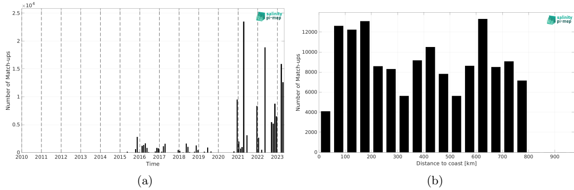
Figure 2: Number of match-ups between TSG (Polarstern) and SMAP SSS L2 v5.3 - 40 km (RSS) SSS as a function of time (a) and as function of the distance to coast (b) over the SMOS coastal zone (<800km) 60N-60S Pi-MEP region and for the full satellite product period.
