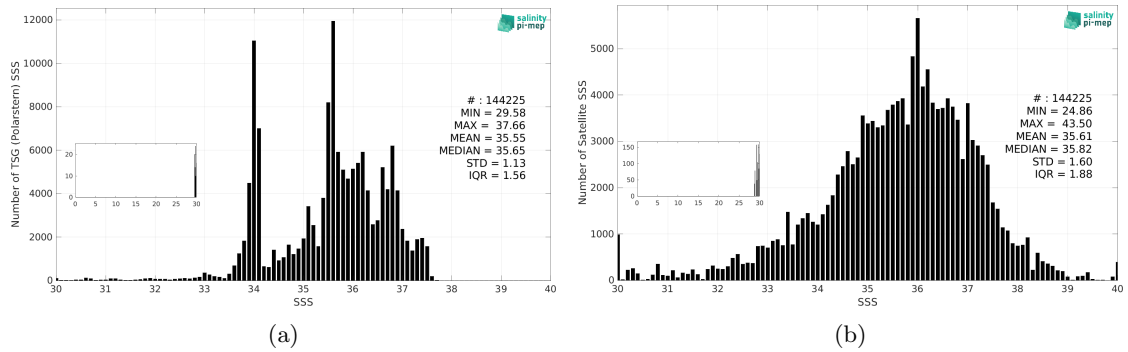
Figure 3: Histograms of SSS from TSG (Polarstern) (a) and SMAP SSS L2 v5.3 - 40 km (RSS) (b) considering all match-up pairs per bins of 0.1 over the SMOS coastal zone (<800km) 60N-60S Pi-MEP region and for the full satellite product period.
