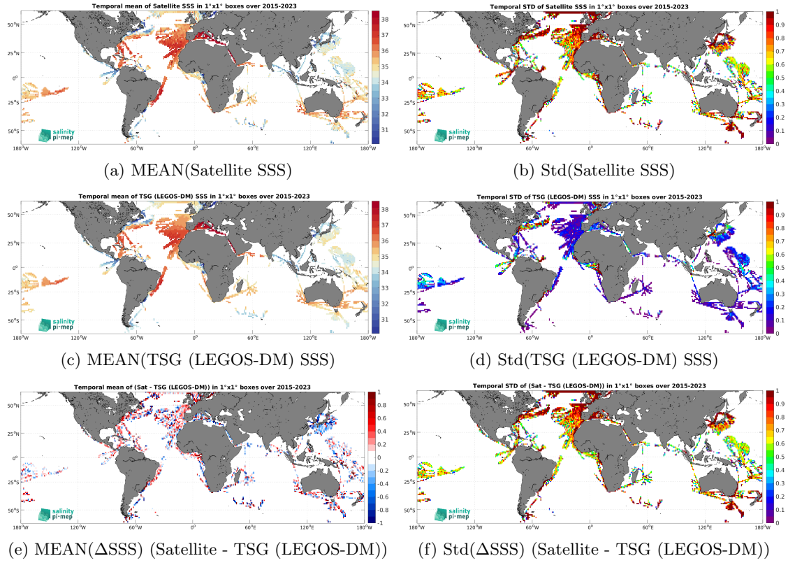
Figure 7: Temporal mean (left) and Std (right) of SSS from SMAP SSS L2 v5.3 - 40 km (RSS) (top), TSG (LEGOS-DM) (middle), and of \Delta SSS (Satellite - TSG (LEGOS-DM)). Only match-up pairs are used to generate these maps.
