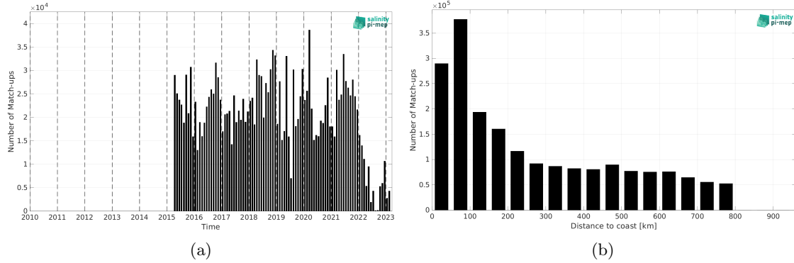
Figure 2: Number of match-ups between TSG (LEGOS-DM) and SMAP SSS L2 v5.3 - 40 km (RSS) SSS as a function of time (a) and as function of the distance to coast (b) over the SMOS coastal zone (<800km) 60N-60S Pi-MEP region and for the full satellite product period.
