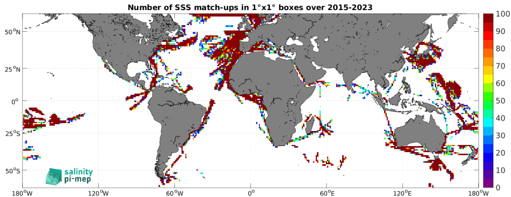
Figure 5: Number of SSS match-ups between TSG (LEGOS-DM) SSS and the SMAP SSS L2 v5.3 - 40 km (RSS) SSS product for the SMOS coastal zone ( <800\text{km} ) 60\text{N} - 60\text{S} Pi-MEP region over 1^\circ \times 1^\circ boxes and for the full satellite product period.
