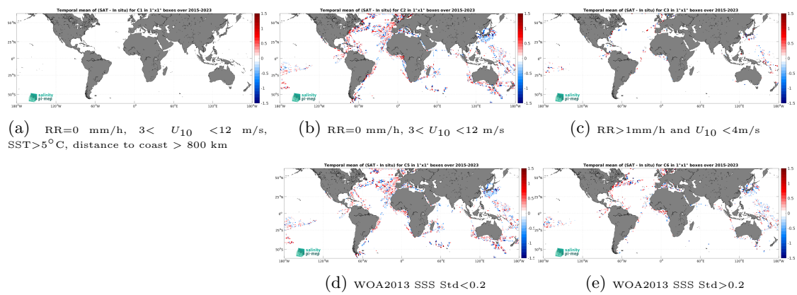
Figure 14: Temporal mean gridded over spatial boxes of size 1^\circ \times 1^\circ of \Delta\text{SSS} (SMAP SSS L2 v5.3 - 40 km (RSS) - TSG (LEGOS-DM)) for 5 different subdatasets corresponding to:RR=0 mm/h, 3 < U_{10} < 12 m/s, SST >5^\circ\text{C} , distance to coast > 800 km (a), RR=0 mm/h, 3 < U_{10} < 12 m/s (b), RR >1 mm/h and U_{10} < 4 m/s (c), WOA2013 SSS Std <0.2 (d), WOA2013 SSS Std >0.2 (e).
