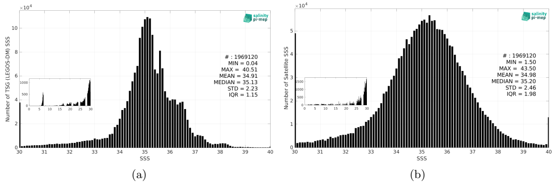
Figure 3: Histograms of SSS from TSG (LEGOS-DM) (a) and SMAP SSS L2 v5.3 - 40 km (RSS) (b) considering all match-up pairs per bins of 0.1 over the SMOS coastal zone (<800km) 60N-60S Pi-MEP region and for the full satellite product period.
