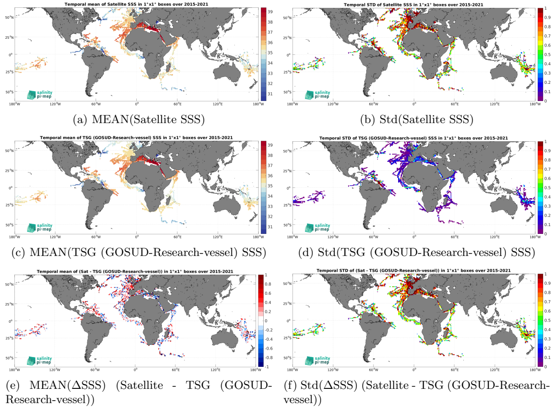
Figure 7: Temporal mean (left) and Std (right) of SSS from SMAP SSS L2 v5.3 - 40 km (RSS) (top), TSG (GOSUD-Research-vessel) (middle), and of \Delta SSS (Satellite - TSG (GOSUD-Research-vessel)). Only match-up pairs are used to generate these maps.
