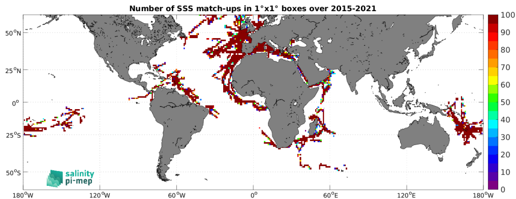
Figure 5: Number of SSS match-ups between TSG (GOSUD-Research-vessel) SSS and the SMAP SSS L2 v5.3 - 40 km (RSS) SSS product for the SMOS coastal zone (<800km) 60N-60S Pi-MEP region over 1^\circ \times 1^\circ boxes and for the full satellite product period.
