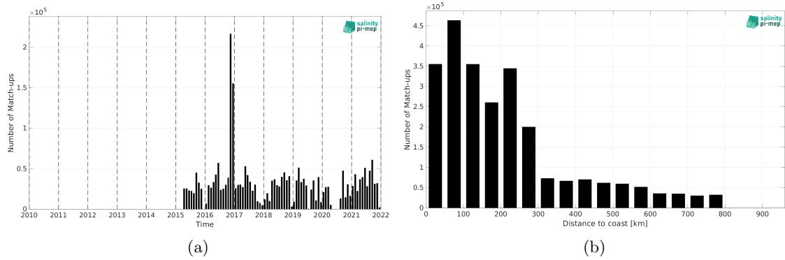
Figure 2: Number of match-ups between TSG (GOSUD-Research-vessel) and SMAP SSS L2 v5.3 - 40 km (RSS) SSS as a function of time (a) and as function of the distance to coast (b) over the SMOS coastal zone (<800km) 60N-60S Pi-MEP region and for the full satellite product period.
