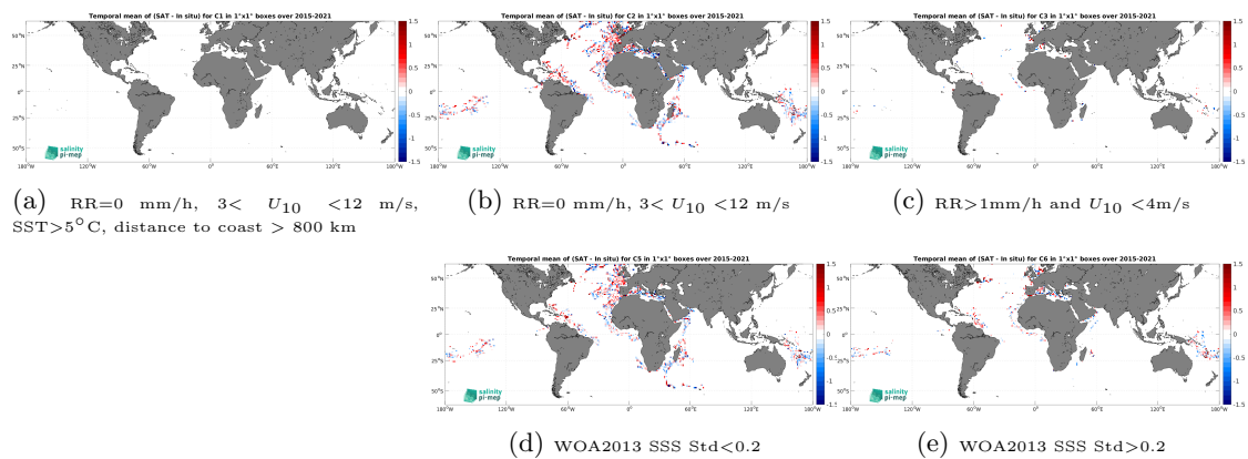
Figure 14: Temporal mean gridded over spatial boxes of size 1^\circ \times 1^\circ of \Delta SSS (SMAP SSS L2 v5.3 - 40 km (RSS) - TSG (GOSUD-Research-vessel)) for 5 different subdatasets corresponding to:RR=0 mm/h, 3 < U_{10} < 12 m/s, SST >5^\circ\text{C} , distance to coast > 800 km (a), RR=0 mm/h, 3 < U_{10} < 12 m/s (b), RR >1 mm/h and U_{10} < 4 m/s (c), WOA2013 SSS Std <0.2 (d), WOA2013 SSS Std >0.2 (e).
