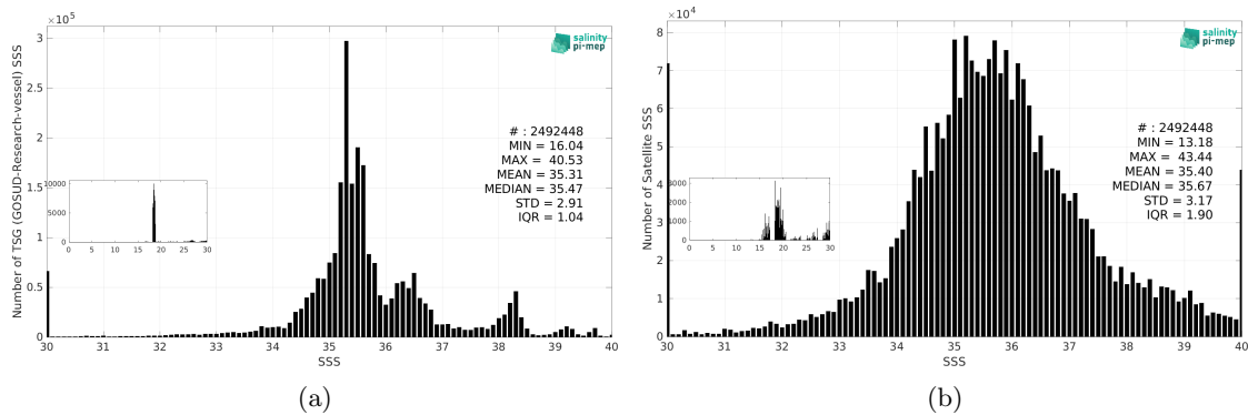
Figure 3: Histograms of SSS from TSG (GOSUD-Research-vessel) (a) and SMAP SSS L2 v5.3 - 40 km (RSS) (b) considering all match-up pairs per bins of 0.1 over the SMOS coastal zone (<800km) 60N-60S Pi-MEP region and for the full satellite product period.
