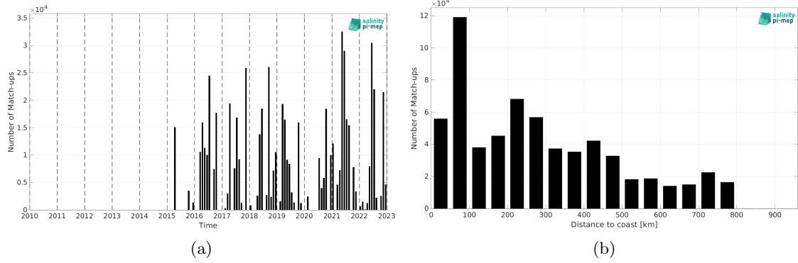
Figure 2: Number of match-ups between TSG (CSIC-UTM) and SMAP SSS L2 v5.3 - 40 km (RSS) SSS as a function of time (a) and as function of the distance to coast (b) over the SMOS coastal zone (<800km) 60N-60S Pi-MEP region and for the full satellite product period.
