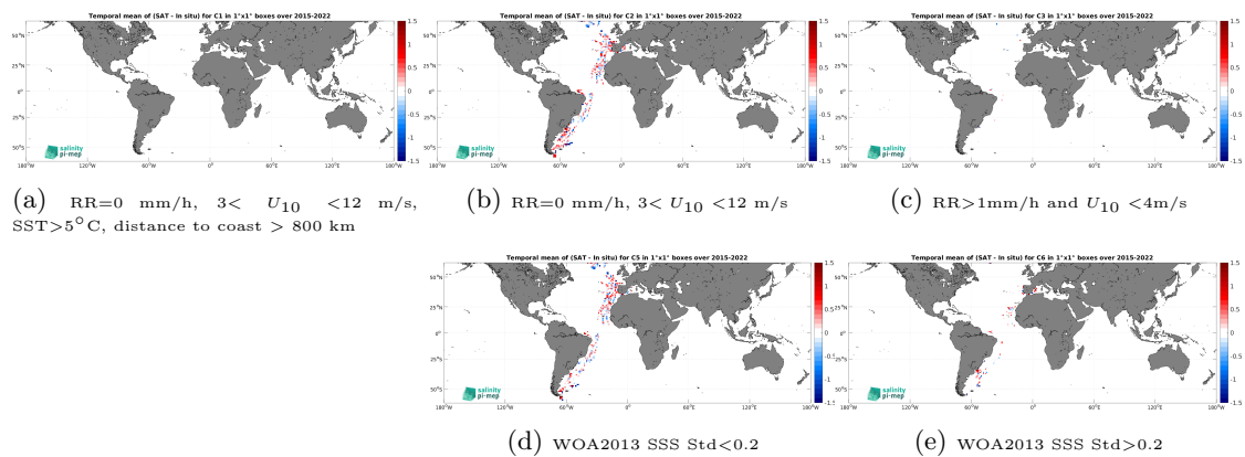
Figure 14: Temporal mean gridded over spatial boxes of size 1^\circ \times 1^\circ of \Delta\text{SSS} (SMAP SSS L2 v5.3 - 40 km (RSS) - TSG (CSIC-UTM)) for 5 different subdatasets corresponding to:RR=0 mm/h, 3 < U_{10} < 12 m/s, SST>5°C, distance to coast > 800 km (a), RR=0 mm/h, 3 < U_{10} < 12 m/s (b), RR>1mm/h and U_{10} < 4 m/s (c), WOA2013 SSS Std<0.2 (d), WOA2013 SSS Std>0.2 (e).
