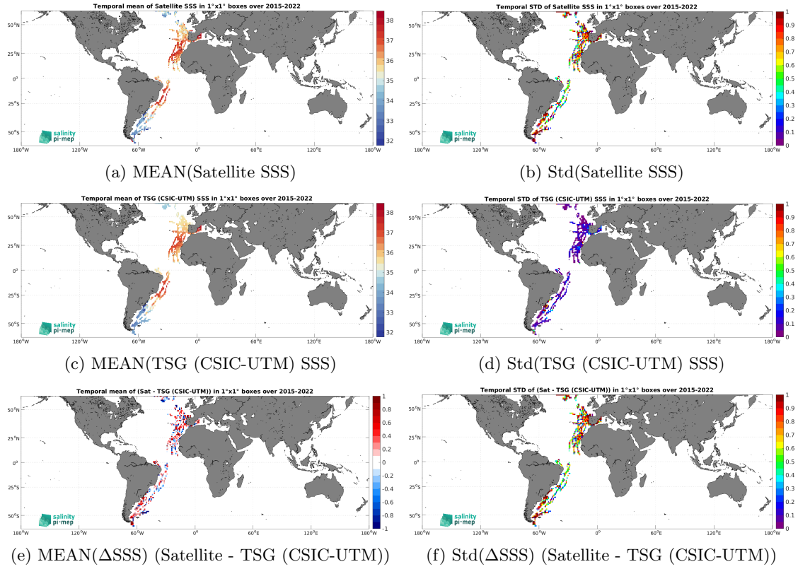
Figure 7: Temporal mean (left) and Std (right) of SSS from SMAP SSS L2 v5.3 - 40 km (RSS) (top), TSG (CSIC-UTM) (middle), and of \Delta SSS (Satellite - TSG (CSIC-UTM)). Only match-up pairs are used to generate these maps.
