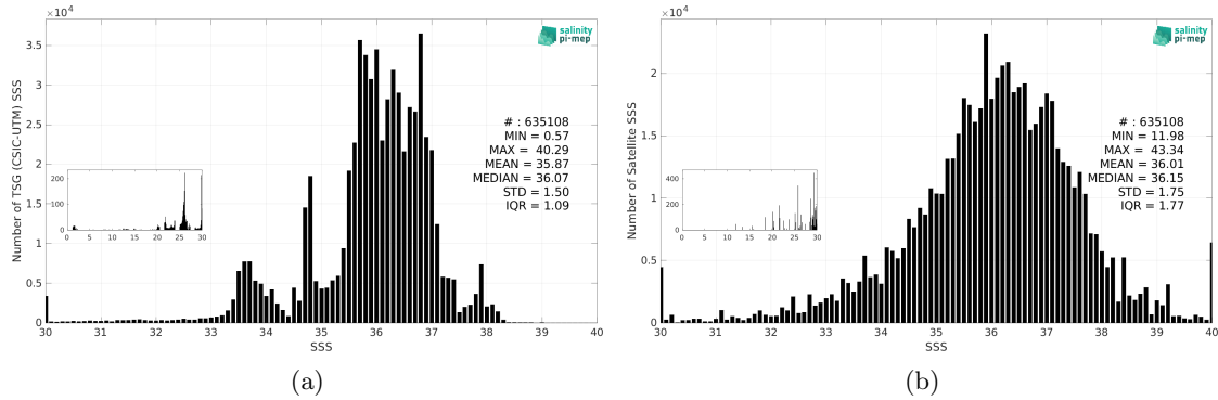
Figure 3: Histograms of SSS from TSG (CSIC-UTM) (a) and SMAP SSS L2 v5.3 - 40 km (RSS) (b) considering all match-up pairs per bins of 0.1 over the SMOS coastal zone (<800km) 60N-60S Pi-MEP region and for the full satellite product period.
