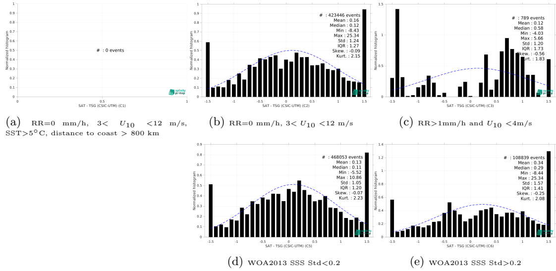
Figure 15: Normalized histogram of \Delta SSS (SMAP SSS L2 v5.3 - 40 km (RSS) - TSG (CSIC-UTM)) for 5 different subdatasets corresponding to: RR=0 mm/h, 3 < U_{10} < 12 m/s, SST > 5°C, distance to coast > 800 km (a), RR=0 mm/h, 3 < U_{10} < 12 m/s (b), RR > 1mm/h and U_{10} < 4 m/s (c), WOA2013 SSS Std < 0.2 (d), WOA2013 SSS Std > 0.2 (e).
