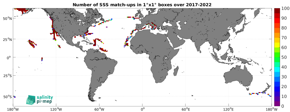
Figure 5: Number of SSS match-ups between Saildrone SSS and the SMAP SSS L2 v5.3 - 40 km (RSS) SSS product for the SMOS coastal zone ( <800\text{km} ) 60N-60S Pi-MEP region over 1^\circ \times 1^\circ boxes and for the full satellite product period.
