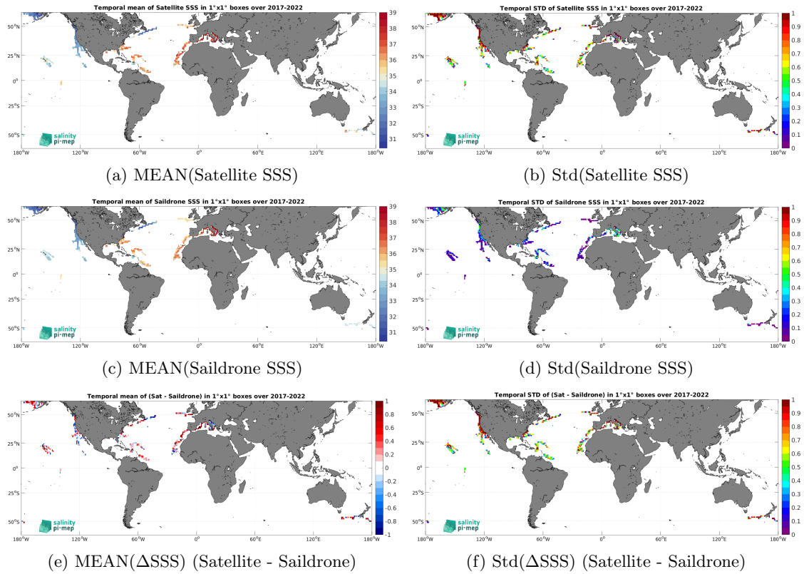
Figure 7: Temporal mean (left) and Std (right) of SSS from SMAP SSS L2 v5.3 - 40 km (RSS) (top), Saildrone (middle), and of \Delta SSS (Satellite - Saildrone). Only match-up pairs are used to generate these maps.
