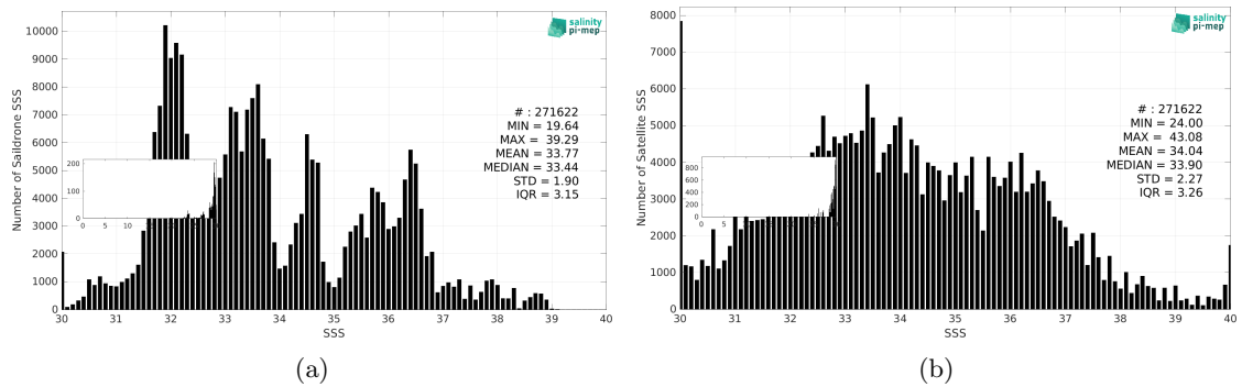
Figure 3: Histograms of SSS from Sailldrone (a) and SMAP SSS L2 v5.3 - 40 km (RSS) (b) considering all match-up pairs per bins of 0.1 over the SMOS coastal zone (<800km) 60N-60S Pi-MEP region and for the full satellite product period.
