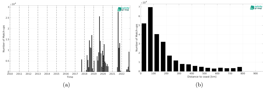
Figure 2: Number of match-ups between Sailldrone and SMAP SSS L2 v5.3 - 40 km (RSS) SSS as a function of time (a) and as function of the distance to coast (b) over the SMOS coastal zone (<800km) 60N-60S Pi-MEP region and for the full satellite product period.
