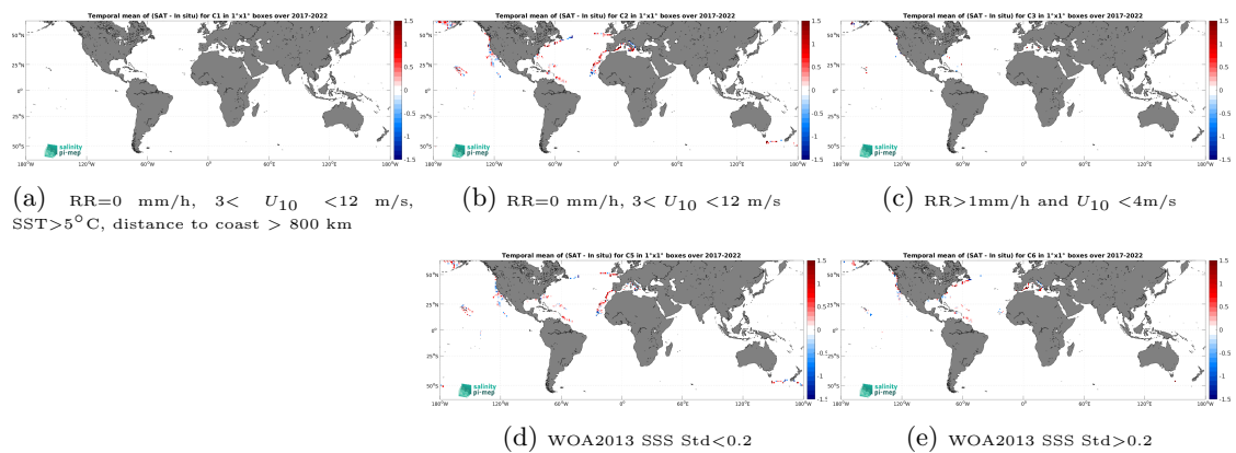
Figure 14: Temporal mean gridded over spatial boxes of size 1^\circ \times 1^\circ of \Delta SSS (SMAP SSS L2 v5.3 - 40 km (RSS) - Sailydrone) for 5 different subdatasets corresponding to:RR=0 mm/h, 3 < U_{10} < 12 m/s, SST >5^\circ\text{C} , distance to coast > 800 km (a), RR=0 mm/h, 3 < U_{10} < 12 m/s (b), RR >1 mm/h and U_{10} < 4 m/s (c), WOA2013 SSS Std <0.2 (d), WOA2013 SSS Std >0.2 (e).
