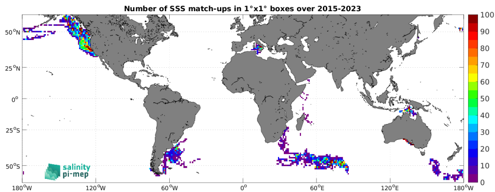
Figure 5: Number of SSS match-ups between Marine mammals SSS and the SMAP SSS L2 v5.3 - 40 km (RSS) SSS product for the SMOS coastal zone (<800km) 60N-60S Pi-MEP region over 1^\circ \times 1^\circ boxes and for the full satellite product period.
