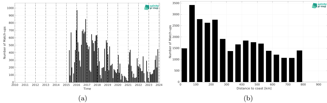
Figure 2: Number of match-ups between Marine mammals and SMAP SSS L2 v5.3 - 40 km (RSS) SSS as a function of time (a) and as function of the distance to coast (b) over the SMOS coastal zone (<800km) 60N-60S Pi-MEP region and for the full satellite product period.
