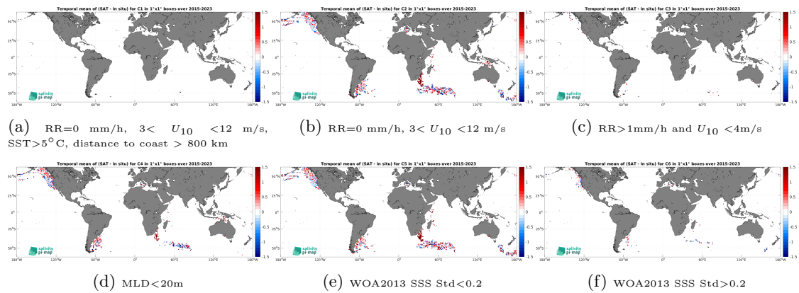
Figure 14: Temporal mean gridded over spatial boxes of size 1^\circ \times 1^\circ of \Delta SSS (SMAP SSS L2 v5.3 - 40 km (RSS) - Marine mammals) for 6 different subdatasets corresponding to:RR=0 mm/h, 3 < U_{10} < 12 m/s, SST > 5^\circ\text{C} , distance to coast > 800 km (a), RR=0 mm/h, 3 < U_{10} < 12 m/s (b), RR > 1 mm/h and U_{10} < 4 m/s (c),MLD < 20 m (d),WOA2013 SSS Std < 0.2 (e),WOA2013 SSS Std > 0.2 (f).
