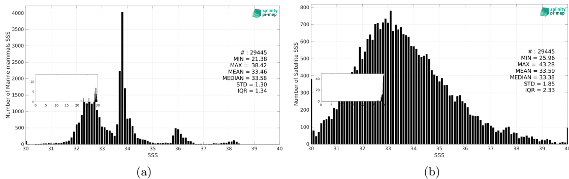
Figure 3: Histograms of SSS from Marine mammals (a) and SMAP SSS L2 v5.3 - 40 km (RSS) (b) considering all match-up pairs per bins of 0.1 over the SMOS coastal zone (<800km) 60N-60S Pi-MEP region and for the full satellite product period.
