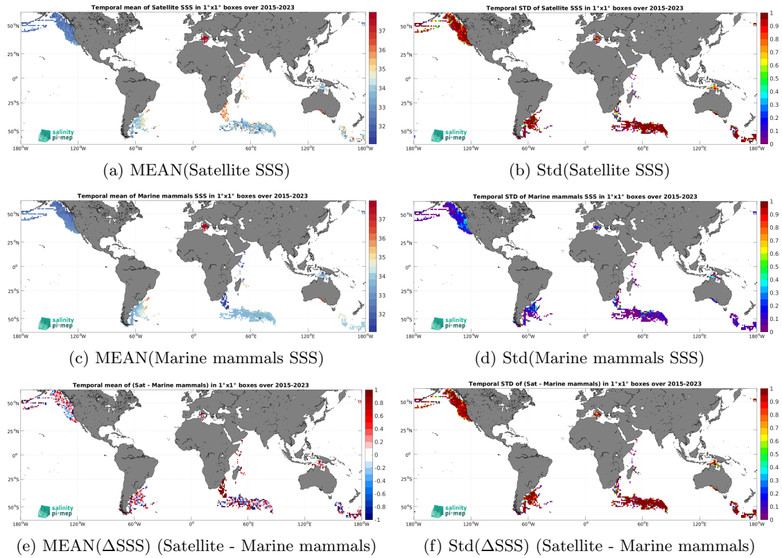
Figure 7: Temporal mean (left) and Std (right) of SSS from SMAP SSS L2 v5.3 - 40 km (RSS) (top), Marine mammals (middle), and of \Delta SSS (Satellite - Marine mammals). Only match-up pairs are used to generate these maps.
