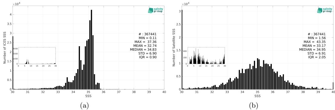
Figure 3: Histograms of SSS from ICES (a) and SMAP SSS L2 v5.3 - 40 km (RSS) (b) considering all match-up pairs per bins of 0.1 over the SMOS coastal zone (<800km) 60N-60S Pi-MEP region and for the full satellite product period.
