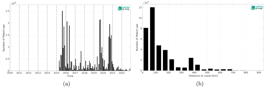
Figure 2: Number of match-ups between ICES and SMAP SSS L2 v5.3 - 40 km (RSS) SSS as a function of time (a) and as function of the distance to coast (b) over the SMOS coastal zone (<800km) 60N-60S Pi-MEP region and for the full satellite product period.
