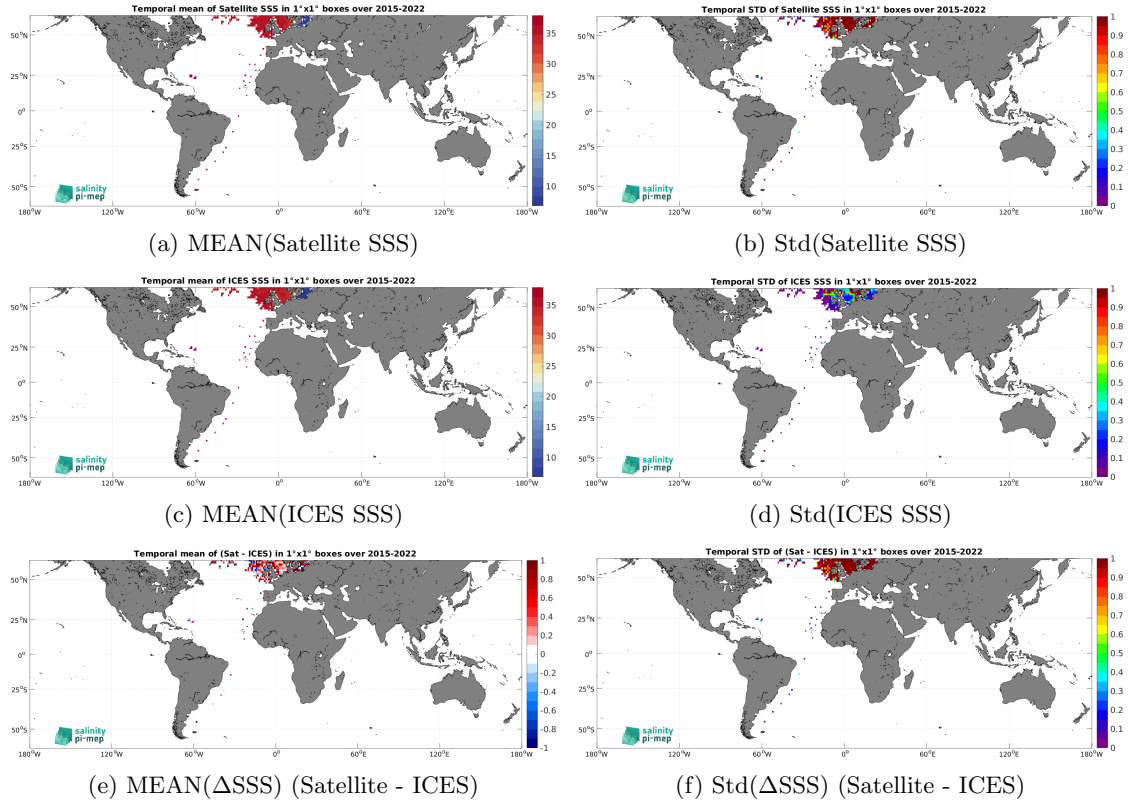
Figure 7: Temporal mean (left) and Std (right) of SSS from SMAP SSS L2 v5.3 - 40 km (RSS) (top), ICES (middle), and of \Delta SSS (Satellite - ICES). Only match-up pairs are used to generate these maps.
