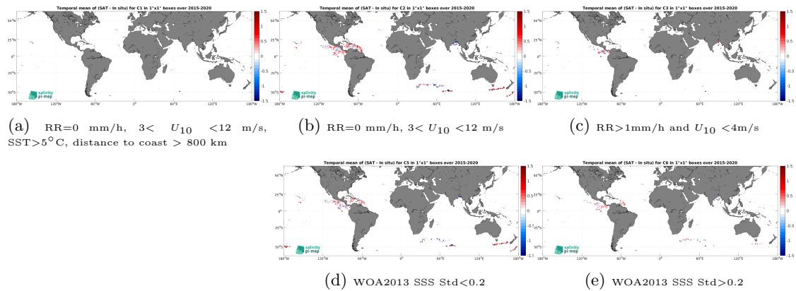
Figure 13: Temporal mean gridded over spatial boxes of size 1^\circ \times 1^\circ of \Delta SSS (SMAP SSS L2 v5.3 - 40 km (RSS) - Surface drifters) for 5 different subdatasets corresponding to:RR=0 mm/h, 3 < U_{10} < 12 m/s, SST >5^\circ\text{C} , distance to coast > 800 km (a), RR=0 mm/h, 3 < U_{10} < 12 m/s (b), RR >1 mm/h and U_{10} < 4 m/s (c), WOA2013 SSS Std <0.2 (d), WOA2013 SSS Std >0.2 (e).
