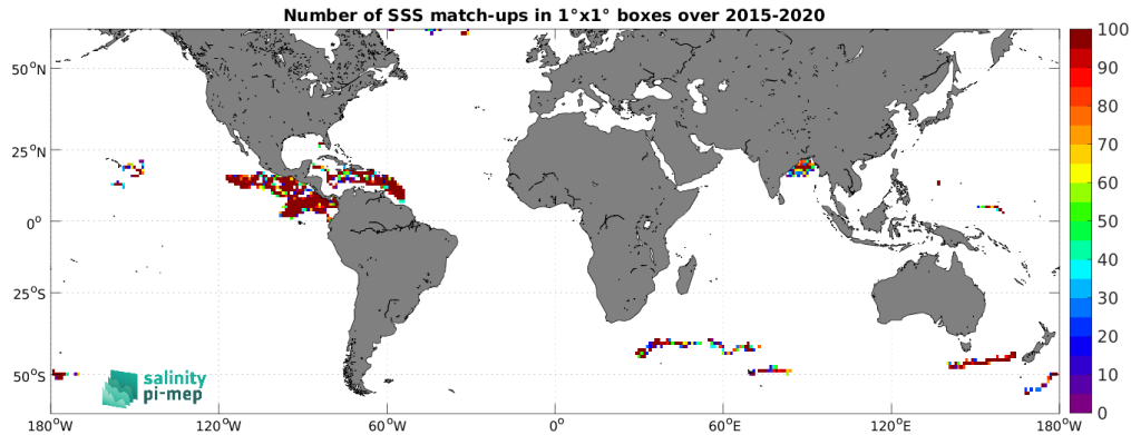
Figure 4: Number of SSS match-ups between Surface drifters SSS and the SMAP SSS L2 v5.3 - 40 km (RSS) SSS product for the SMOS coastal zone (<800km) 60N-60S Pi-MEP region over 1^\circ \times 1^\circ boxes and for the full satellite product period.
