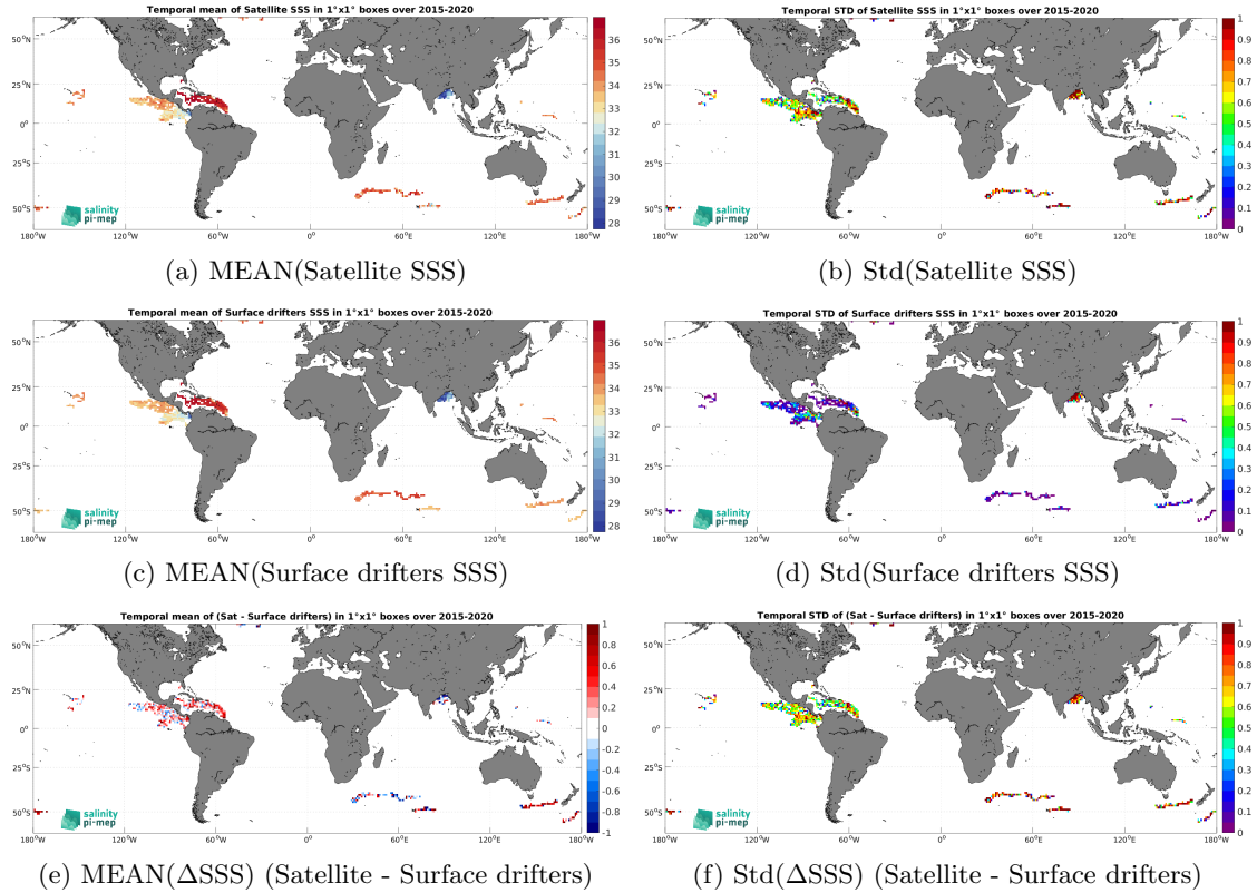
Figure 6: Temporal mean (left) and Std (right) of SSS from SMAP SSS L2 v5.3 - 40 km (RSS) (top), Surface drifters (middle), and of \Delta SSS (Satellite - Surface drifters). Only match-up pairs are used to generate these maps.
