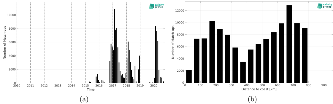
Figure 2: Number of match-ups between Surface drifters and SMAP SSS L2 v5.3 - 40 km (RSS) SSS as a function of time (a) and as function of the distance to coast (b) over the SMOS coastal zone (<800km) 60N-60S Pi-MEP region and for the full satellite product period.
