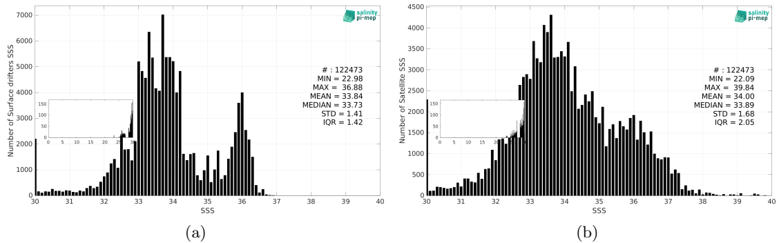
Figure 3: Histograms of SSS from Surface drifters (a) and SMAP SSS L2 v5.3 - 40 km (RSS) (b) considering all match-up pairs per bins of 0.1 over the SMOS coastal zone (<800km) 60N-60S Pi-MEP region and for the full satellite product period.
