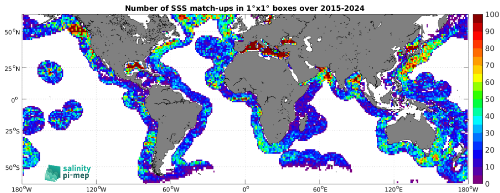
Figure 5: Number of SSS match-ups between Argo SSS and the SMAP SSS L2 v5.3 - 40 km (RSS) SSS product for the SMOS coastal zone (<800km) 60N-60S Pi-MEP region over 1^\circ \times 1^\circ boxes and for the full satellite product period.
