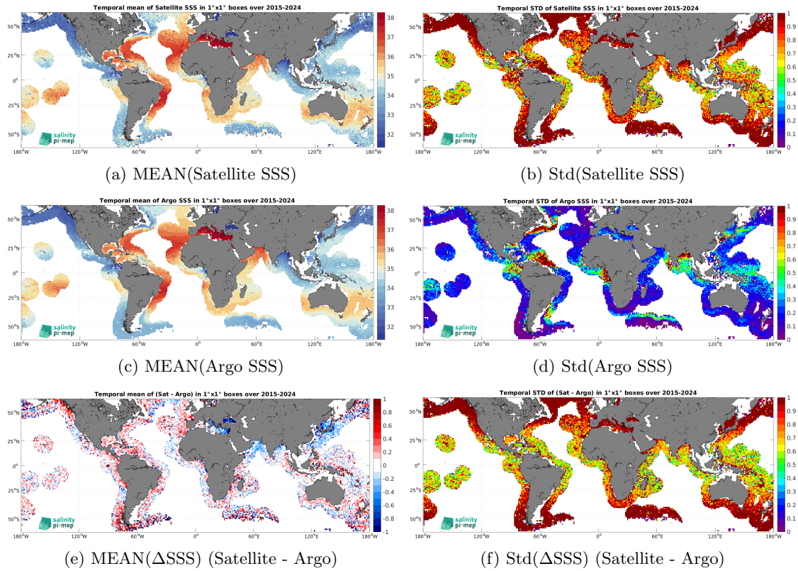
Figure 7: Temporal mean (left) and Std (right) of SSS from SMAP SSS L2 v5.3 - 40 km (RSS) (top), Argo (middle), and of \Delta SSS (Satellite - Argo). Only match-up pairs are used to generate these maps.
