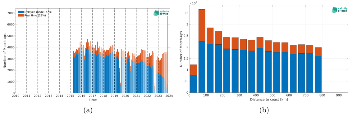
Figure 2: Number of match-ups between Argo and SMAP SSS L2 v5.3 - 40 km (RSS) SSS as a function of time (a) and as function of the distance to coast (b) over the SMOS coastal zone (<800km) 60N-60S Pi-MEP region and for the full satellite product period.
