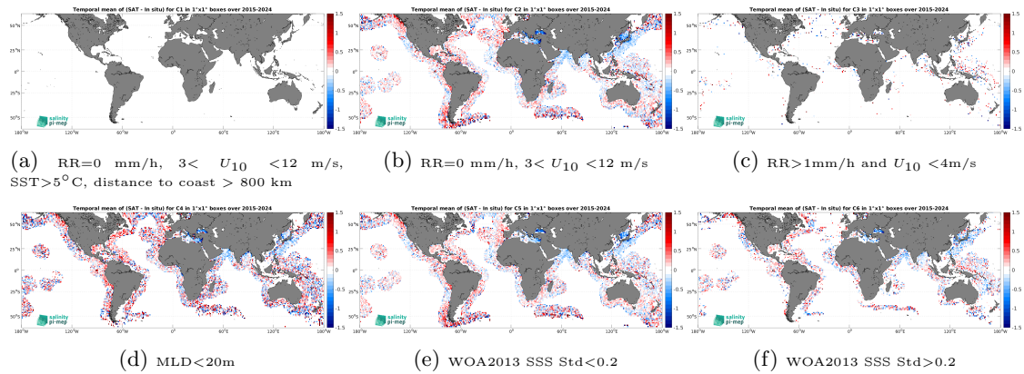
Figure 14: Temporal mean gridded over spatial boxes of size 1^\circ \times 1^\circ of \Delta SSS (SMAP SSS L2 v5.3 - 40 km (RSS) - Argo) for 6 different subdatasets corresponding to:RR=0 mm/h, 3 < U_{10} < 12 m/s, SST > 5^\circ C, distance to coast > 800 km (a), RR=0 mm/h, 3 < U_{10} < 12 m/s (b), RR > 1 mm/h and U_{10} < 4 m/s (c),MLD < 20 m (d),WOA2013 SSS Std < 0.2 (e),WOA2013 SSS Std > 0.2 (f).
