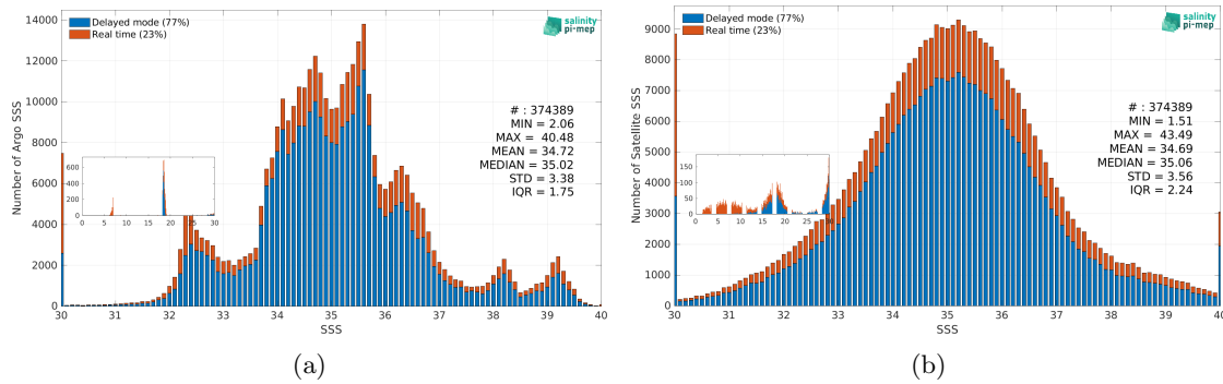
Figure 3: Histograms of SSS from Argo (a) and SMAP SSS L2 v5.3 - 40 km (RSS) (b) considering all match-up pairs per bins of 0.1 over the SMOS coastal zone (<800km) 60N-60S Pi-MEP region and for the full satellite product period.
