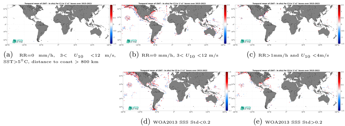
Figure 12: Temporal mean gridded over spatial boxes of size 1^\circ \times 1^\circ of \Delta SSS (SMAP SSS L2 v5 - 40 km (RSS) - TSG (SAMOS)) for 5 different subdatasets corresponding to:RR=0 mm/h, 3 < U_{10} < 12 m/s, SST >5^\circ\text{C} , distance to coast > 800 km (a), RR=0 mm/h, 3 < U_{10} < 12 m/s (b), RR >1 mm/h and U_{10} < 4 m/s (c), WOA2013 SSS Std <0.2 (d), WOA2013 SSS Std >0.2 (e).
