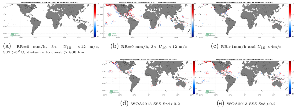
Figure 12: Temporal mean gridded over spatial boxes of size 1^\circ \times 1^\circ of \Delta\text{SSS} (SMAP SSS L2 v5 - 40 km (RSS) - TSG (SAMOS)) for 5 different subdatasets corresponding to:RR=0 mm/h, 3 < U_{10} < 12 m/s, SST >5^\circ\text{C} , distance to coast > 800 km (a), RR=0 mm/h, 3 < U_{10} < 12 m/s (b), RR >1 mm/h and U_{10} < 4 m/s (c), WOA2013 SSS Std <0.2 (d), WOA2013 SSS Std >0.2 (e).
