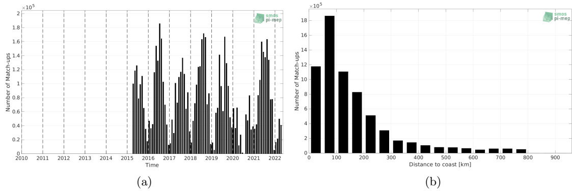
Figure 1: Number of match-ups between TSG (SAMOS) and SMAP SSS L2 v5 - 40 km (RSS) SSS as a function of time (a) and as function of the distance to coast (b) over the SMOS coastal zone (<800km) 60N-60S Pi-MEP region and for the full satellite product period.
