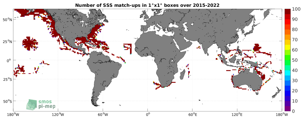
Figure 4: Number of SSS match-ups between TSG (SAMOS) SSS and the SMAP SSS L2 v5 - 40 km (RSS) SSS product for the SMOS coastal zone (<800km) 60N-60S Pi-MEP region over 1^\circ \times 1^\circ boxes and for the full satellite product period.
