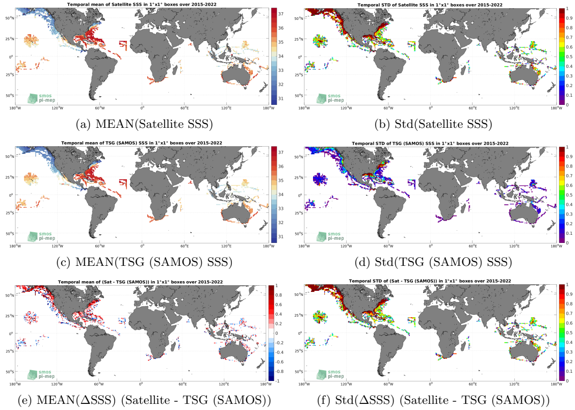
Figure 6: Temporal mean (left) and Std (right) of SSS from SMAP SSS L2 v5 - 40 km (RSS) (top), TSG (SAMOS) (middle), and of \Delta SSS (Satellite - TSG (SAMOS)). Only match-up pairs are used to generate these maps.
