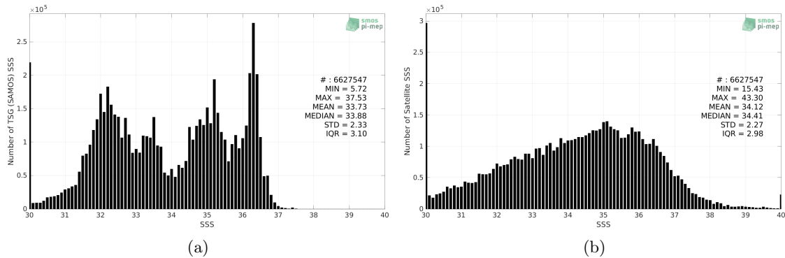
Figure 2: Histograms of SSS from TSG (SAMOS) (a) and SMAP SSS L2 v5 - 40 km (RSS) (b) considering all match-up pairs per bins of 0.1 over the SMOS coastal zone (<800km) 60N-60S Pi-MEP region and for the full satellite product period.
