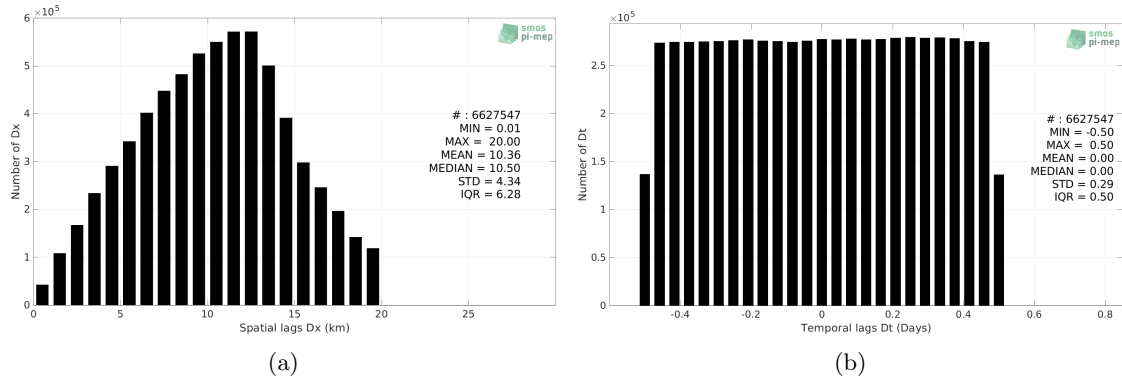
Figure 5: Histograms of the spatial (a) and temporal (b) lags between the location/time of the TSG (SAMOS) measurement and the date of the corresponding SMAP SSS L2 v5 - 40 km (RSS) SSS pixel.
