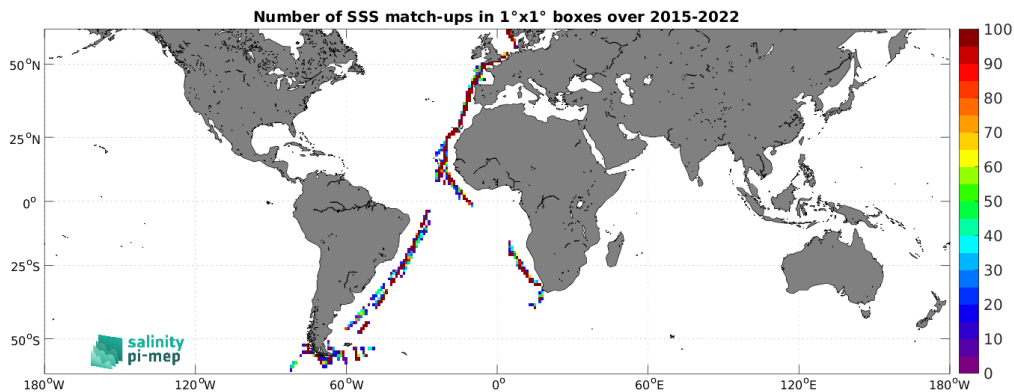
Figure 4: Number of SSS match-ups between TSG (Polarstern) SSS and the SMAP SSS L2 v5 - 40 km (RSS) SSS product for the SMOS coastal zone (<800km) 60N-60S Pi-MEP region over 1^\circ \times 1^\circ boxes and for the full satellite product period.
