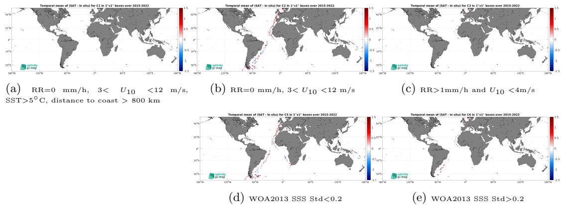
Figure 12: Temporal mean gridded over spatial boxes of size 1^\circ \times 1^\circ of \Delta\text{SSS} (SMAP SSS L2 v5 - 40 km (RSS) - TSG (Polarstern)) for 5 different subdatasets corresponding to:RR=0 mm/h, 3 < U_{10} < 12 m/s, SST >5^\circ\text{C} , distance to coast > 800 km (a), RR=0 mm/h, 3 < U_{10} < 12 m/s (b), RR >1 mm/h and U_{10} < 4 m/s (c), WOA2013 SSS Std <0.2 (d), WOA2013 SSS Std >0.2 (e).
