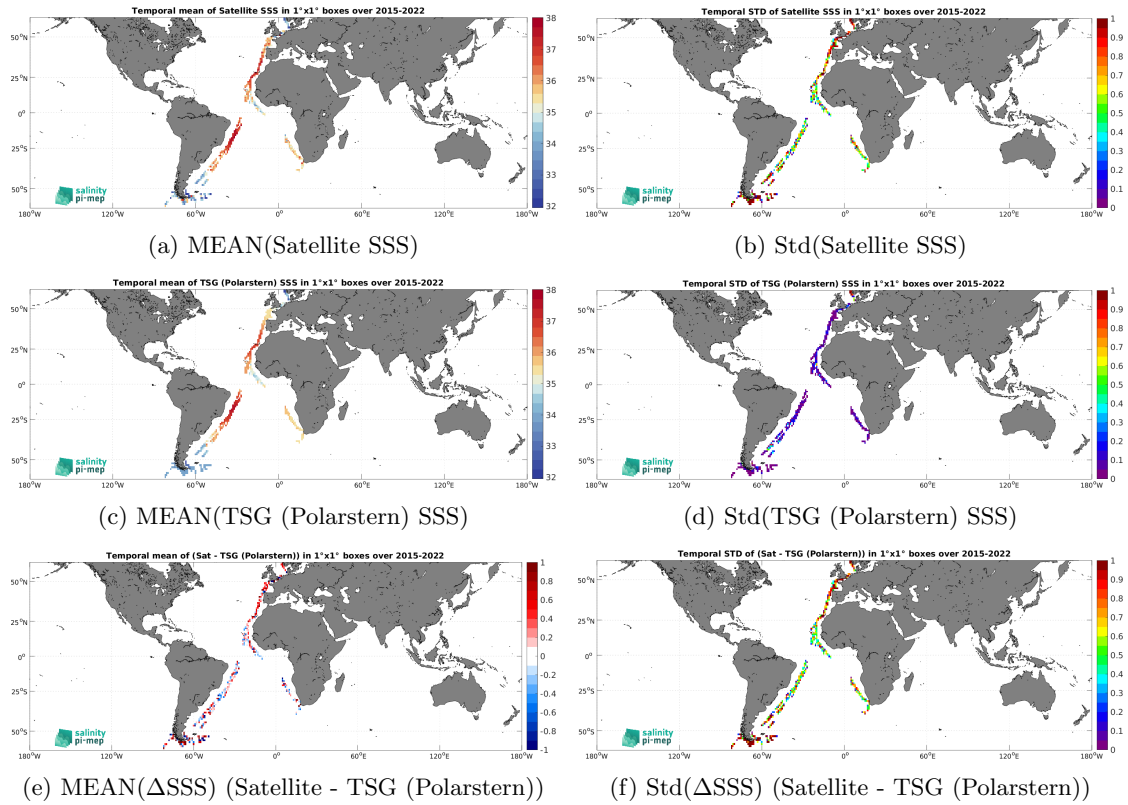
Figure 6: Temporal mean (left) and Std (right) of SSS from SMAP SSS L2 v5 - 40 km (RSS) (top), TSG (Polarstern) (middle), and of \Delta SSS (Satellite - TSG (Polarstern)). Only match-up pairs are used to generate these maps.
