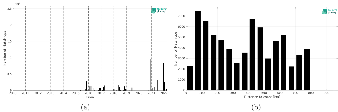
Figure 1: Number of match-ups between TSG (Polarstern) and SMAP SSS L2 v5 - 40 km (RSS) SSS as a function of time (a) and as function of the distance to coast (b) over the SMOS coastal zone (<800km) 60N-60S Pi-MEP region and for the full satellite product period.
