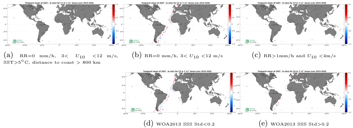
Figure 12: Temporal mean gridded over spatial boxes of size 1^\circ \times 1^\circ of \Delta SSS (SMAP SSS L2 v5 - 40 km (RSS) - TSG (Polarstern)) for 5 different subdatasets corresponding to:RR=0 mm/h, 3 < U_{10} < 12 m/s, SST >5^\circ\text{C} , distance to coast > 800 km (a), RR=0 mm/h, 3 < U_{10} < 12 m/s (b), RR >1 mm/h and U_{10} < 4 m/s (c), WOA2013 SSS Std <0.2 (d), WOA2013 SSS Std >0.2 (e).
