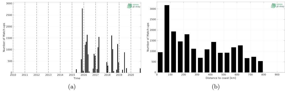
Figure 1: Number of match-ups between TSG (Polarstern) and SMAP SSS L2 v5 - 40 km (RSS) SSS as a function of time (a) and as function of the distance to coast (b) over the SMOS coastal zone (<800km) 60N-60S Pi-MEP region and for the full satellite product period.
