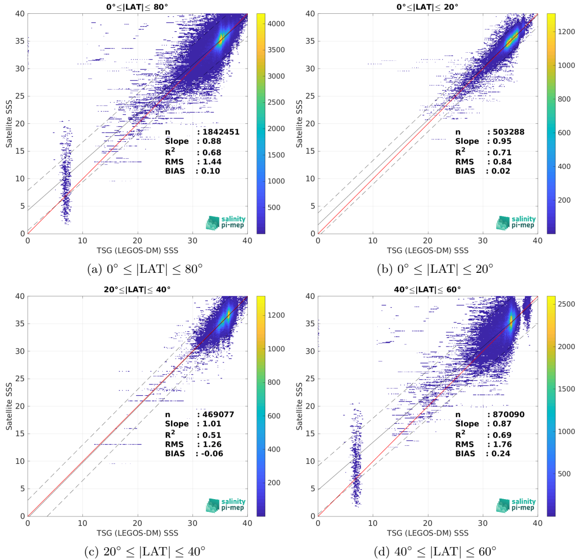
Figure 9: Contour maps of the concentration of SMAP SSS L2 v5 - 40 km (RSS) SSS (y-axis) versus TSG (LEGOS-DM) SSS (x-axis) at match-up pairs for different latitude bands. For each plot, the red line shows x=y . The black thin and dashed lines indicate a linear fit through the data cloud and the \pm 95\% confidence levels, respectively. The number match-up pairs n , the slope and R^2 coefficient of the linear fit, the root mean square (RMS) and the mean bias between satellite and in situ data are indicated for each latitude band in each plots.
