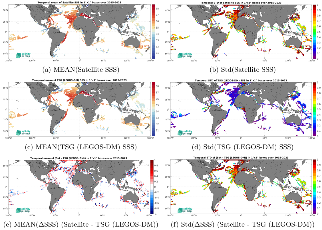
Figure 6: Temporal mean (left) and Std (right) of SSS from SMAP SSS L2 v5 - 40 km (RSS) (top), TSG (LEGOS-DM) (middle), and of \Delta SSS (Satellite - TSG (LEGOS-DM)). Only match-up pairs are used to generate these maps.
