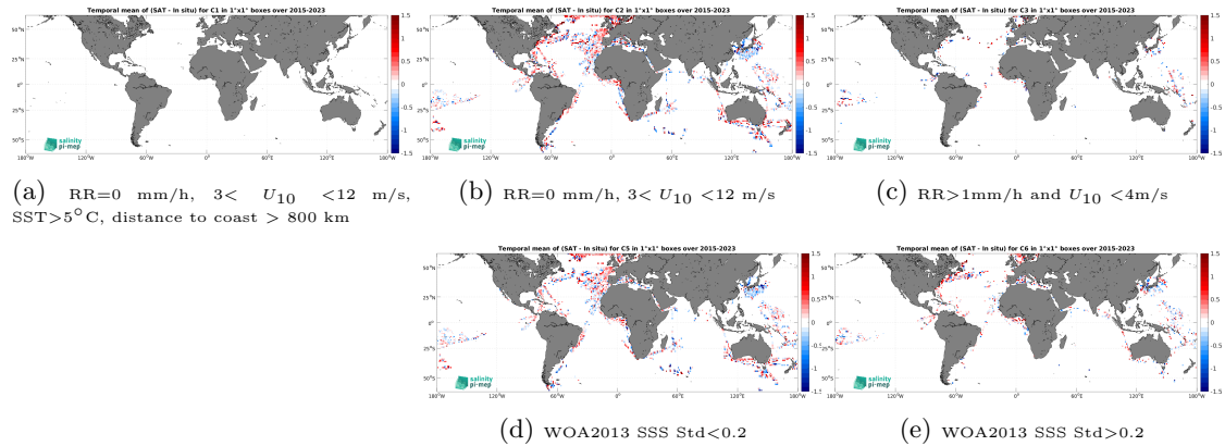
Figure 12: Temporal mean gridded over spatial boxes of size 1^\circ \times 1^\circ of \Delta\text{SSS} (SMAP SSS L2 v5 - 40 km (RSS) - TSG (LEGOS-DM)) for 5 different subdatasets corresponding to:RR=0 mm/h, 3 < U_{10} < 12 m/s, SST >5^\circ\text{C} , distance to coast > 800 km (a), RR=0 mm/h, 3 < U_{10} < 12 m/s (b), RR >1 mm/h and U_{10} < 4 m/s (c), WOA2013 SSS Std <0.2 (d), WOA2013 SSS Std >0.2 (e).
