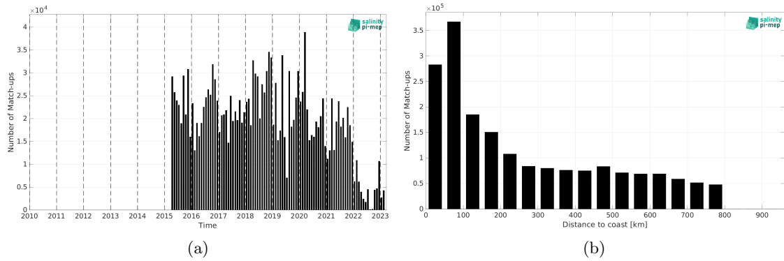
Figure 1: Number of match-ups between TSG (LEGOS-DM) and SMAP SSS L2 v5 - 40 km (RSS) SSS as a function of time (a) and as function of the distance to coast (b) over the SMOS coastal zone (<800km) 60N-60S Pi-MEP region and for the full satellite product period.
