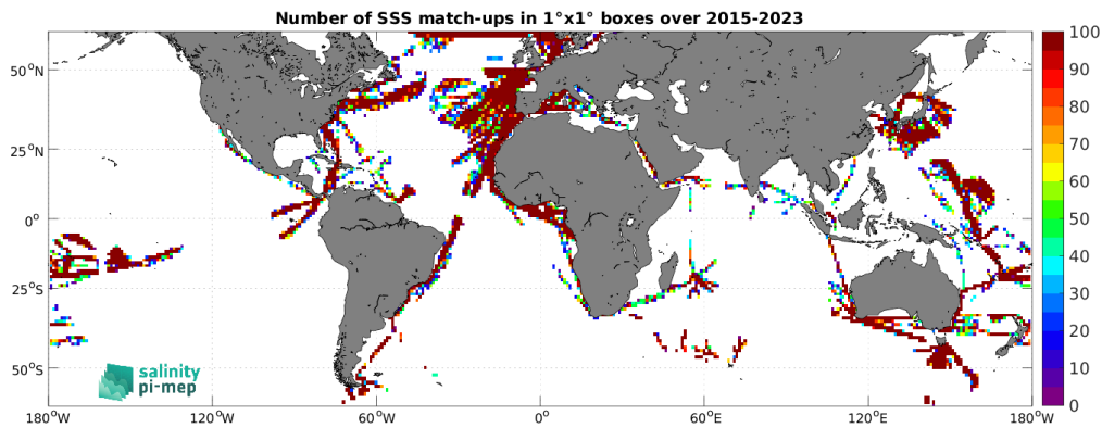
Figure 4: Number of SSS match-ups between TSG (LEGOS-DM) SSS and the SMAP SSS L2 v5 - 40 km (RSS) SSS product for the SMOS coastal zone (<800km) 60N-60S Pi-MEP region over 1^\circ \times 1^\circ boxes and for the full satellite product period.
