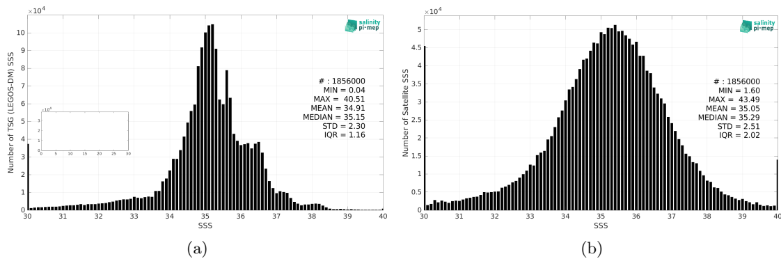
Figure 2: Histograms of SSS from TSG (LEGOS-DM) (a) and SMAP SSS L2 v5 - 40 km (RSS) (b) considering all match-up pairs per bins of 0.1 over the SMOS coastal zone (<800km) 60N-60S Pi-MEP region and for the full satellite product period.
