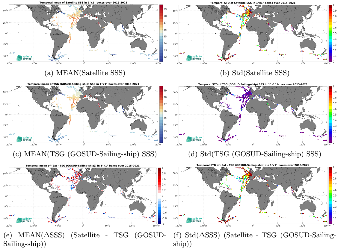
Figure 6: Temporal mean (left) and Std (right) of SSS from SMAP SSS L2 v5 - 40 km (RSS) (top), TSG (GOSUD-Sailing-ship) (middle), and of \Delta SSS (Satellite - TSG (GOSUD-Sailing-ship)). Only match-up pairs are used to generate these maps.
