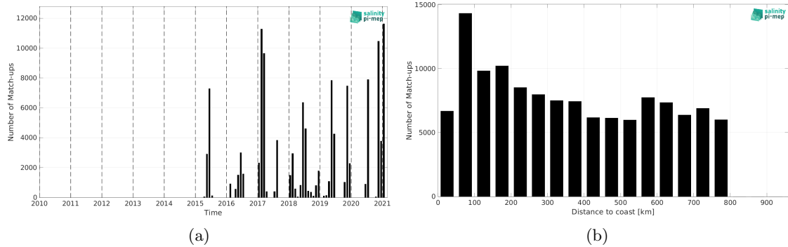
Figure 1: Number of match-ups between TSG (GOSUD-Sailing-ship) and SMAP SSS L2 v5 - 40 km (RSS) SSS as a function of time (a) and as function of the distance to coast (b) over the SMOS coastal zone (<800km) 60N-60S Pi-MEP region and for the full satellite product period.
