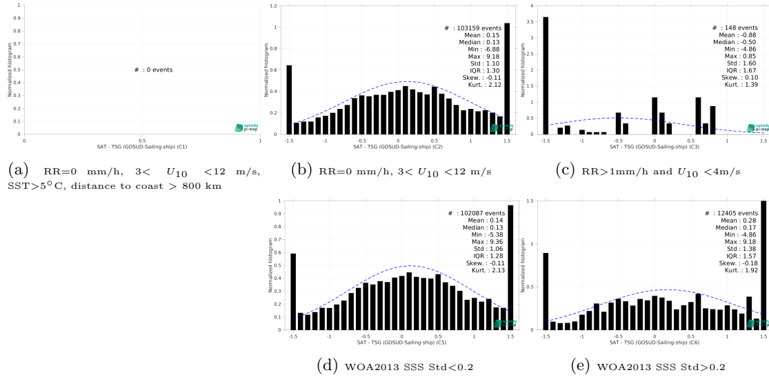
Figure 13: Normalized histogram of \Delta SSS (SMAP SSS L2 v5 - 40 km (RSS) - TSG (GOSUD-Sailing-ship)) for 5 different subdatasets corresponding to: RR=0 mm/h, 3 < U_{10} < 12 m/s, SST>5°C, distance to coast > 800 km (a), RR=0 mm/h, 3 < U_{10} < 12 m/s (b), RR>1mm/h and U_{10} < 4 m/s (c), WOA2013 SSS Std<0.2 (d), WOA2013 SSS Std>0.2 (e).
