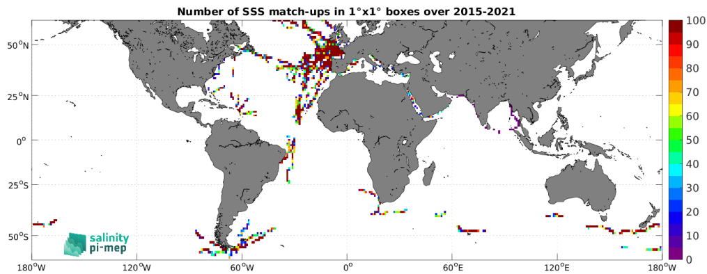
Figure 4: Number of SSS match-ups between TSG (GOSUD-Sailing-ship) SSS and the SMAP SSS L2 v5 - 40 km (RSS) SSS product for the SMOS coastal zone (<800km) 60N-60S Pi-MEP region over 1^\circ \times 1^\circ boxes and for the full satellite product period.
