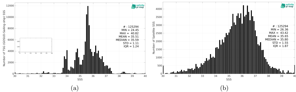
Figure 2: Histograms of SSS from TSG (GOSUD-Sailing-ship) (a) and SMAP SSS L2 v5 - 40 km (RSS) (b) considering all match-up pairs per bins of 0.1 over the SMOS coastal zone (<800km) 60N-60S Pi-MEP region and for the full satellite product period.
