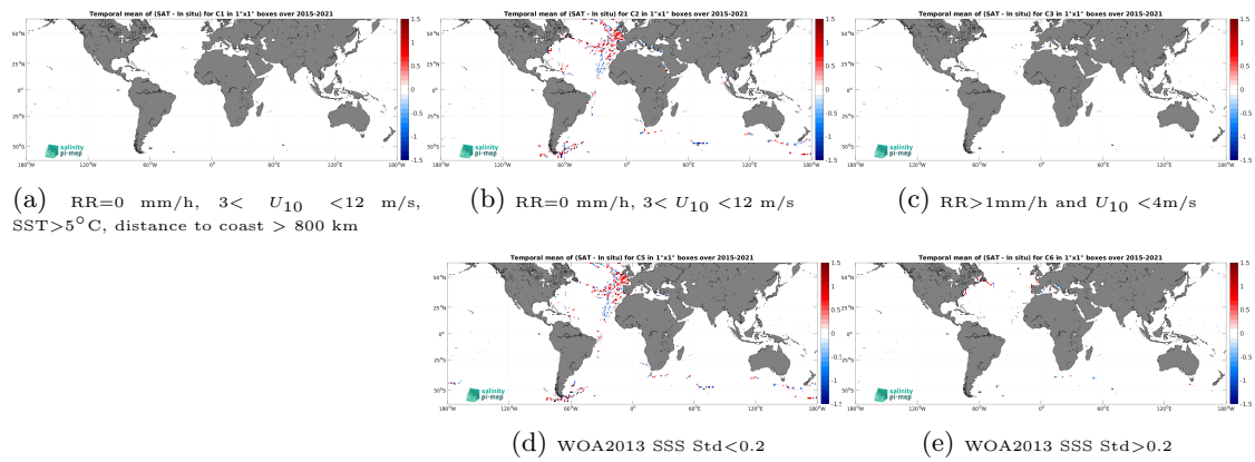
Figure 12: Temporal mean gridded over spatial boxes of size 1^\circ \times 1^\circ of \Delta\text{SSS} (SMAP SSS L2 v5 - 40 km (RSS) - TSG (GOSUD-Sailing-ship)) for 5 different subdatasets corresponding to: RR=0 mm/h, 3 < U_{10} < 12 m/s, SST > 5°C, distance to coast > 800 km (a), RR=0 mm/h, 3 < U_{10} < 12 m/s (b), RR > 1mm/h and U_{10} < 4 m/s (c), WOA2013 SSS Std < 0.2 (d), WOA2013 SSS Std > 0.2 (e).
