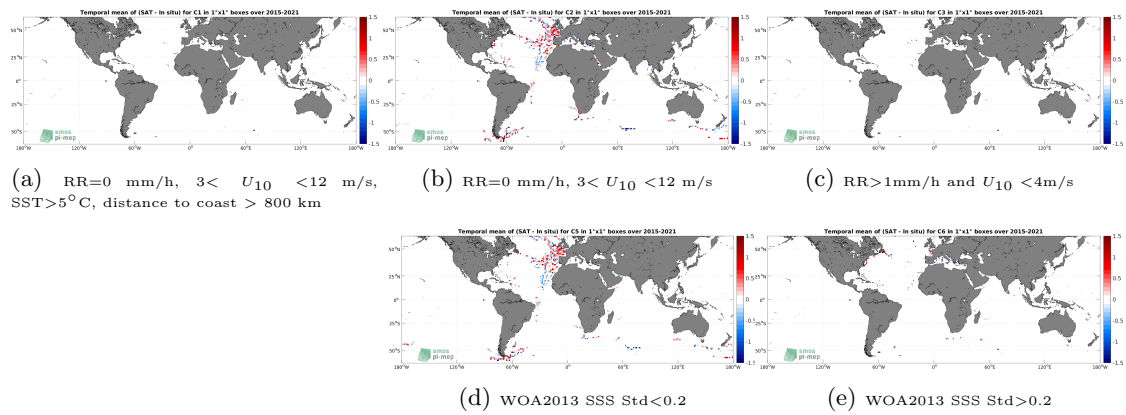
Figure 12: Temporal mean gridded over spatial boxes of size 1^\circ \times 1^\circ of \Delta SSS (SMAP SSS L2 v5 - 40 km (RSS) - TSG (GOSUD-Sailing-ship)) for 5 different subdatasets corresponding to:RR=0 mm/h, 3 < U_{10} < 12 m/s, SST >5^\circ\text{C} , distance to coast > 800 km (a), RR=0 mm/h, 3 < U_{10} < 12 m/s (b), RR >1 mm/h and U_{10} < 4 m/s (c), WOA2013 SSS Std <0.2 (d), WOA2013 SSS Std >0.2 (e).
