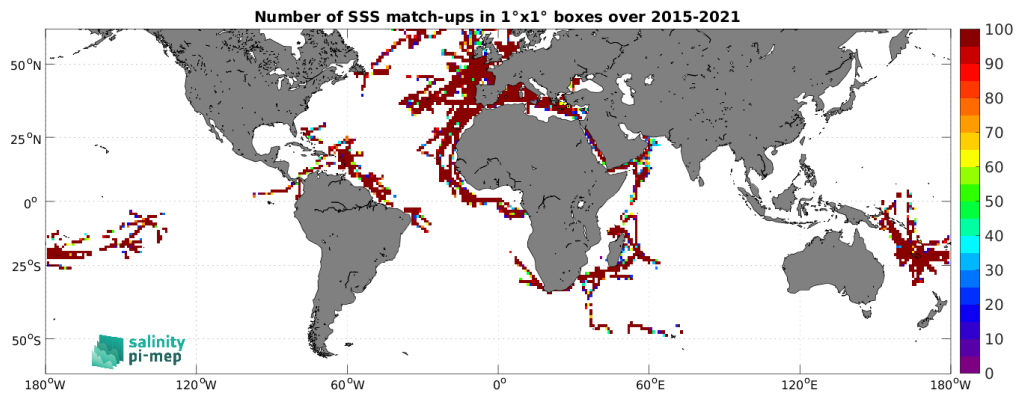
Figure 4: Number of SSS match-ups between TSG (GOSUD-Research-vessel) SSS and the SMAP SSS L2 v5 - 40 km (RSS) SSS product for the SMOS coastal zone ( <800\text{km} ) 60N-60S Pi-MEP region over 1^\circ \times 1^\circ boxes and for the full satellite product period.
