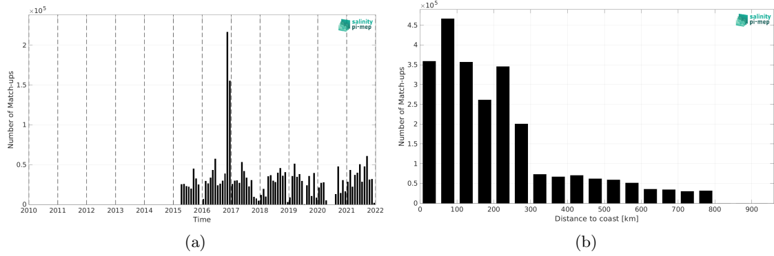
Figure 1: Number of match-ups between TSG (GOSUD-Research-vessel) and SMAP SSS L2 v5 - 40 km (RSS) SSS as a function of time (a) and as function of the distance to coast (b) over the SMOS coastal zone (<800km) 60N-60S Pi-MEP region and for the full satellite product period.
