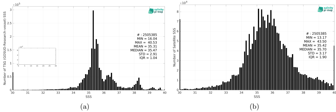
Figure 2: Histograms of SSS from TSG (GOSUD-Research-vessel) (a) and SMAP SSS L2 v5 - 40 km (RSS) (b) considering all match-up pairs per bins of 0.1 over the SMOS coastal zone (<800km) 60N-60S Pi-MEP region and for the full satellite product period.
