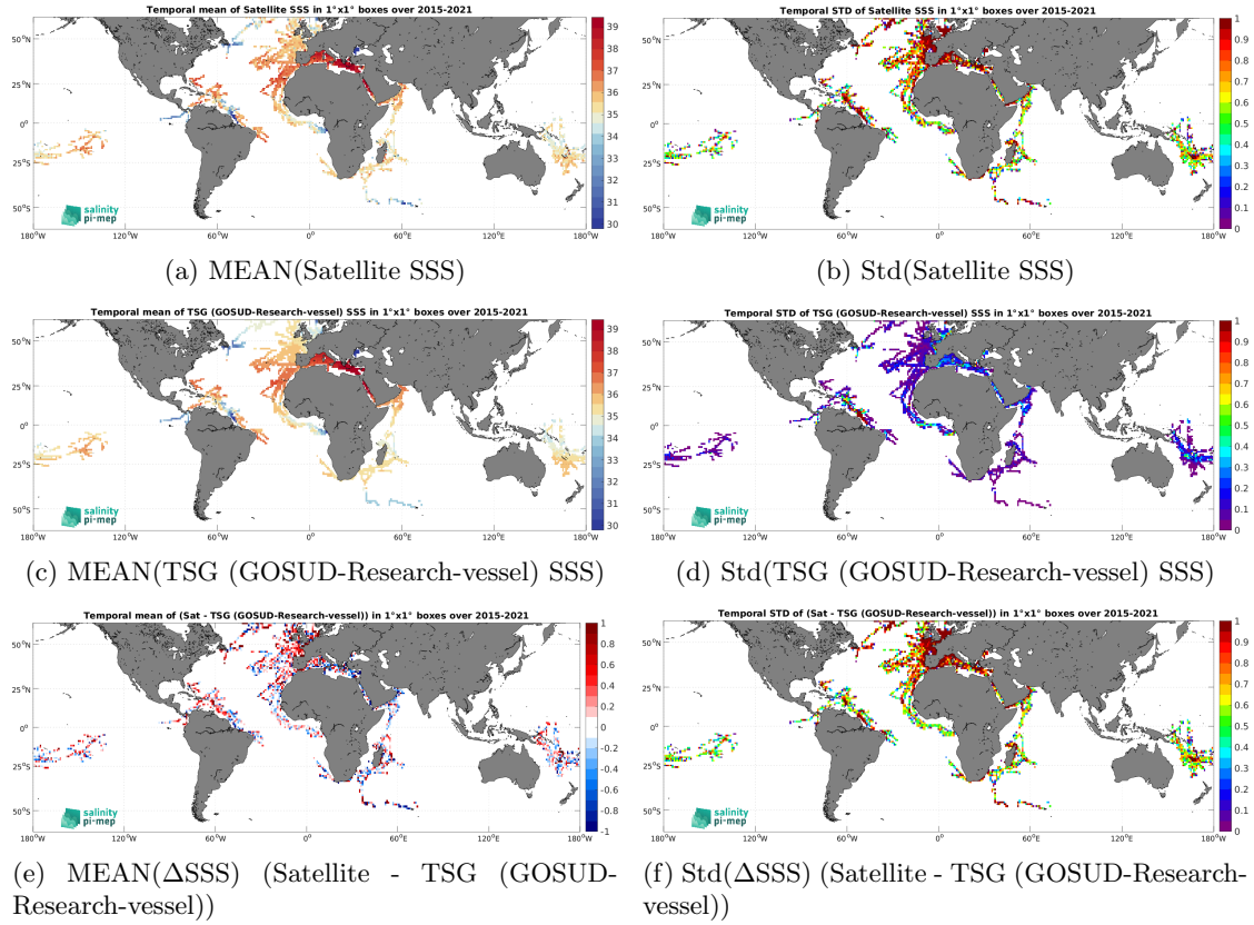
Figure 6: Temporal mean (left) and Std (right) of SSS from SMAP SSS L2 v5 - 40 km (RSS) (top), TSG (GOSUD-Research-vessel) (middle), and of \Delta SSS (Satellite - TSG (GOSUD-Research-vessel)). Only match-up pairs are used to generate these maps.
