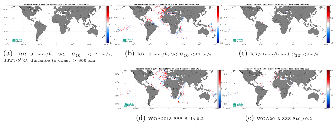
Figure 12: Temporal mean gridded over spatial boxes of size 1^\circ \times 1^\circ of \Delta\text{SSS} (SMAP SSS L2 v5 - 40 km (RSS) - TSG (GOSUD-Research-vessel)) for 5 different subdatasets corresponding to: RR=0 mm/h, 3 < U_{10} < 12 m/s, SST > 5°C, distance to coast > 800 km (a), RR=0 mm/h, 3 < U_{10} < 12 m/s (b), RR > 1mm/h and U_{10} < 4 m/s (c), WOA2013 SSS Std < 0.2 (d), WOA2013 SSS Std > 0.2 (e).
