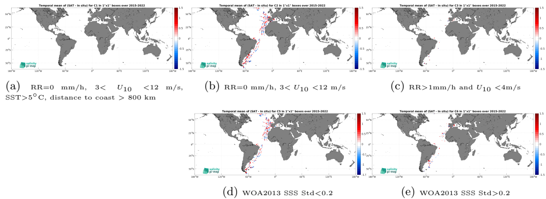
Figure 12: Temporal mean gridded over spatial boxes of size 1^\circ \times 1^\circ of \Delta\text{SSS} (SMAP SSS L2 v5 - 40 km (RSS) - TSG (CSIC-UTM)) for 5 different subdatasets corresponding to:RR=0 mm/h, 3 < U_{10} < 12 m/s, SST >5^\circ\text{C} , distance to coast > 800 km (a), RR=0 mm/h, 3 < U_{10} < 12 m/s (b), RR >1 mm/h and U_{10} < 4 m/s (c), WOA2013 SSS Std <0.2 (d), WOA2013 SSS Std >0.2 (e).
