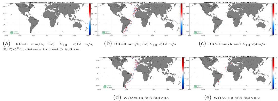
Figure 12: Temporal mean gridded over spatial boxes of size 1^\circ \times 1^\circ of \Delta SSS (SMAP SSS L2 v5 - 40 km (RSS) - TSG (CSIC-UTM)) for 5 different subdatasets corresponding to:RR=0 mm/h, 3 < U_{10} < 12 m/s, SST >5^\circ\text{C} , distance to coast > 800 km (a), RR=0 mm/h, 3 < U_{10} < 12 m/s (b), RR >1 mm/h and U_{10} < 4 m/s (c), WOA2013 SSS Std <0.2 (d), WOA2013 SSS Std >0.2 (e).
