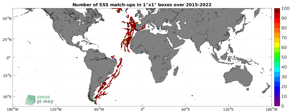
Figure 4: Number of SSS match-ups between TSG (CSIC-UTM) SSS and the SMAP SSS L2 v5 - 40 km (RSS) SSS product for the SMOS coastal zone (<800km) 60N-60S Pi-MEP region over 1^\circ \times 1^\circ boxes and for the full satellite product period.
