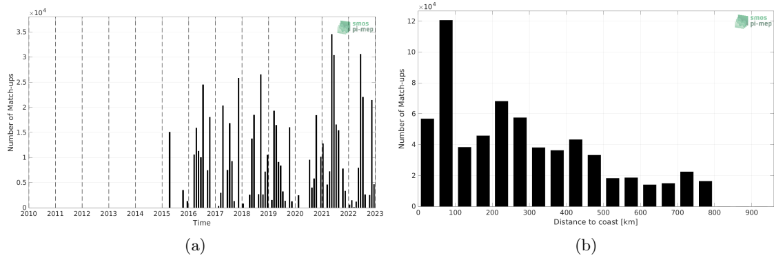
Figure 1: Number of match-ups between TSG (CSIC-UTM) and SMAP SSS L2 v5 - 40 km (RSS) SSS as a function of time (a) and as function of the distance to coast (b) over the SMOS coastal zone (<800km) 60N-60S Pi-MEP region and for the full satellite product period.
