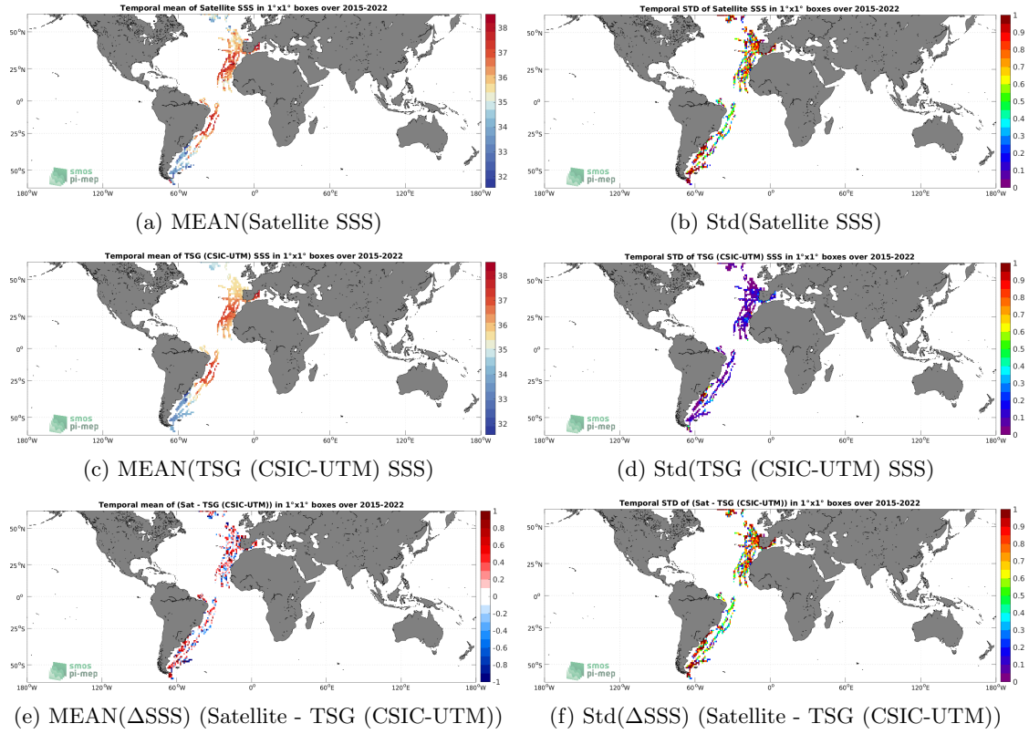
Figure 6: Temporal mean (left) and Std (right) of SSS from SMAP SSS L2 v5 - 40 km (RSS) (top), TSG (CSIC-UTM) (middle), and of \Delta SSS (Satellite - TSG (CSIC-UTM)). Only match-up pairs are used to generate these maps.
