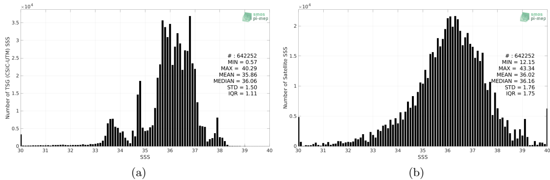
Figure 2: Histograms of SSS from TSG (CSIC-UTM) (a) and SMAP SSS L2 v5 - 40 km (RSS) (b) considering all match-up pairs per bins of 0.1 over the SMOS coastal zone (<800km) 60N-60S Pi-MEP region and for the full satellite product period.
