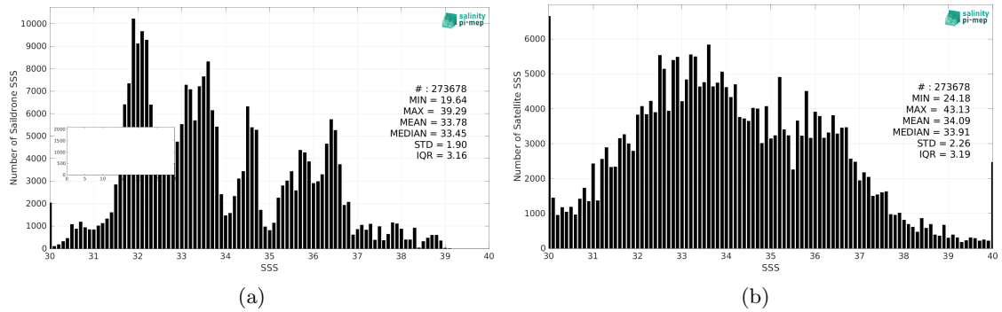
Figure 2: Histograms of SSS from Saildrone (a) and SMAP SSS L2 v5 - 40 km (RSS) (b) considering all match-up pairs per bins of 0.1 over the SMOS coastal zone (<800km) 60N-60S Pi-MEP region and for the full satellite product period.
