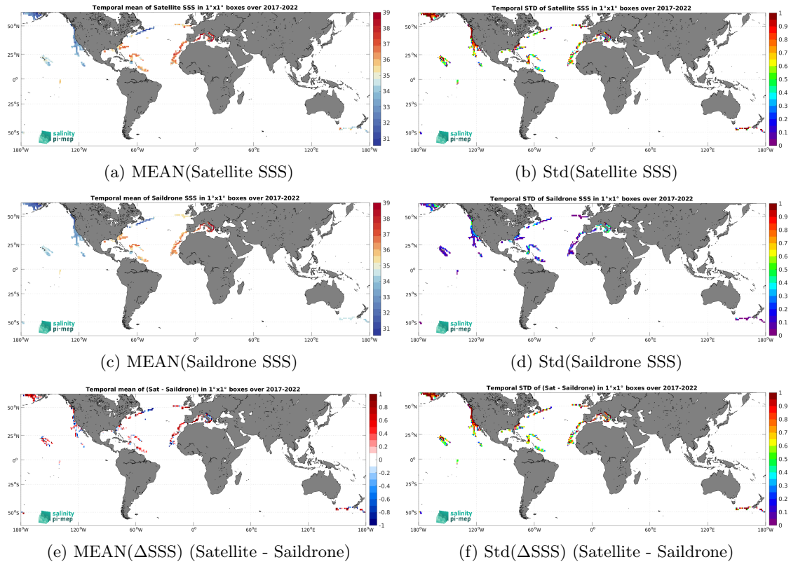
Figure 6: Temporal mean (left) and Std (right) of SSS from SMAP SSS L2 v5 - 40 km (RSS) (top), Saildrone (middle), and of \Delta SSS (Satellite - Saildrone). Only match-up pairs are used to generate these maps.
