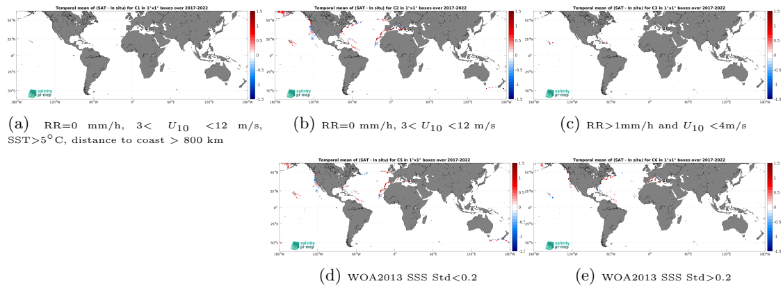
Figure 12: Temporal mean gridded over spatial boxes of size 1^\circ \times 1^\circ of \Delta SSS (SMAP SSS L2 v5 - 40 km (RSS) - Saildrone) for 5 different subdatasets corresponding to:RR=0 mm/h, 3 < U_{10} < 12 m/s, SST >5^\circ\text{C} , distance to coast > 800 km (a), RR=0 mm/h, 3 < U_{10} < 12 m/s (b), RR >1 mm/h and U_{10} < 4 m/s (c), WOA2013 SSS Std <0.2 (d), WOA2013 SSS Std >0.2 (e).
