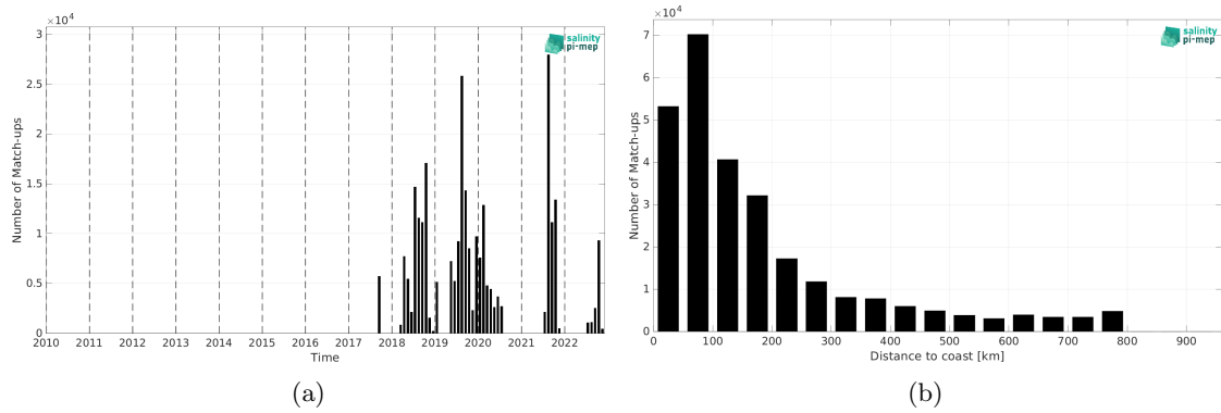
Figure 1: Number of match-ups between Saildrone and SMAP SSS L2 v5 - 40 km (RSS) SSS as a function of time (a) and as function of the distance to coast (b) over the SMOS coastal zone (<800km) 60N-60S Pi-MEP region and for the full satellite product period.
