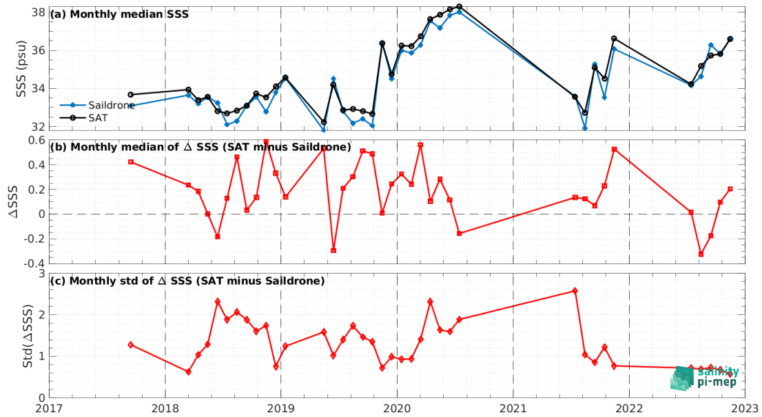
Figure 7: Time series of the monthly median SSS (top), median of \Delta SSS (Satellite - SAILDRONE) and Std of \Delta SSS (Satellite - SAILDRONE) over the SMOS coastal zone ( <800\text{km} ) 60\text{N} - 60\text{S} Pi-MEP region considering all match-ups collected by the Pi-MEP.
