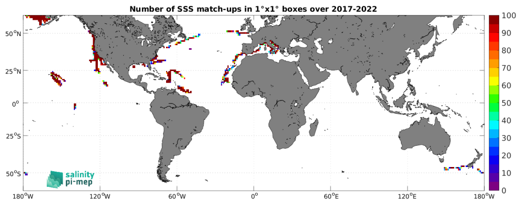
Figure 4: Number of SSS match-ups between Saildrone SSS and the SMAP SSS L2 v5 - 40 km (RSS) SSS product for the SMOS coastal zone (<800km) 60N-60S Pi-MEP region over 1^\circ \times 1^\circ boxes and for the full satellite product period.
