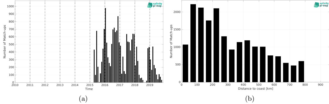
Figure 1: Number of match-ups between Marine mammals and SMAP SSS L2 v5 - 40 km (RSS) SSS as a function of time (a) and as function of the distance to coast (b) over the SMOS coastal zone (<800km) 60N-60S Pi-MEP region and for the full satellite product period.
