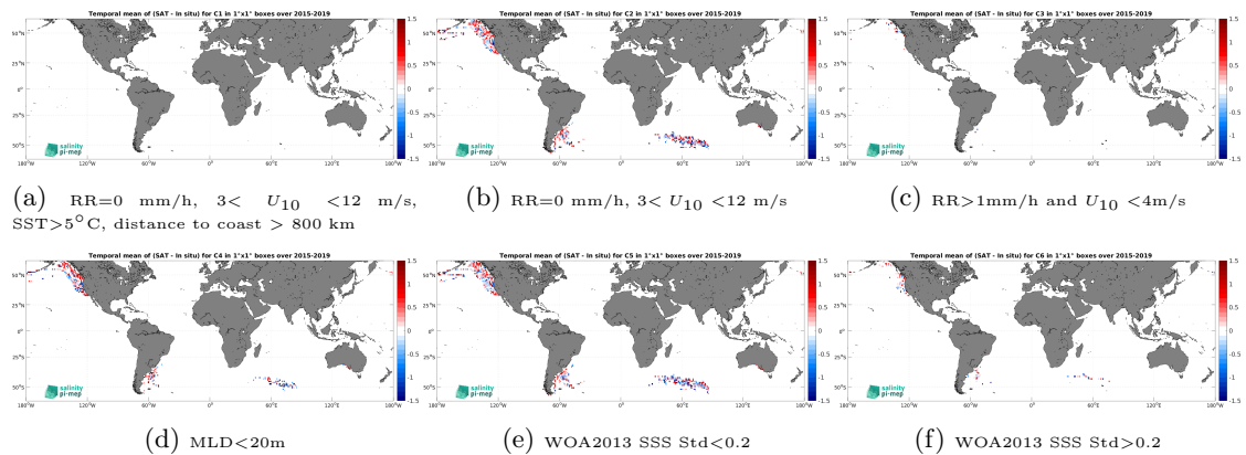
Figure 12: Temporal mean gridded over spatial boxes of size 1^\circ \times 1^\circ of \Delta SSS (SMAP SSS L2 v5 - 40 km (RSS) - Marine mammals) for 6 different subdatasets corresponding to:RR=0 mm/h, 3 < U_{10} < 12 m/s, SST >5^\circ C, distance to coast > 800 km (a), RR=0 mm/h, 3 < U_{10} < 12 m/s (b), RR >1 mm/h and U_{10} < 4 m/s (c),MLD <20 m (d),WOA2013 SSS Std <0.2 (e),WOA2013 SSS Std >0.2 (f).
