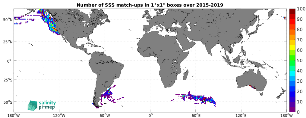
Figure 4: Number of SSS match-ups between Marine mammals SSS and the SMAP SSS L2 v5 - 40 km (RSS) SSS product for the SMOS coastal zone (<800km) 60N-60S Pi-MEP region over 1^\circ \times 1^\circ boxes and for the full satellite product period.
