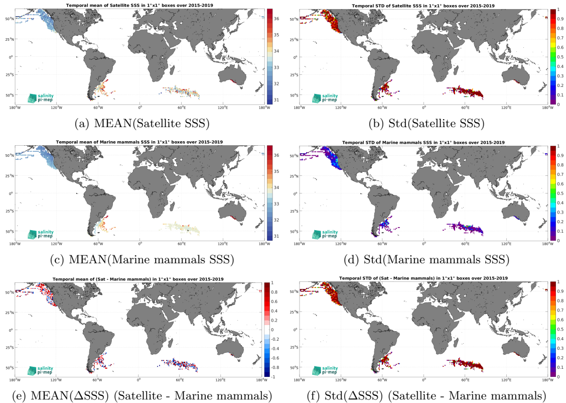
Figure 6: Temporal mean (left) and Std (right) of SSS from SMAP SSS L2 v5 - 40 km (RSS) (top), Marine mammals (middle), and of \Delta SSS (Satellite - Marine mammals). Only match-up pairs are used to generate these maps.
