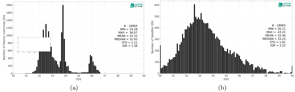
Figure 2: Histograms of SSS from Marine mammals (a) and SMAP SSS L2 v5 - 40 km (RSS) (b) considering all match-up pairs per bins of 0.1 over the SMOS coastal zone (<800km) 60N-60S Pi-MEP region and for the full satellite product period.
