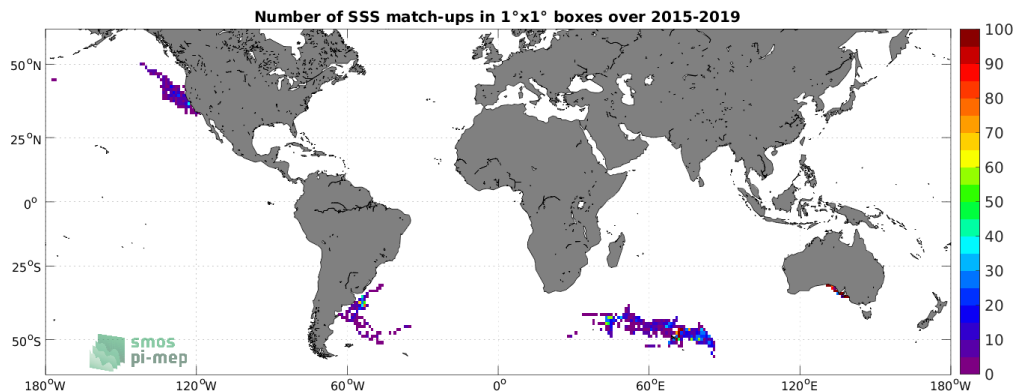
Figure 4: Number of SSS match-ups between Marine mammals SSS and the SMAP SSS L2 v5 - 40 km (RSS) SSS product for the SMOS coastal zone (<800km) 60N-60S Pi-MEP region over 1°x1° boxes and for the full satellite product period.
