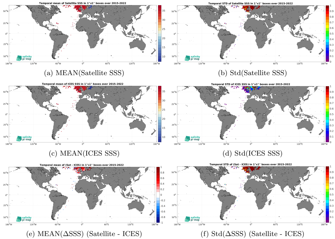
Figure 6: Temporal mean (left) and Std (right) of SSS from SMAP SSS L2 v5 - 40 km (RSS) (top), ICES (middle), and of \Delta SSS (Satellite - ICES). Only match-up pairs are used to generate these maps.
