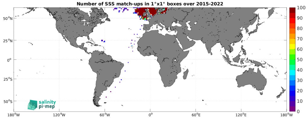
Figure 4: Number of SSS match-ups between ICES SSS and the SMAP SSS L2 v5 - 40 km (RSS) SSS product for the SMOS coastal zone (<800km) 60N-60S Pi-MEP region over 1^\circ \times 1^\circ boxes and for the full satellite product period.
