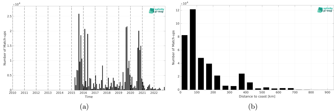
Figure 1: Number of match-ups between ICES and SMAP SSS L2 v5 - 40 km (RSS) SSS as a function of time (a) and as function of the distance to coast (b) over the SMOS coastal zone (<800km) 60N-60S Pi-MEP region and for the full satellite product period.
