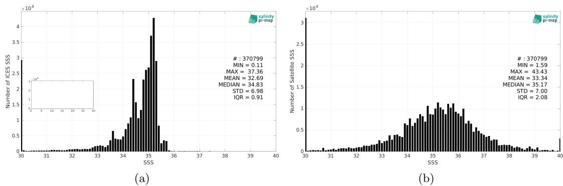
Figure 2: Histograms of SSS from ICES (a) and SMAP SSS L2 v5 - 40 km (RSS) (b) considering all match-up pairs per bins of 0.1 over the SMOS coastal zone (<800km) 60N-60S Pi-MEP region and for the full satellite product period.
