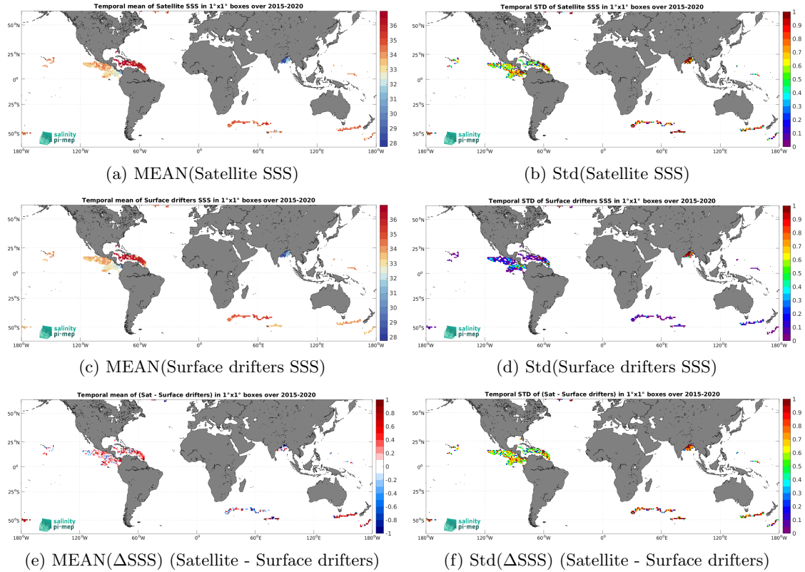
Figure 5: Temporal mean (left) and Std (right) of SSS from SMAP SSS L2 v5 - 40 km (RSS) (top), Surface drifters (middle), and of \Delta SSS (Satellite - Surface drifters). Only match-up pairs are used to generate these maps.
