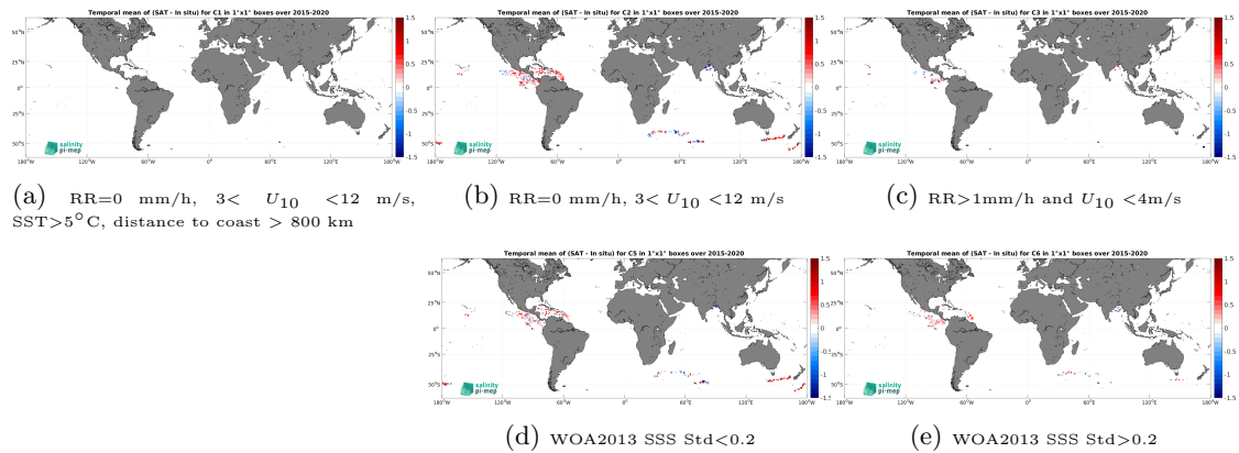
Figure 11: Temporal mean gridded over spatial boxes of size 1^\circ \times 1^\circ of \Delta SSS (SMAP SSS L2 v5 - 40 km (RSS) - Surface drifters) for 5 different subdatasets corresponding to:RR=0 mm/h, 3 < U_{10} < 12 m/s, SST >5^\circ C, distance to coast > 800 km (a), RR=0 mm/h, 3 < U_{10} < 12 m/s (b), RR >1 mm/h and U_{10} < 4 m/s (c), WOA2013 SSS Std <0.2 (d), WOA2013 SSS Std >0.2 (e).
