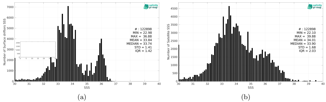
Figure 2: Histograms of SSS from Surface drifters (a) and SMAP SSS L2 v5 - 40 km (RSS) (b) considering all match-up pairs per bins of 0.1 over the SMOS coastal zone (<800km) 60N-60S Pi-MEP region and for the full satellite product period.
