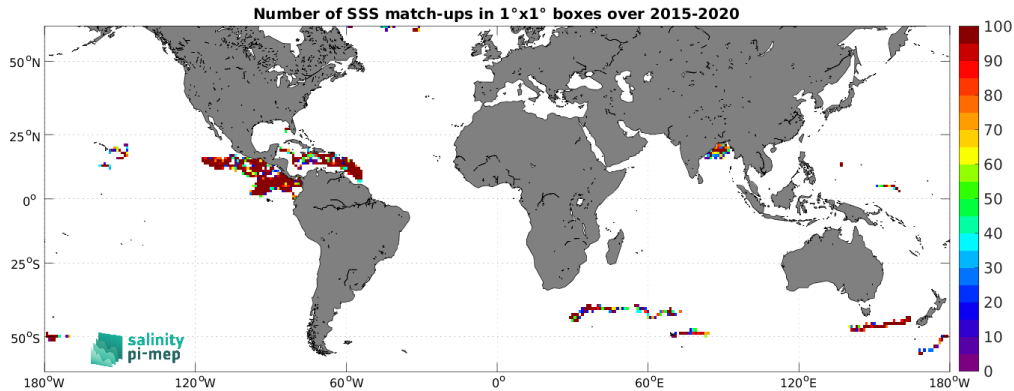
Figure 3: Number of SSS match-ups between Surface drifters SSS and the SMAP SSS L2 v5 - 40 km (RSS) SSS product for the SMOS coastal zone (<800km) 60N-60S Pi-MEP region over 1^\circ \times 1^\circ boxes and for the full satellite product period.
