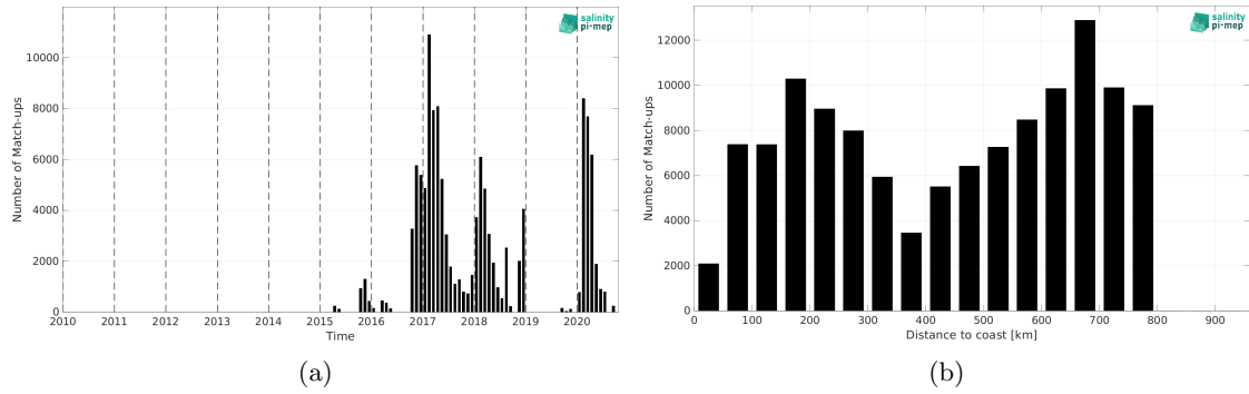
Figure 1: Number of match-ups between Surface drifters and SMAP SSS L2 v5 - 40 km (RSS) SSS as a function of time (a) and as function of the distance to coast (b) over the SMOS coastal zone (<800km) 60N-60S Pi-MEP region and for the full satellite product period.
