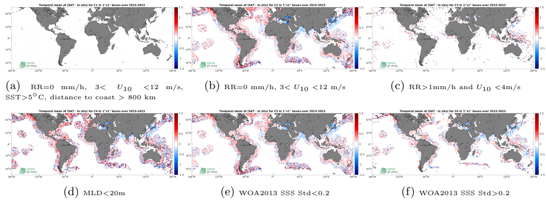
Figure 12: Temporal mean gridded over spatial boxes of size 1^\circ \times 1^\circ of \Delta SSS (SMAP SSS L2 v5 - 40 km (RSS) - Argo) for 6 different subdatasets corresponding to:RR=0 mm/h, 3 < U_{10} < 12 m/s, SST > 5^\circ\text{C} , distance to coast > 800 km (a), RR=0 mm/h, 3 < U_{10} < 12 m/s (b), RR > 1 mm/h and U_{10} < 4 m/s (c),MLD < 20 m (d),WOA2013 SSS Std < 0.2 (e),WOA2013 SSS Std > 0.2 (f).
