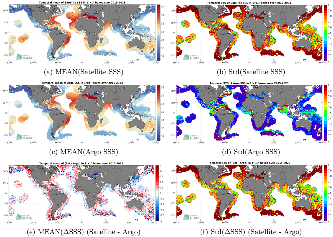
Figure 6: Temporal mean (left) and Std (right) of SSS from SMAP SSS L2 v5 - 40 km (RSS) (top), Argo (middle), and of \Delta SSS (Satellite - Argo). Only match-up pairs are used to generate these maps.
