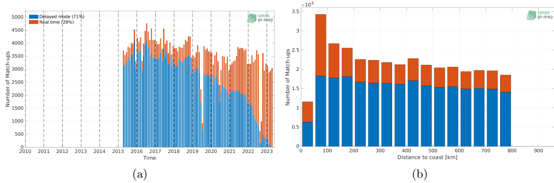
Figure 1: Number of match-ups between Argo and SMAP SSS L2 v5 - 40 km (RSS) SSS as a function of time (a) and as function of the distance to coast (b) over the SMOS coastal zone (<800km) 60N-60S Pi-MEP region and for the full satellite product period.
