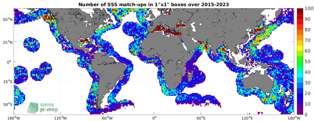
Figure 4: Number of SSS match-ups between Argo SSS and the SMAP SSS L2 v5 - 40 km (RSS) SSS product for the SMOS coastal zone (<800km) 60N-60S Pi-MEP region over 1^\circ \times 1^\circ boxes and for the full satellite product period.
