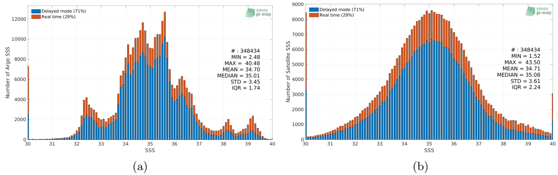
Figure 2: Histograms of SSS from Argo (a) and SMAP SSS L2 v5 - 40 km (RSS) (b) considering all match-up pairs per bins of 0.1 over the SMOS coastal zone (<800km) 60N-60S Pi-MEP region and for the full satellite product period.
