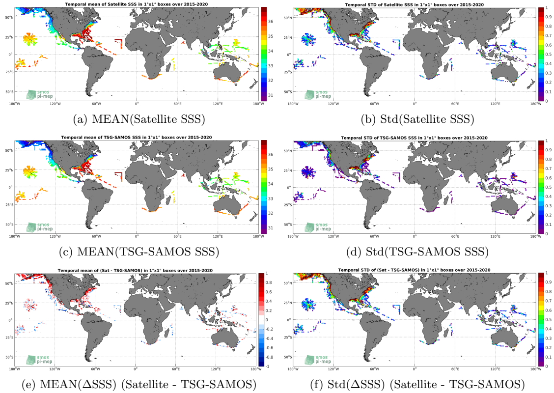
Figure 6: Temporal mean (left) and Std (right) of SSS from SMAP-L2-RSS-V4 (top), TSG-SAMOS (middle), and of \Delta SSS (Satellite - TSG-SAMOS). Only match-up pairs are used to generate these maps.
