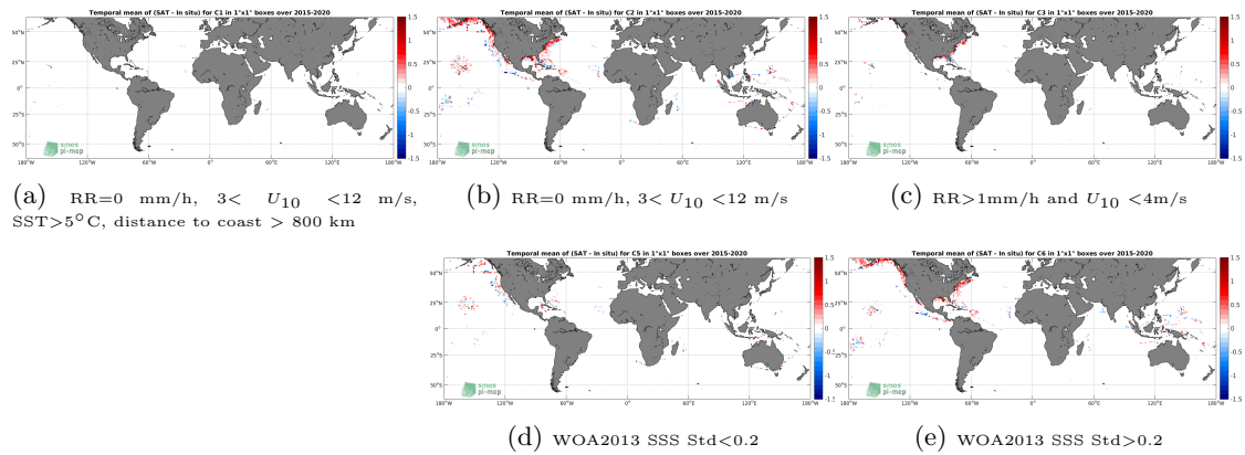
Figure 12: Temporal mean gridded over spatial boxes of size 1^\circ \times 1^\circ of \Delta SSS (SMAP-L2-RSS-V4 - TSG-SAMOS) for 5 different subdatasets corresponding to:RR=0 mm/h, 3 < U_{10} < 12 m/s, SST >5^\circ C, distance to coast > 800 km (a), RR=0 mm/h, 3 < U_{10} < 12 m/s (b), RR >1 mm/h and U_{10} < 4 m/s (c), WOA2013 SSS Std <0.2 (d), WOA2013 SSS Std >0.2 (e).
