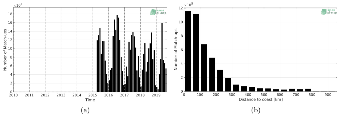
Figure 1: Number of match-ups between TSG-SAMOS and SMAP-L2-RSS-V4 SSS as a function of time (a) and as function of the distance to coast (b) over the SMOS coastal zone ( \pm 800 km) 60N-60S Pi-MEP region and for the full satellite product period.
