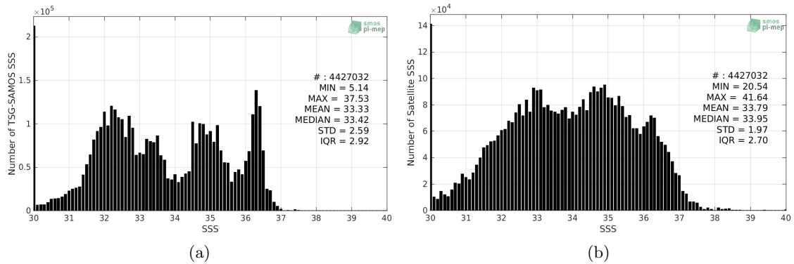
Figure 2: Histograms of SSS from TSG-SAMOS (a) and SMAP-L2-RSS-V4 (b) considering all match-up pairs per bins of 0.1 over the SMOS coastal zone ( \approx 800\text{km} ) 60N-60S Pi-MEP region and for the full satellite product period.
