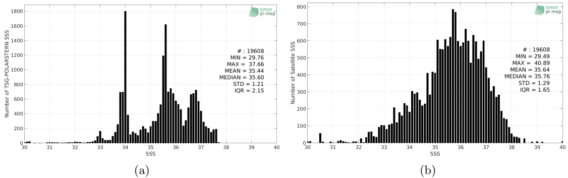
Figure 2: Histograms of SSS from TSG-POLARSTERN (a) and SMAP-L2-RSS-V4 (b) considering all match-up pairs per bins of 0.1 over the SMOS coastal zone (<800km) 60N-60S Pi-MEP region and for the full satellite product period.
