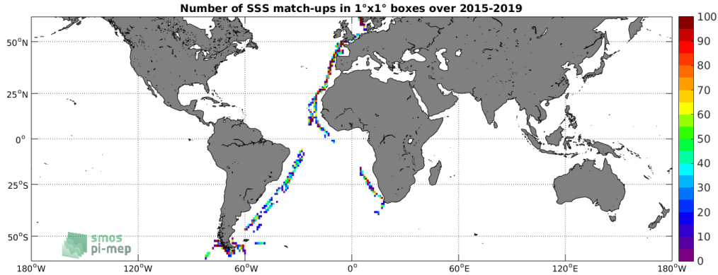
Figure 4: Number of SSS match-ups between TSG-POLARSTERN SSS and the SMAP-L2-RSS-V4 SSS product for the SMOS coastal zone (<800km) 60N-60S Pi-MEP region over 1^\circ \times 1^\circ boxes and for the full satellite product period.
