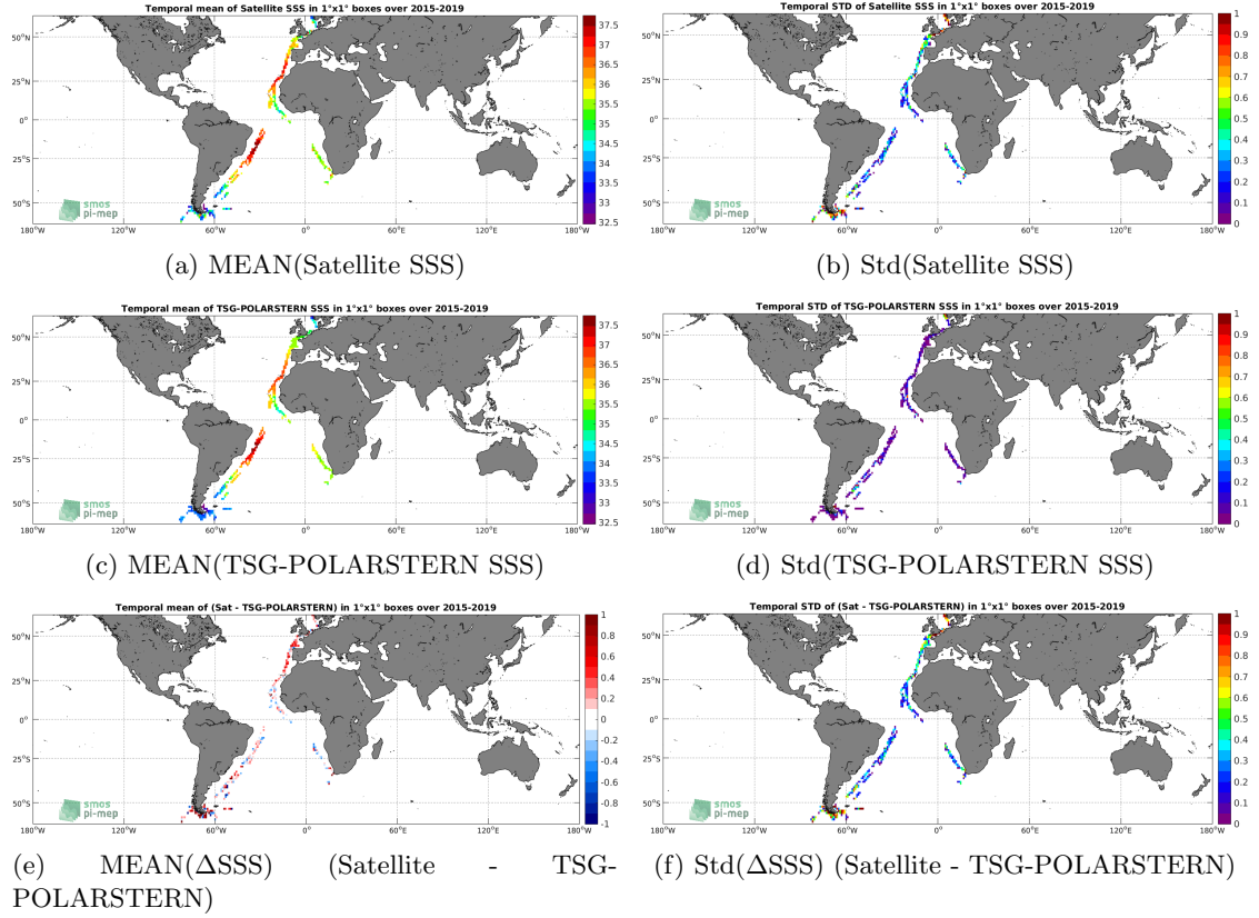
Figure 6: Temporal mean (left) and Std (right) of SSS from SMAP-L2-RSS-V4 (top), TSG-POLARSTERN (middle), and of \Delta SSS (Satellite - TSG-POLARSTERN). Only match-up pairs are used to generate these maps.
