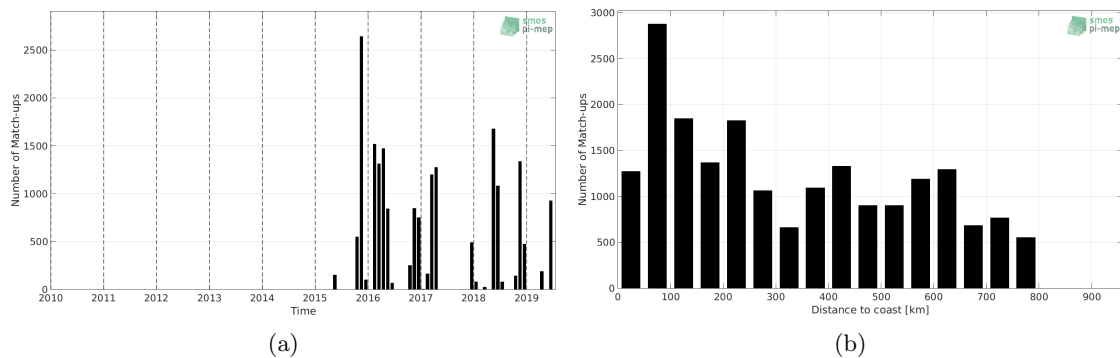
Figure 1: Number of match-ups between TSG-POLARSTERN and SMAP-L2-RSS-V4 SSS as a function of time (a) and as function of the distance to coast (b) over the SMOS coastal zone (<800km) 60N-60S Pi-MEP region and for the full satellite product period.
