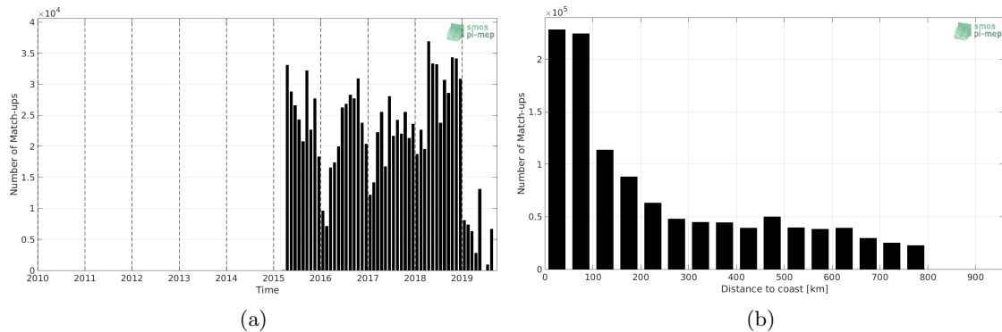
Figure 1: Number of match-ups between TSG (LEGOS-DM) and SMAP SSS L2 v4 (RSS) SSS as a function of time (a) and as function of the distance to coast (b) over the SMOS coastal zone (<800km) 60N-60S Pi-MEP region and for the full satellite product period.
