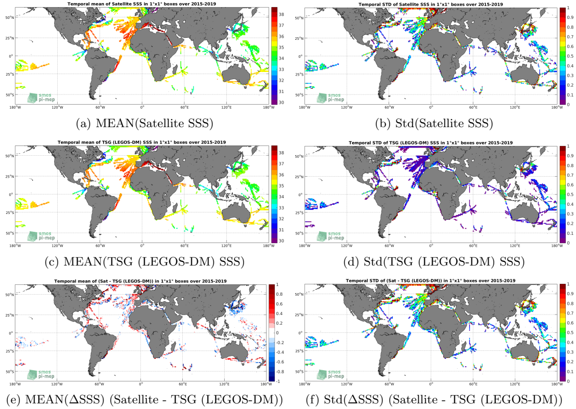
Figure 6: Temporal mean (left) and Std (right) of SSS from SMAP SSS L2 v4 (RSS) (top), TSG (LEGOS-DM) (middle), and of \Delta SSS (Satellite - TSG (LEGOS-DM)). Only match-up pairs are used to generate these maps.
