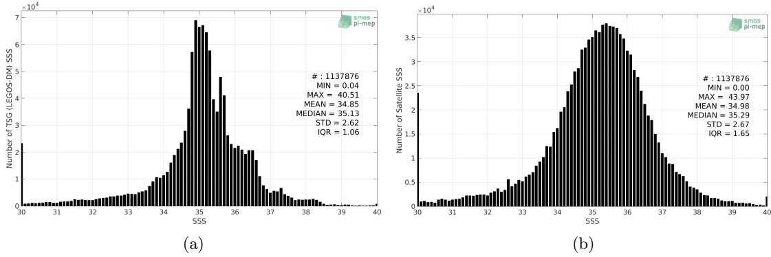
Figure 2: Histograms of SSS from TSG (LEGOS-DM) (a) and SMAP SSS L2 v4 (RSS) (b) considering all match-up pairs per bins of 0.1 over the SMOS coastal zone (<800km) 60N-60S Pi-MEP region and for the full satellite product period.
