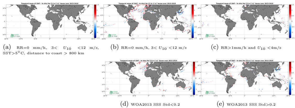
Figure 12: Temporal mean gridded over spatial boxes of size 1^\circ \times 1^\circ of \Delta SSS (SMAP SSS L2 v4 (RSS) - TSG (LEGOS-DM)) for 5 different subdatasets corresponding to:RR=0 mm/h, 3 < U_{10} < 12 m/s, SST >5^\circ\text{C} , distance to coast > 800 km (a), RR=0 mm/h, 3 < U_{10} < 12 m/s (b), RR >1 mm/h and U_{10} < 4 m/s (c), WOA2013 SSS Std <0.2 (d), WOA2013 SSS Std >0.2 (e).
