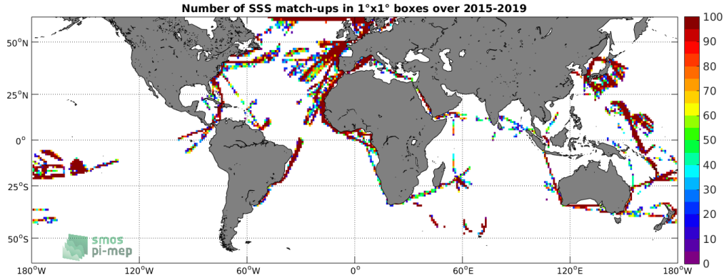
Figure 4: Number of SSS match-ups between TSG (LEGOS-DM) SSS and the SMAP SSS L2 v4 (RSS) SSS product for the SMOS coastal zone (<800km) 60N-60S Pi-MEP region over 1^\circ \times 1^\circ boxes and for the full satellite product period.
