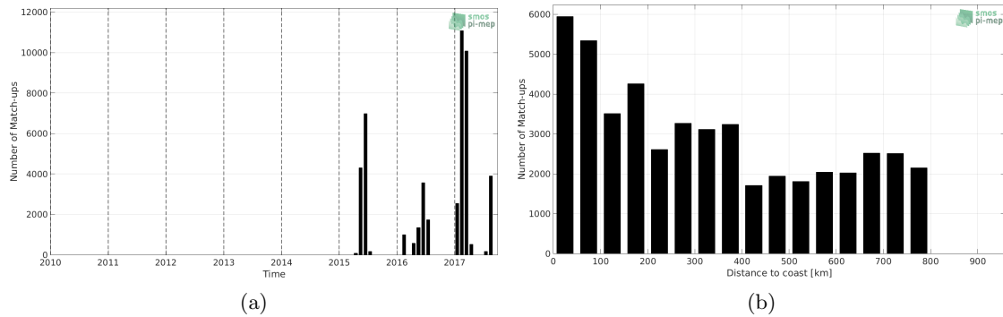
Figure 1: Number of match-ups between TSG (GOSUD-Sailing-ship) and SMAP SSS L2 v4 (RSS) SSS as a function of time (a) and as function of the distance to coast (b) over the SMOS coastal zone (<800km) 60N-60S Pi-MEP region and for the full satellite product period.
