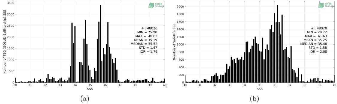
Figure 2: Histograms of SSS from TSG (GOSUD-Sailing-ship) (a) and SMAP SSS L2 v4 (RSS) (b) considering all match-up pairs per bins of 0.1 over the SMOS coastal zone (<800km) 60N-60S Pi-MEP region and for the full satellite product period.
