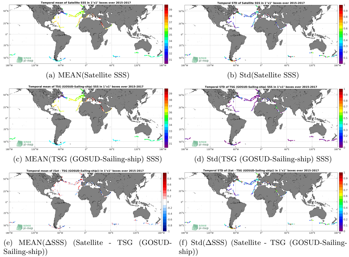
Figure 6: Temporal mean (left) and Std (right) of SSS from SMAP SSS L2 v4 (RSS) (top), TSG (GOSUD-Sailing-ship) (middle), and of \Delta SSS (Satellite - TSG (GOSUD-Sailing-ship)). Only match-up pairs are used to generate these maps.
