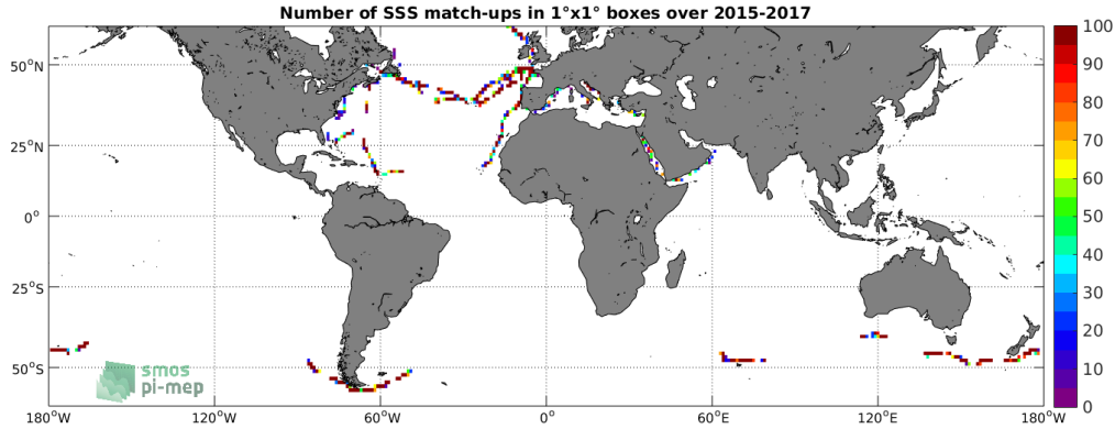
Figure 4: Number of SSS match-ups between TSG (GOSUD-Sailing-ship) SSS and the SMAP SSS L2 v4 (RSS) SSS product for the SMOS coastal zone (<800km) 60N-60S Pi-MEP region over 1^\circ \times 1^\circ boxes and for the full satellite product period.
