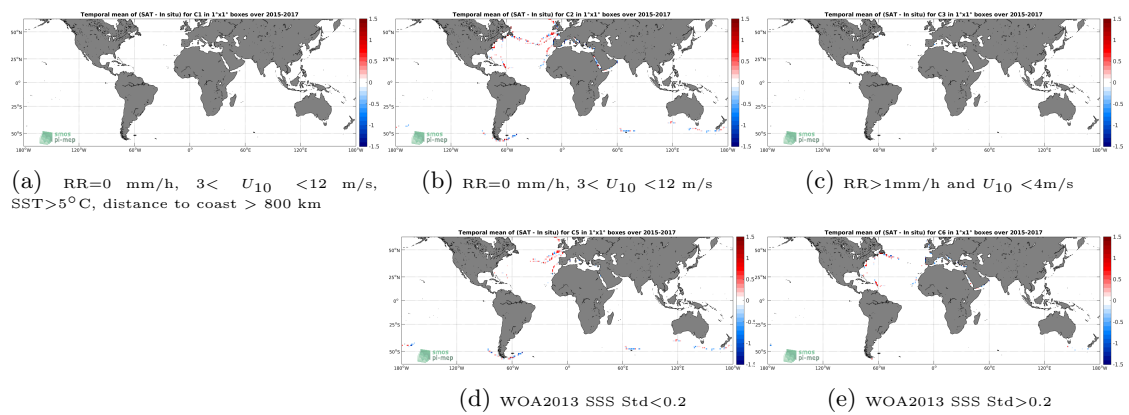
Figure 12: Temporal mean gridded over spatial boxes of size 1^\circ \times 1^\circ of \Delta SSS (SMAP SSS L2 v4 (RSS) - TSG (GOSUD-Sailing-ship)) for 5 different subdatasets corresponding to: RR=0 mm/h, 3 < U_{10} < 12 m/s, SST > 5°C, distance to coast > 800 km (a), RR=0 mm/h, 3 < U_{10} < 12 m/s (b), RR > 1mm/h and U_{10} < 4 m/s (c), WOA2013 SSS Std < 0.2 (d), WOA2013 SSS Std > 0.2 (e).
