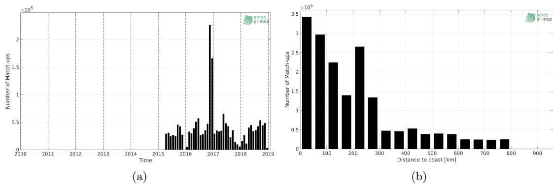
Figure 1: Number of match-ups between TSG-GOSUD-Research-vessel and SMAP-L2-RSS-V4 SSS as a function of time (a) and as function of the distance to coast (b) over the SMOS coastal zone (<800km) 60N-60S Pi-MEP region and for the full satellite product period.
