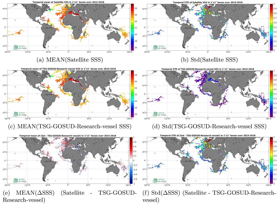
Figure 6: Temporal mean (left) and Std (right) of SSS from SMAP-L2-RSS-V4 (top), TSG-GOSUD-Research-vessel (middle), and of \Delta SSS (Satellite - TSG-GOSUD-Research-vessel). Only match-up pairs are used to generate these maps.
