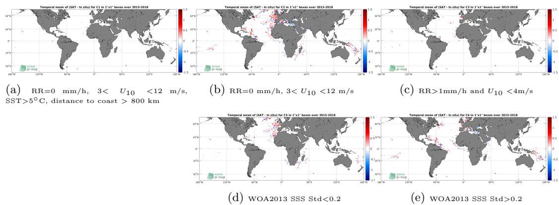
Figure 12: Temporal mean gridded over spatial boxes of size 1^\circ \times 1^\circ of \Delta SSS (SMAP-L2-RSS-V4 - TSG-GOSUD-Research-vessel) for 5 different subdatasets corresponding to:RR=0 mm/h, 3 < U_{10} < 12 m/s, SST >5^\circ\text{C} , distance to coast > 800 km (a), RR=0 mm/h, 3 < U_{10} < 12 m/s (b), RR >1 mm/h and U_{10} < 4 m/s (c), WOA2013 SSS Std <0.2 (d), WOA2013 SSS Std >0.2 (e).
