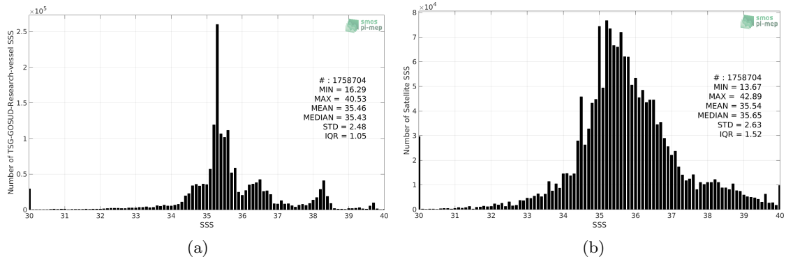
Figure 2: Histograms of SSS from TSG-GOSUD-Research-vessel (a) and SMAP-L2-RSS-V4 (b) considering all match-up pairs per bins of 0.1 over the SMOS coastal zone (<800km) 60N-60S Pi-MEP region and for the full satellite product period.
