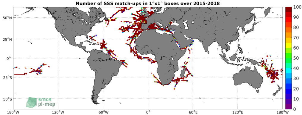
Figure 4: Number of SSS match-ups between TSG-GOSUD-Research-vessel SSS and the SMAP-L2-RSS-V4 SSS product for the SMOS coastal zone (<800km) 60N-60S Pi-MEP region over 1^\circ \times 1^\circ boxes and for the full satellite product period.
