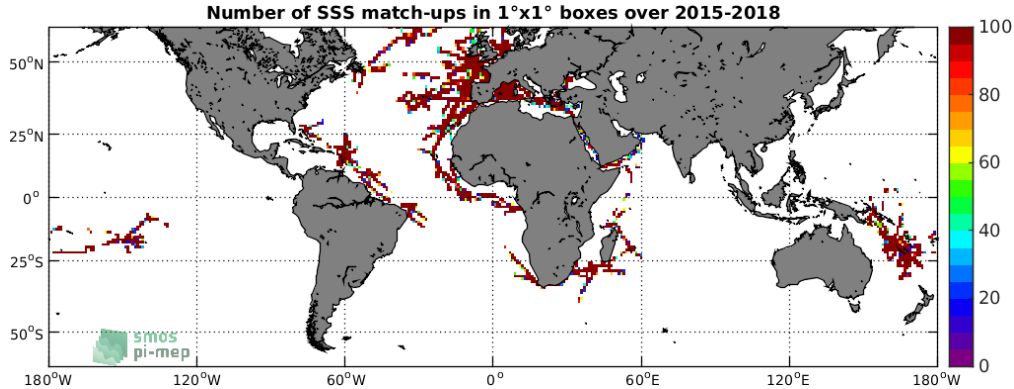
Figure 4: Number of SSS match-ups between TSG-GOSUD-Research-vessel SSS and the SMAP-L2-RSS-V4 SSS product for the SMOS coastal zone ( \approx 800\text{km} ) 60N-60S Pi-MEP region over 1^\circ \times 1^\circ boxes and for the full satellite product period.
