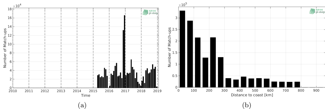
Figure 1: Number of match-ups between TSG-GOSUD-Research-vessel and SMAP-L2-RSS-V4 SSS as a function of time (a) and as function of the distance to coast (b) over the SMOS coastal zone ( \approx 800 km) 60N-60S Pi-MEP region and for the full satellite product period.
