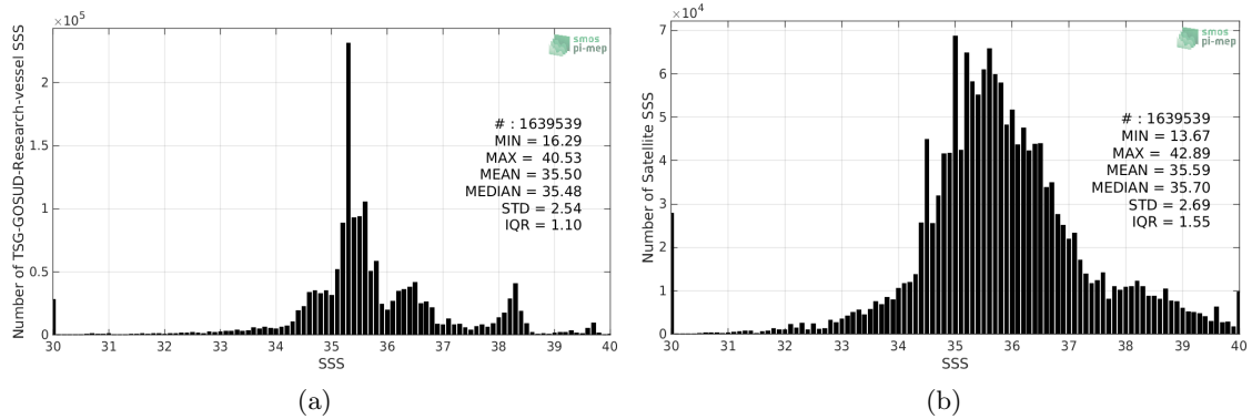
Figure 2: Histograms of SSS from TSG-GOSUD-Research-vessel (a) and SMAP-L2-RSS-V4 (b) considering all match-up pairs per bins of 0.1 over the SMOS coastal zone ( \approx 800\text{km} ) 60N-60S Pi-MEP region and for the full satellite product period.
