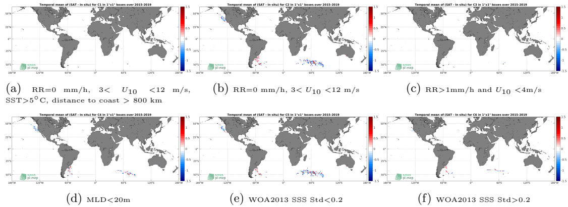
Figure 12: Temporal mean gridded over spatial boxes of size 1^\circ \times 1^\circ of \Delta SSS (SMAP SSS L2 v4 (RSS) - Marine mammals) for 6 different subdatasets corresponding to: RR=0 mm/h, 3 < U_{10} < 12 m/s, SST > 5°C, distance to coast > 800 km (a), RR=0 mm/h, 3 < U_{10} < 12 m/s (b), RR > 1mm/h and U_{10} < 4 m/s (c), MLD < 20m (d), WOA2013 SSS Std < 0.2 (e), WOA2013 SSS Std > 0.2 (f).
