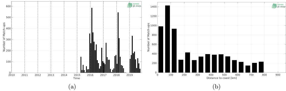
Figure 1: Number of match-ups between Marine mammals and SMAP SSS L2 v4 (RSS) SSS as a function of time (a) and as function of the distance to coast (b) over the SMOS coastal zone (<800km) 60N-60S Pi-MEP region and for the full satellite product period.
