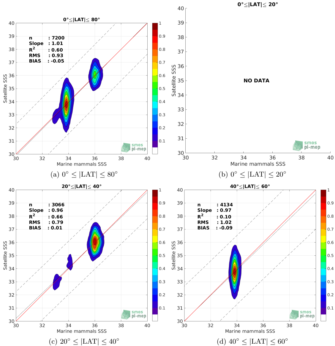
Figure 9: Contour maps of the concentration of SMAP SSS L2 v4 (RSS) SSS (y-axis) versus Marine mammals SSS (x-axis) at match-up pairs for different latitude bands. For each plot, the red line shows x=y . The black thin and dashed lines indicate a linear fit through the data cloud and the \pm 95\% confidence levels, respectively. The number match-up pairs n , the slope and R^2 coefficient of the linear fit, the root mean square (RMS) and the mean bias between satellite and in situ data are indicated for each latitude band in each plots.
