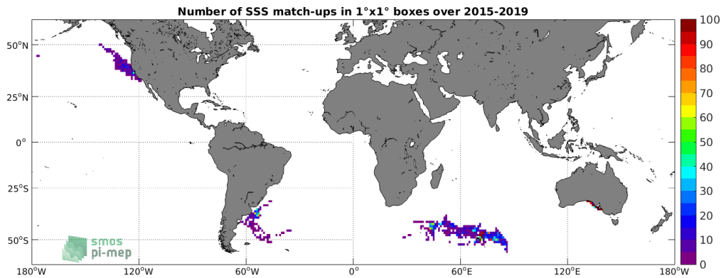
Figure 4: Number of SSS match-ups between Marine mammals SSS and the SMAP SSS L2 v4 (RSS) SSS product for the SMOS coastal zone (<800km) 60N-60S Pi-MEP region over 1^{\circ} \times 1^{\circ} boxes and for the full satellite product period.
