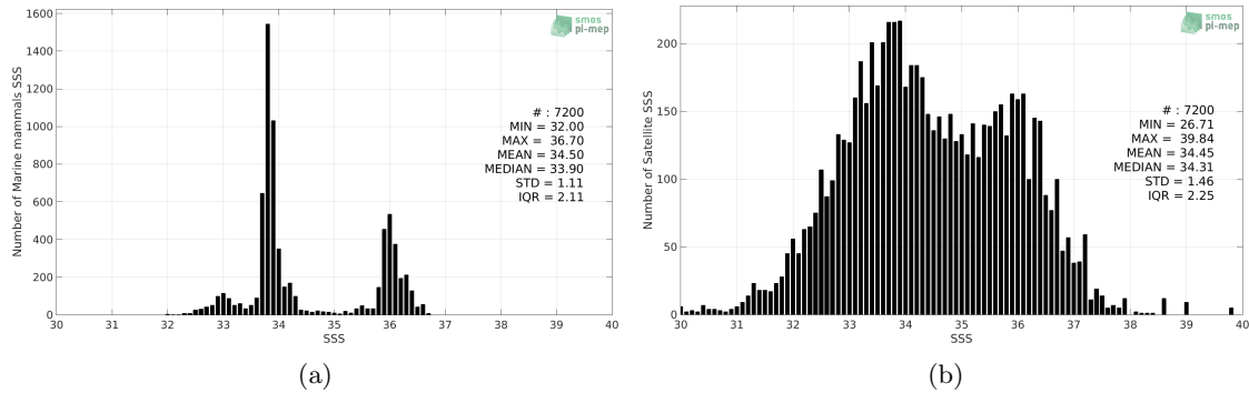
Figure 2: Histograms of SSS from Marine mammals (a) and SMAP SSS L2 v4 (RSS) (b) considering all match-up pairs per bins of 0.1 over the SMOS coastal zone (<800km) 60N-60S Pi-MEP region and for the full satellite product period.
