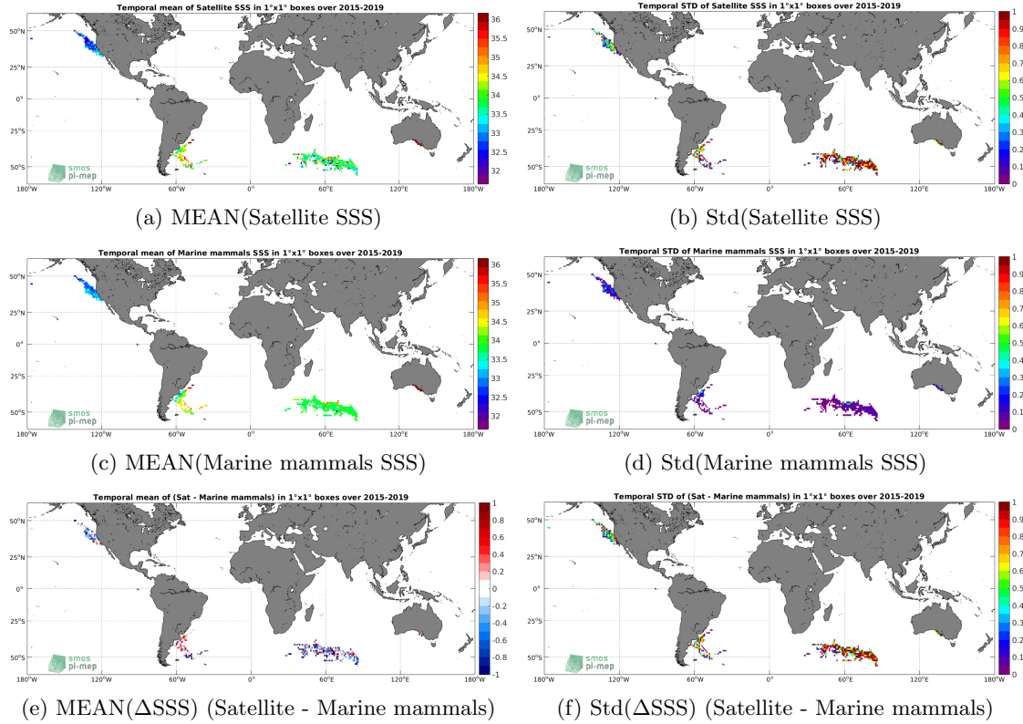
Figure 6: Temporal mean (left) and Std (right) of SSS from SMAP SSS L2 v4 (RSS) (top), Marine mammals (middle), and of \Delta SSS (Satellite - Marine mammals). Only match-up pairs are used to generate these maps.
