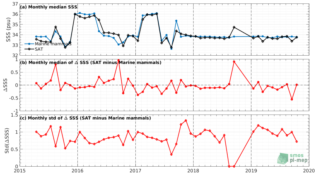
Figure 7: Time series of the monthly median SSS (top), median of \Delta SSS (Satellite - Marine mammals) over the SMOS coastal zone (<800km) 60N-60S Pi-MEP region considering all match-ups collected by the Pi-MEP.
