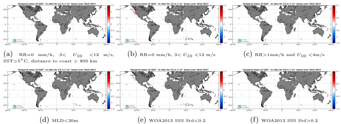
Figure 12: Temporal mean gridded over spatial boxes of size 1^\circ \times 1^\circ of \Delta SSS (SMAP-L2-RSS-V4 - Sea mammals) for 6 different subdatasets corresponding to: RR=0 mm/h, 3 < U_{10} < 12 m/s, SST > 5^\circ\text{C} , distance to coast > 800 km (a), RR=0 mm/h, 3 < U_{10} < 12 m/s (b), RR > 1 mm/h and U_{10} < 4 m/s (c), MLD < 20 m (d), WOA2013 SSS Std < 0.2 (e), WOA2013 SSS Std > 0.2 (f).
