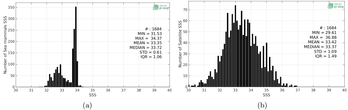
Figure 2: Histograms of SSS from Sea mammals (a) and SMAP-L2-RSS-V4 (b) considering all match-up pairs per bins of 0.1 over the SMOS coastal zone ( \pm 800\text{km} ) 60N-60S Pi-MEP region and for the full satellite product period.
