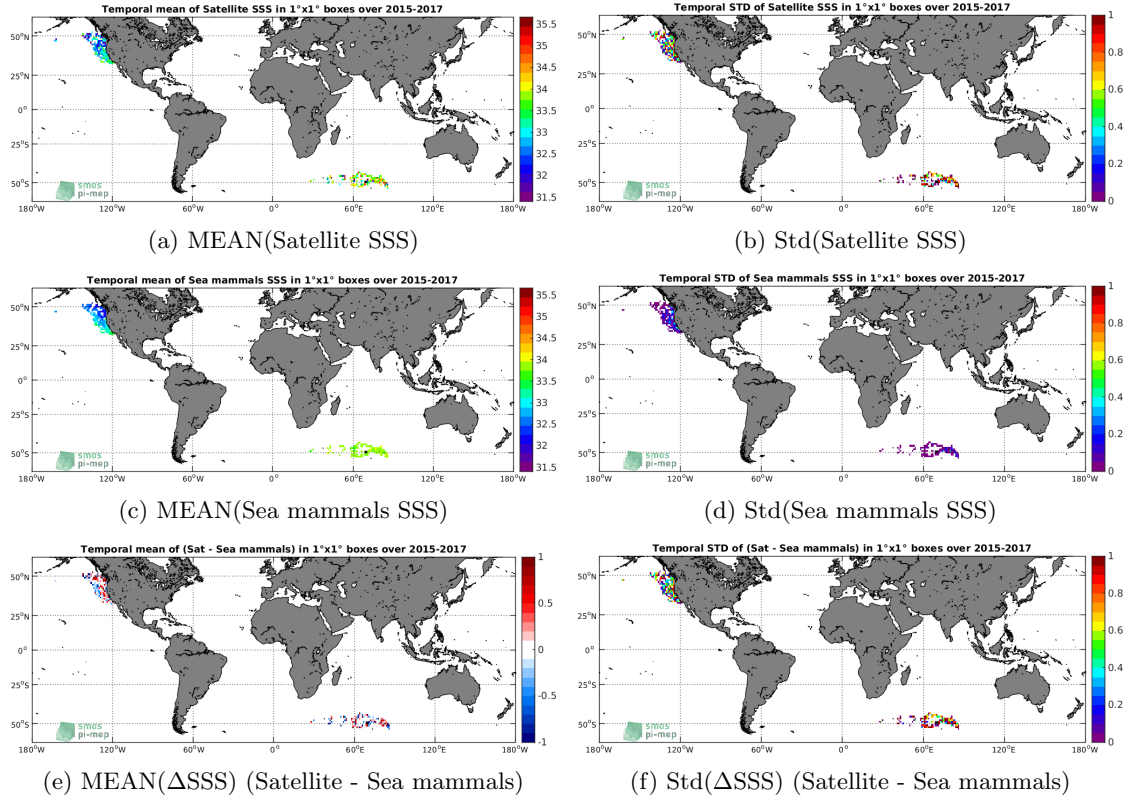
Figure 6: Temporal mean (left) and Std (right) of SSS from SMAP-L2-RSS-V4 (top), Sea mammals (middle), and of \Delta SSS (Satellite - Sea mammals). Only match-up pairs are used to generate these maps.
