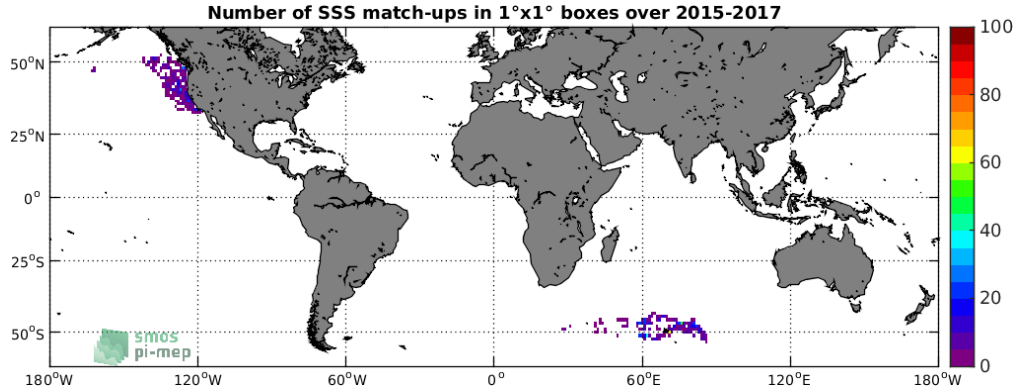
Figure 4: Number of SSS match-ups between Sea mammals SSS and the SMAP-L2-RSS-V4 SSS product for the SMOS coastal zone ( \approx 800\text{km} ) 60N-60S Pi-MEP region over 1^\circ \times 1^\circ boxes and for the full satellite product period.
