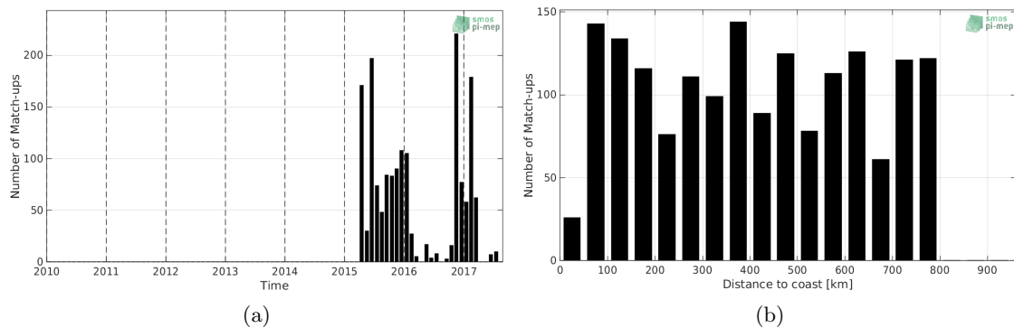
Figure 1: Number of match-ups between Sea mammals and SMAP-L2-RSS-V4 SSS as a function of time (a) and as function of the distance to coast (b) over the SMOS coastal zone ( \leq 800 km) 60N-60S Pi-MEP region and for the full satellite product period.
