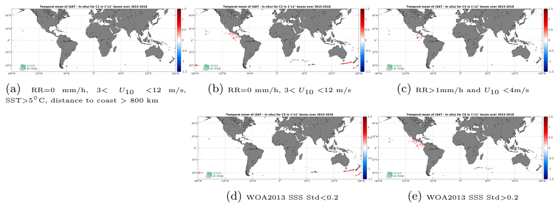
Figure 11: Temporal mean gridded over spatial boxes of size 1^\circ \times 1^\circ of \Delta SSS (SMAP SSS L2 v4 (RSS) - Surface drifters) for 5 different subdatasets corresponding to: RR=0 mm/h, 3 < U_{10} < 12 m/s, SST > 5°C, distance to coast > 800 km (a), RR=0 mm/h, 3 < U_{10} < 12 m/s (b), RR > 1mm/h and U_{10} < 4 m/s (c), WOA2013 SSS Std < 0.2 (d), WOA2013 SSS Std > 0.2 (e).
