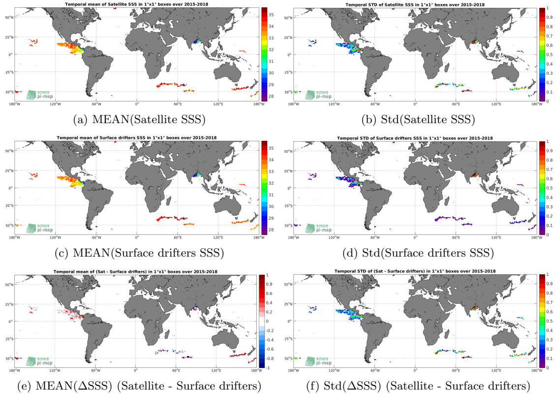
Figure 5: Temporal mean (left) and Std (right) of SSS from SMAP SSS L2 v4 (RSS) (top), Surface drifters (middle), and of \Delta SSS (Satellite - Surface drifters). Only match-up pairs are used to generate these maps.
