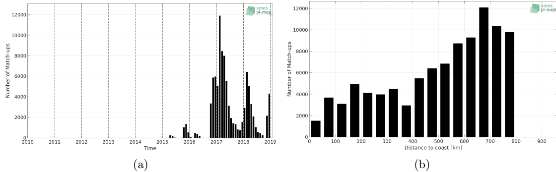
Figure 1: Number of match-ups between Surface drifters and SMAP SSS L2 v4 (RSS) SSS as a function of time (a) and as function of the distance to coast (b) over the SMOS coastal zone (<800km) 60N-60S Pi-MEP region and for the full satellite product period.
