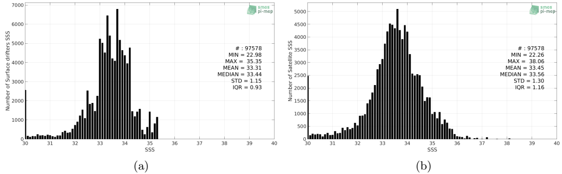
Figure 2: Histograms of SSS from Surface drifters (a) and SMAP SSS L2 v4 (RSS) (b) considering all match-up pairs per bins of 0.1 over the SMOS coastal zone (<800km) 60N-60S Pi-MEP region and for the full satellite product period.
