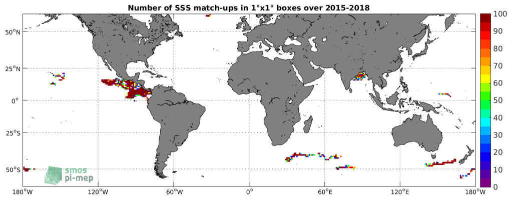
Figure 3: Number of SSS match-ups between Surface drifters SSS and the SMAP SSS L2 v4 (RSS) SSS product for the SMOS coastal zone (<800km) 60N-60S Pi-MEP region over 1°x1° boxes and for the full satellite product period.
