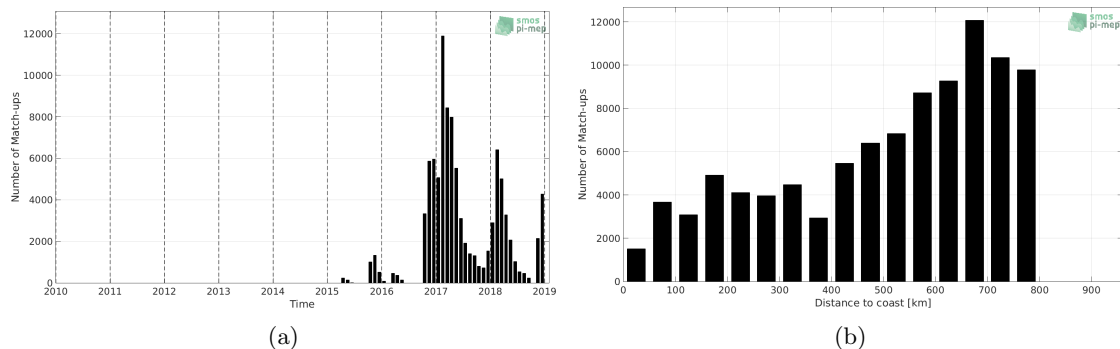
Figure 1: Number of match-ups between Surface drifters and SMAP-L2-RSS-V4 SSS as a function of time (a) and as function of the distance to coast (b) over the SMOS coastal zone (<800km) 60N-60S Pi-MEP region and for the full satellite product period.
