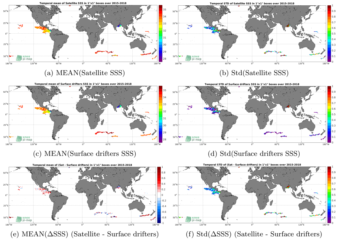
Figure 5: Temporal mean (left) and Std (right) of SSS from SMAP-L2-RSS-V4 (top), Surface drifters (middle), and of \Delta SSS (Satellite - Surface drifters). Only match-up pairs are used to generate these maps.
