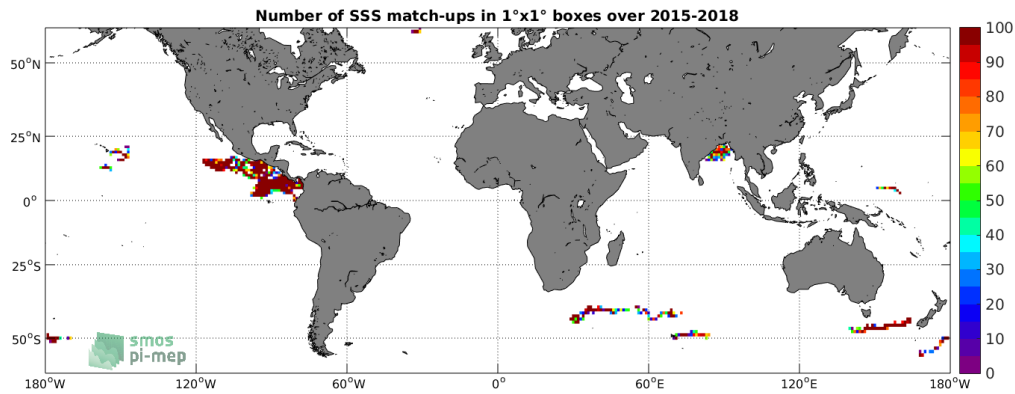
Figure 3: Number of SSS match-ups between Surface drifters SSS and the SMAP-L2-RSS-V4 SSS product for the SMOS coastal zone (<800km) 60N-60S Pi-MEP region over 1°x1° boxes and for the full satellite product period.
