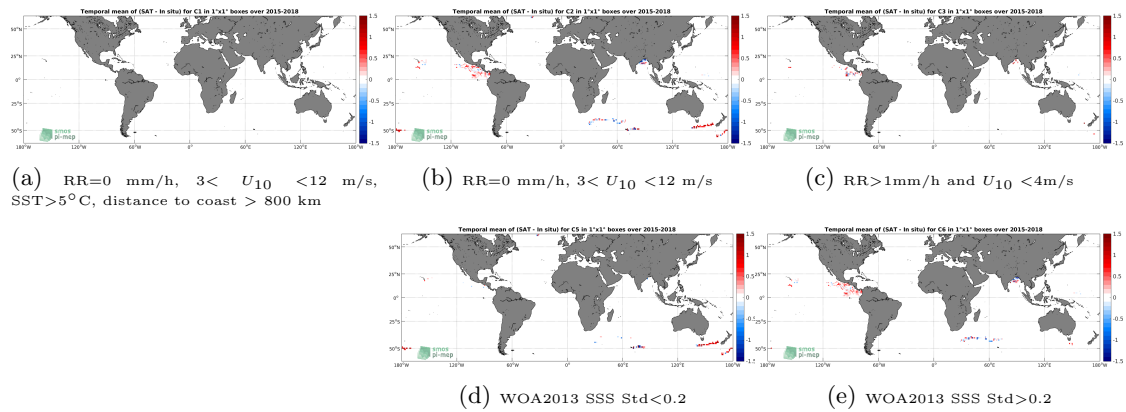
Figure 11: Temporal mean gridded over spatial boxes of size 1^\circ \times 1^\circ of \Delta SSS (SMAP-L2-RSS-V4 - Surface drifters) for 5 different subdatasets corresponding to:RR=0 mm/h, 3 < U_{10} < 12 m/s, SST >5^\circ C, distance to coast > 800 km (a), RR=0 mm/h, 3 < U_{10} < 12 m/s (b), RR >1 mm/h and U_{10} < 4 m/s (c), WOA2013 SSS Std <0.2 (d), WOA2013 SSS Std >0.2 (e).
