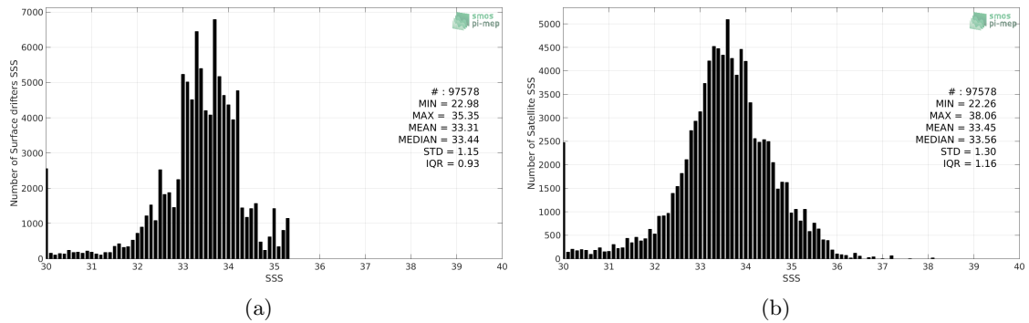
Figure 2: Histograms of SSS from Surface drifters (a) and SMAP-L2-RSS-V4 (b) considering all match-up pairs per bins of 0.1 over the SMOS coastal zone (<800km) 60N-60S Pi-MEP region and for the full satellite product period.
