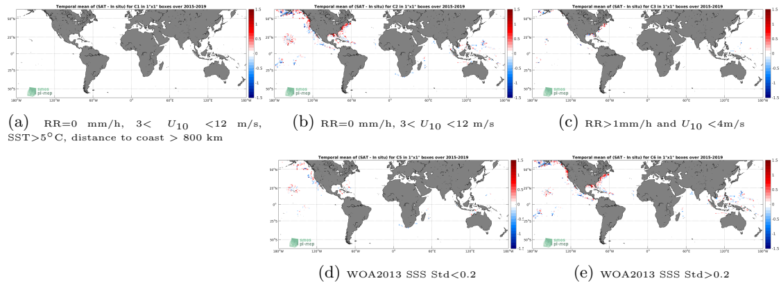
Figure 12: Temporal mean gridded over spatial boxes of size 1^\circ \times 1^\circ of \Delta SSS (SMAP-L2-RSS-V3-70KM - TSG-SAMOS) for 5 different subdatasets corresponding to:RR=0 mm/h, 3 < U_{10} < 12 m/s, SST >5^\circ C, distance to coast > 800 km (a), RR=0 mm/h, 3 < U_{10} < 12 m/s (b), RR >1 mm/h and U_{10} < 4 m/s (c), WOA2013 SSS Std <0.2 (d), WOA2013 SSS Std >0.2 (e).
