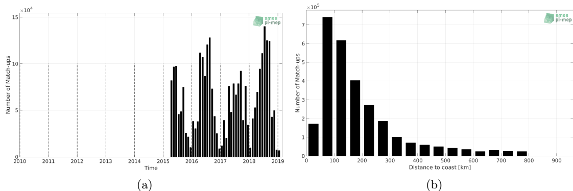
Figure 1: Number of match-ups between TSG-SAMOS and SMAP-L2-RSS-V3-70KM SSS as a function of time (a) and as function of the distance to coast (b) over the SMOS coastal zone ( \pm 800 km) 60N-60S Pi-MEP region and for the full satellite product period.
