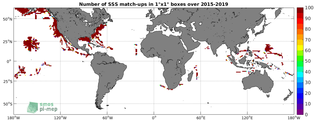
Figure 4: Number of SSS match-ups between TSG-SAMOS SSS and the SMAP-L2-RSS-V3-70KM SSS product for the SMOS coastal zone ( \geq 800\text{km} ) 60N-60S Pi-MEP region over 1^\circ \times 1^\circ boxes and for the full satellite product period.
