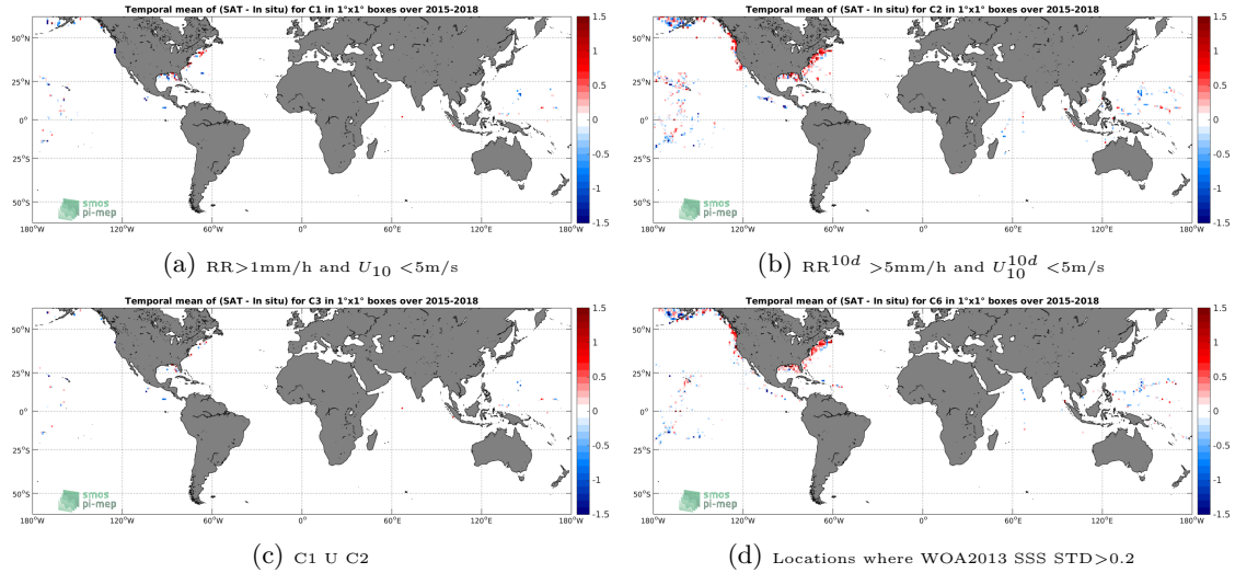
Figure 12: Temporal mean gridded over spatial boxes of size 1^\circ \times 1^\circ of \Delta SSS (SMAP-L2-RSS-V3-70KM - TSG-SAMOS) for 4 different subdatasets corresponding to: RR > 1\text{mm/h} and U_{10} < 5\text{m/s} (a), RR^{10d} > 5\text{mm/h} and U_{10}^{10d} < 5\text{m/s} (b), C1 U C2 (c), Locations where WOA2013 SSS STD > 0.2 (d).
