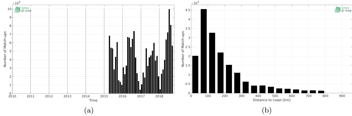
Figure 1: Number of match-ups between TSG-SAMOS and SMAP-L2-RSS-V3-70KM SSS as a function of time (a) and as function of the distance to coast (b) over the SMOS coastal zone ( \pm 800\text{km} ) 60N-60S Pi-MEP region and for the full satellite product period.
