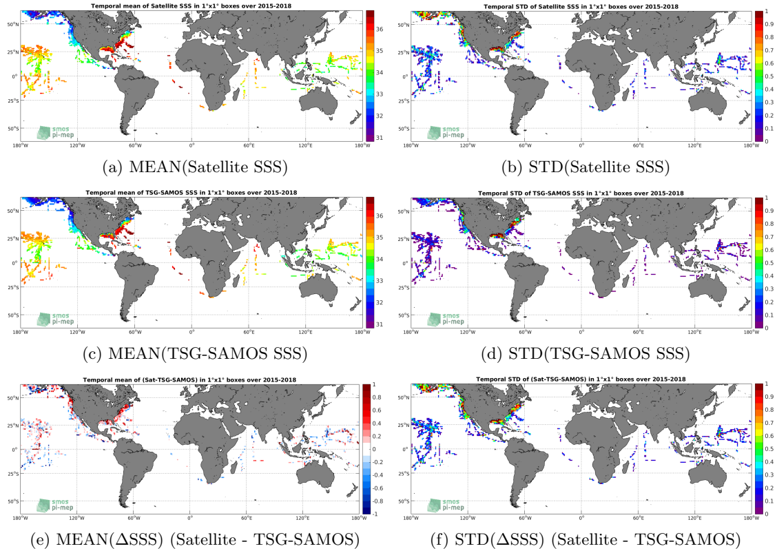
Figure 6: Temporal mean (left) and STD (right) of SSS from SMAP-L2-RSS-V3-70KM (top), TSG-SAMOS (middle), and of \Delta SSS (Satellite - TSG-SAMOS). Only match-up pairs are used to generate these maps.
