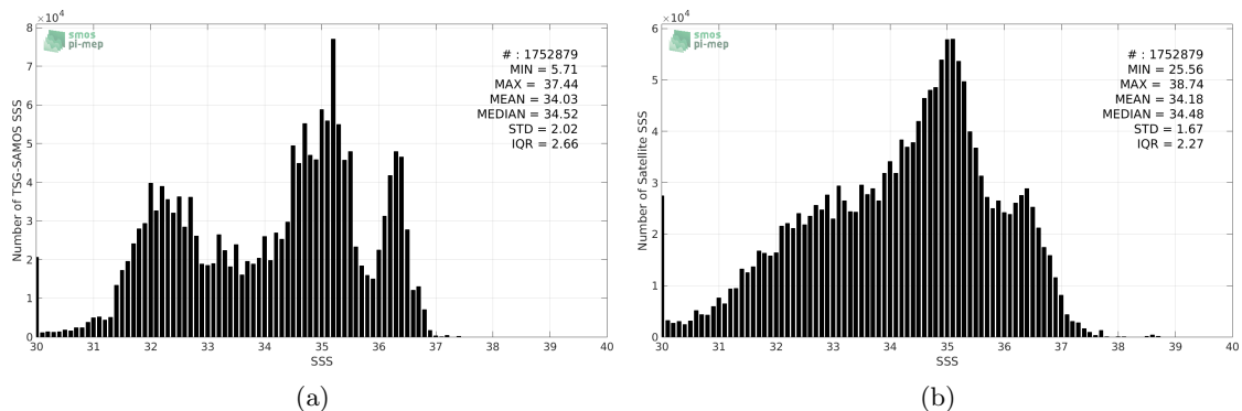
Figure 2: Histograms of SSS from TSG-SAMOS (a) and SMAP-L2-RSS-V3-70KM (b) considering all match-up pairs per bins of 0.1 over the SMOS coastal zone ( \pm 800\text{km} ) 60N-60S Pi-MEP region and for the full satellite product period.
