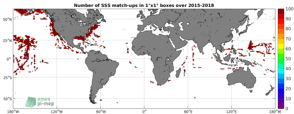
Figure 4: Number of SSS match-ups between TSG-SAMOS SSS and the SMAP-L2-RSS-V3-70KM SSS product for the SMOS coastal zone ( \approx 800\text{km} ) 60N-60S Pi-MEP region over 1^\circ \times 1^\circ boxes and for the full satellite product period.
