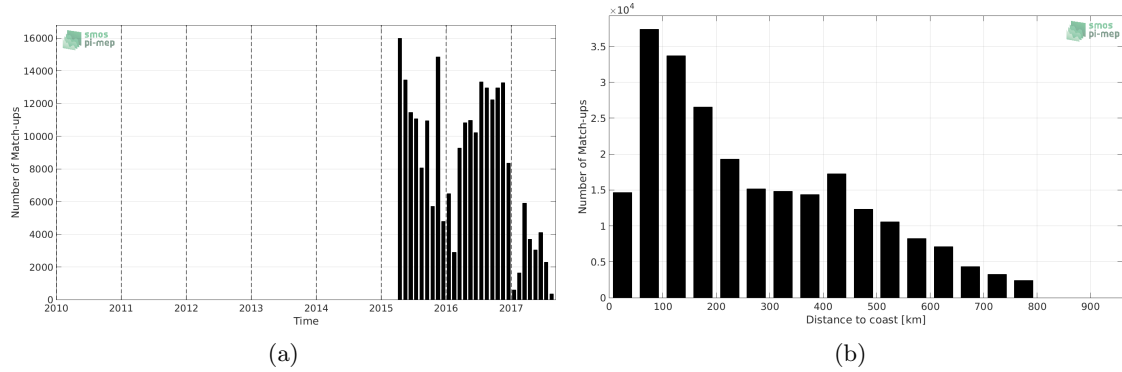
Figure 1: Number of match-ups between TSG-LEGOS-DM and SMAP-L2-RSS-V3-70KM SSS as a function of time (a) and as function of the distance to coast (b) over the SMOS coastal zone ( \approx 800 km) 60N-60S Pi-MEP region and for the full satellite product period.
