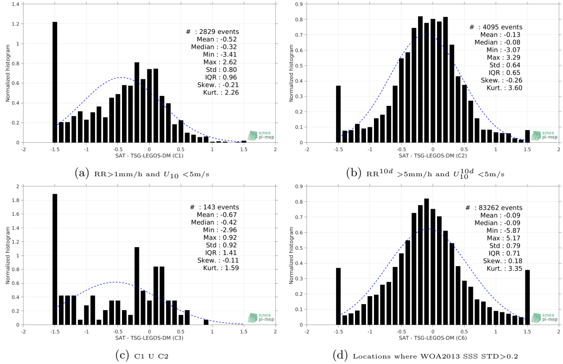
Figure 13: Normalized histogram of \Delta SSS (SMAP-L2-RSS-V3-70KM - TSG-LEGOS-DM) for 6 different subdatasets corresponding to: RR > 1mm/h and U_{10} < 5 m/s (a), RR^{10d} > 5 mm/h and U_{10}^{10d} < 5 m/s (b), C1 U C2 (c), Locations where WOA2013 SSS STD > 0.2 (d).
