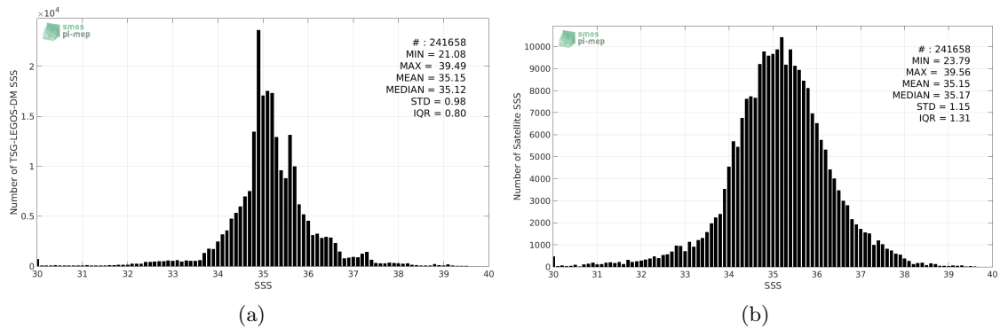
Figure 2: Histograms of SSS from TSG-LEGOS-DM (a) and SMAP-L2-RSS-V3-70KM (b) considering all match-up pairs per bins of 0.1 over the SMOS coastal zone ( \approx 800 km) 60N-60S Pi-MEP region and for the full satellite product period.
