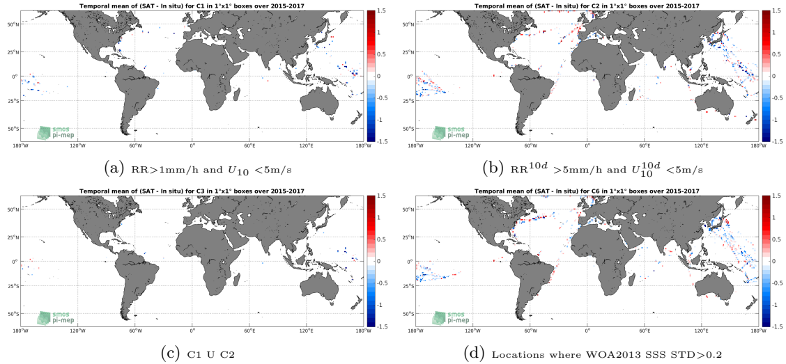
Figure 12: Temporal mean gridded over spatial boxes of size 1^\circ \times 1^\circ of \Delta SSS (SMAP-L2-RSS-V3-70KM - TSG-LEGOS-DM) for 4 different subdatasets corresponding to: RR > 1mm/h and U_{10} < 5\text{m/s} (a), RR^{10d} > 5\text{mm/h} and U_{10}^{10d} < 5\text{m/s} (b), C1 U C2 (c), Locations where WOA2013 SSS STD > 0.2 (d).
