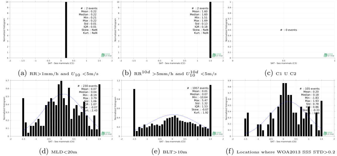
Figure 13: Normalized histogram of \Delta\text{SSS} (SMAP-L2-RSS-V3-70KM - Sea mammals) for 6 different subdatasets corresponding to: \text{RR}>1\text{mm/h} and U_{10}<5\text{m/s} (a), \text{RR}^{10d}>5\text{mm/h} and U_{10}^{10d}<5\text{m/s} (b), C1 U C2 (c), \text{MLD}<20\text{m} (d), \text{BLT}>10\text{m} (e), Locations where WOA2013 SSS STD >0.2 (f).
