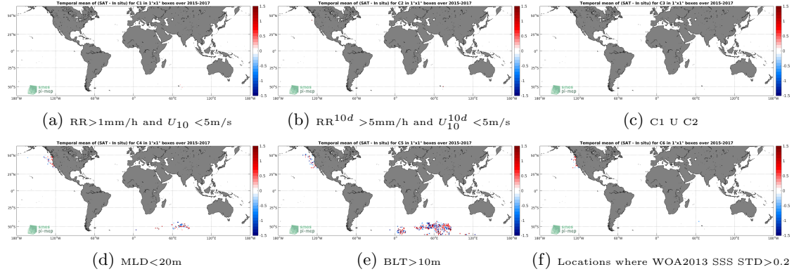
Figure 12: Temporal mean gridded over spatial boxes of size 1^\circ \times 1^\circ of \Delta\text{SSS} (SMAP-L2-RSS-V3-70KM - Sea mammals) for 6 different subdatasets corresponding to: \text{RR}>1\text{mm/h} and U_{10}<5\text{m/s} (a), \text{RR}^{10d}>5\text{mm/h} and U_{10}^{10d}<5\text{m/s} (b), C1 U C2 (c), \text{MLD}<20\text{m} (d), \text{BLT}>10\text{m} (e), Locations where WOA2013 SSS STD >0.2 (f).
