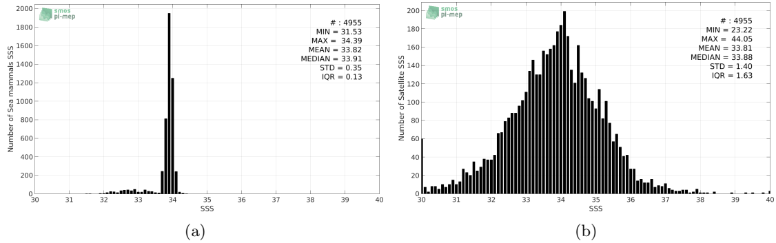
Figure 2: Histograms of SSS from Sea mammals (a) and SMAP-L2-RSS-V3-70KM (b) considering all match-up pairs per bins of 0.1 over the SMOS coastal zone ( \pm 800 km) 60N-60S Pi-MEP region and for the full satellite product period.
