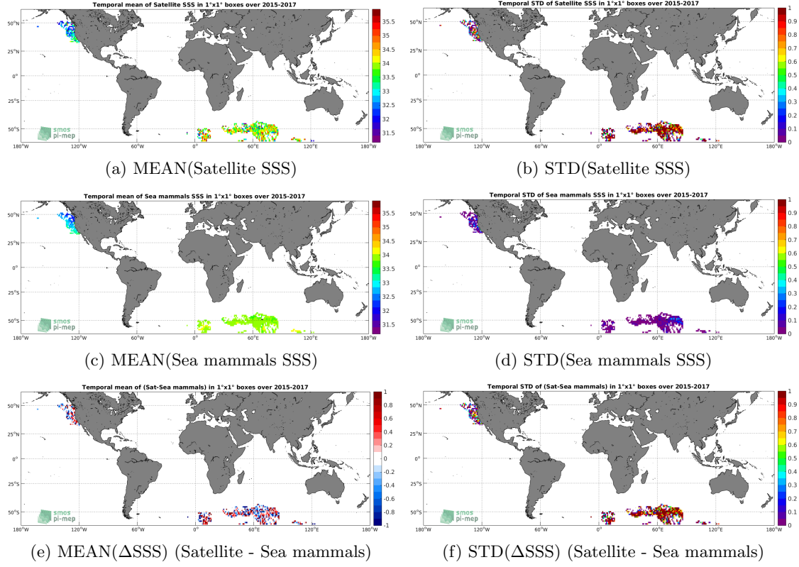
Figure 6: Temporal mean (left) and STD (right) of SSS from SMAP-L2-RSS-V3-70KM (top), Sea mammals (middle), and of \Delta SSS (Satellite - Sea mammals). Only match-up pairs are used to generate these maps.
