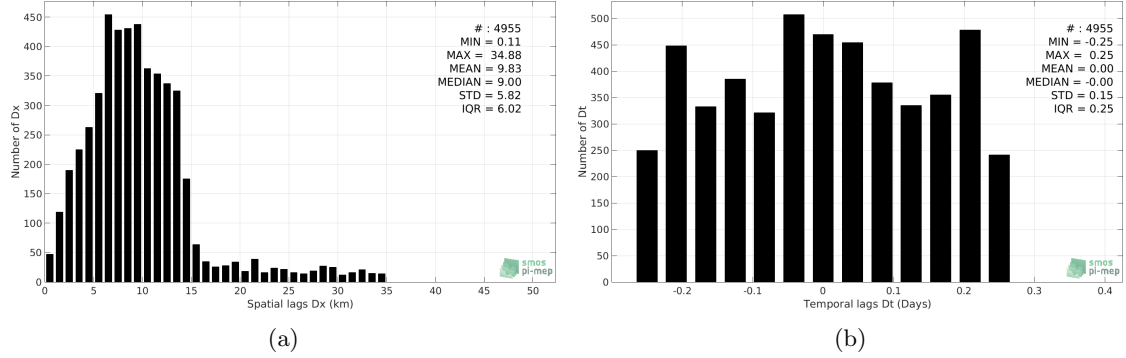
Figure 5: Histograms of the spatial (a) and temporal (b) lags between the time of the Sea mammals measurements and the date of the corresponding SMAP-L2-RSS-V3-70KM SSS product.
