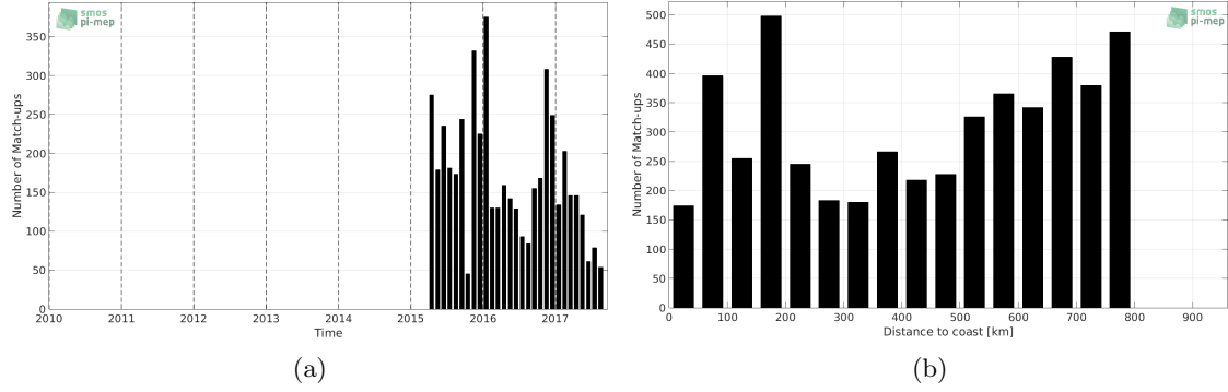
Figure 1: Number of match-ups between Sea mammals and SMAP-L2-RSS-V3-70KM SSS as a function of time (a) and as function of the distance to coast (b) over the SMOS coastal zone ( \pm 800 km) 60N-60S Pi-MEP region and for the full satellite product period.
