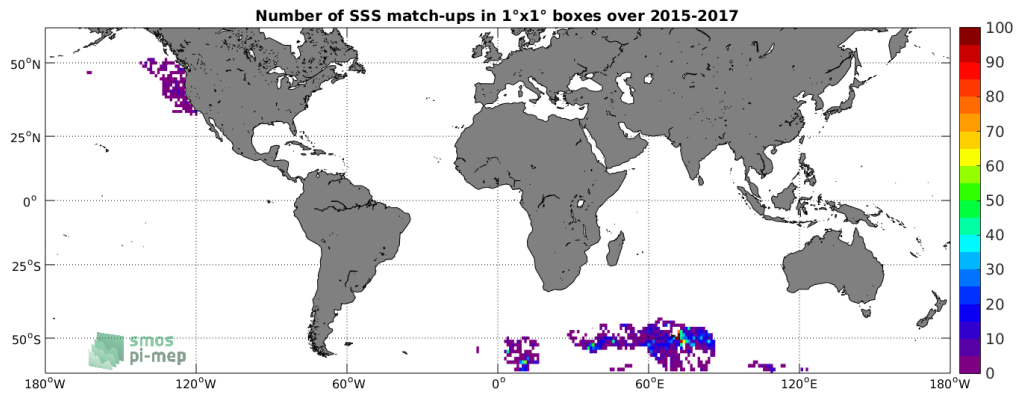
Figure 4: Number of SSS match-ups between Sea mammals SSS and the SMAP-L2-RSS-V3-70KM SSS product for the SMOS coastal zone ( \pm 800\text{km} ) 60N-60S Pi-MEP region over 1^\circ \times 1^\circ boxes and for the full satellite product period.
