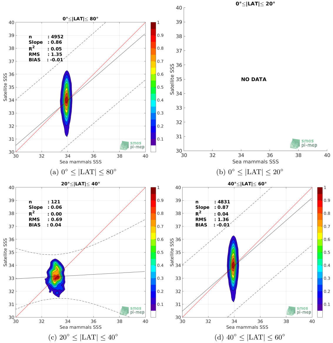
Figure 9: Contour maps of the concentration of SMAP-L2-RSS-V3-70KM SSS (y-axis) versus Sea mammals SSS (x-axis) at match-up pairs for different latitude bands. For each plot, the red line shows x=y . The black thin and dashed lines indicate a linear fit through the data cloud and the \pm 95\% confidence levels, respectively. The number match-up pairs n , the slope and R^2 coefficient of the linear fit, the root mean square (RMS) and the mean bias between satellite and in situ data are indicated for each latitude band in each plots.
