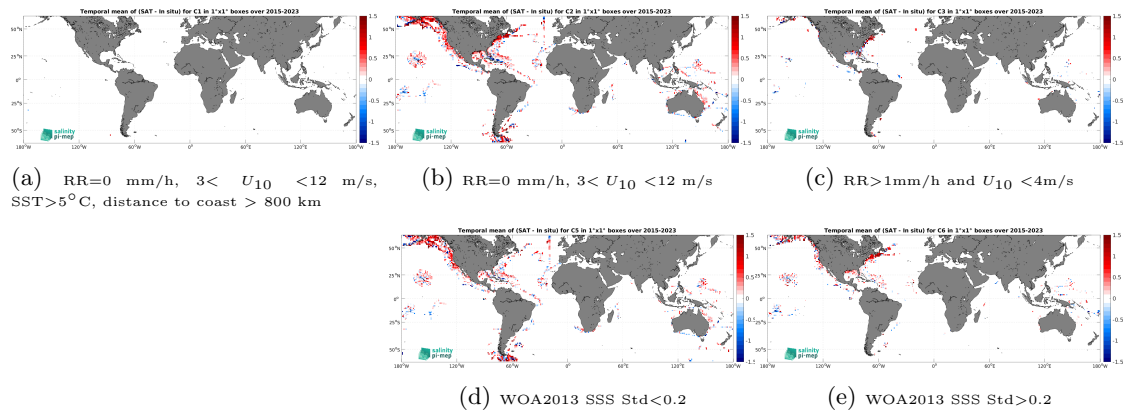
Figure 12: Temporal mean gridded over spatial boxes of size 1^\circ \times 1^\circ of \Delta\text{SSS} (SMAP SSS L2 v5.0 (JPL) - TSG (SAMOS)) for 5 different subdatasets corresponding to:RR=0 mm/h, 3 < U_{10} < 12 m/s, SST >5^\circ\text{C} , distance to coast > 800 km (a), RR=0 mm/h, 3 < U_{10} < 12 m/s (b), RR >1 mm/h and U_{10} < 4 m/s (c), WOA2013 SSS Std <0.2 (d), WOA2013 SSS Std >0.2 (e).
