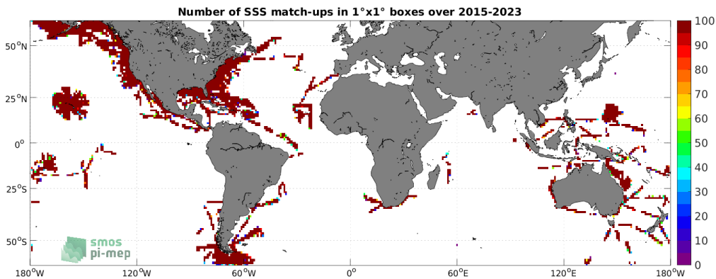
Figure 4: Number of SSS match-ups between TSG (SAMOS) SSS and the SMAP SSS L2 v5.0 (JPL) SSS product for the SMOS coastal zone (<800km) 60N-60S Pi-MEP region over 1°×1° boxes and for the full satellite product period.
