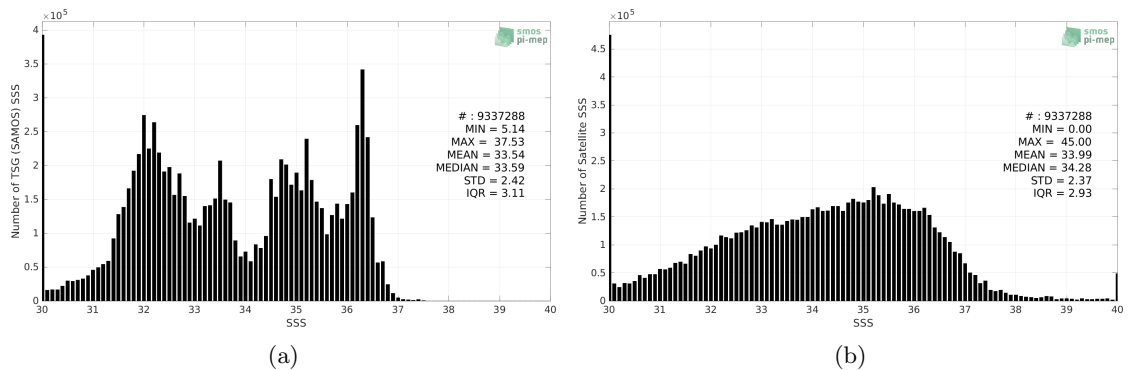
Figure 2: Histograms of SSS from TSG (SAMOS) (a) and SMAP SSS L2 v5.0 (JPL) (b) considering all match-up pairs per bins of 0.1 over the SMOS coastal zone (<800km) 60N-60S Pi-MEP region and for the full satellite product period.
