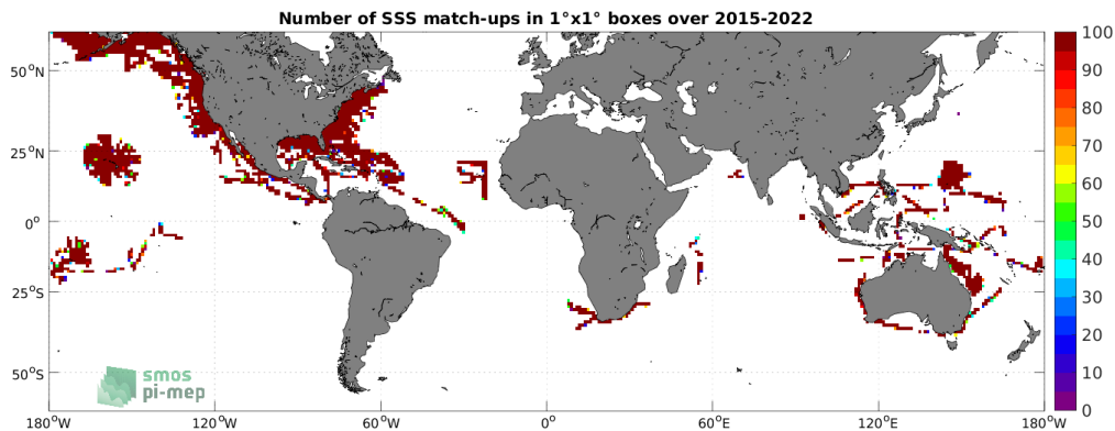
Figure 4: Number of SSS match-ups between TSG (SAMOS) SSS and the SMAP SSS L2 v5.0 (JPL) SSS product for the SMOS coastal zone (<800km) 60N-60S Pi-MEP region over 1^\circ \times 1^\circ boxes and for the full satellite product period.
