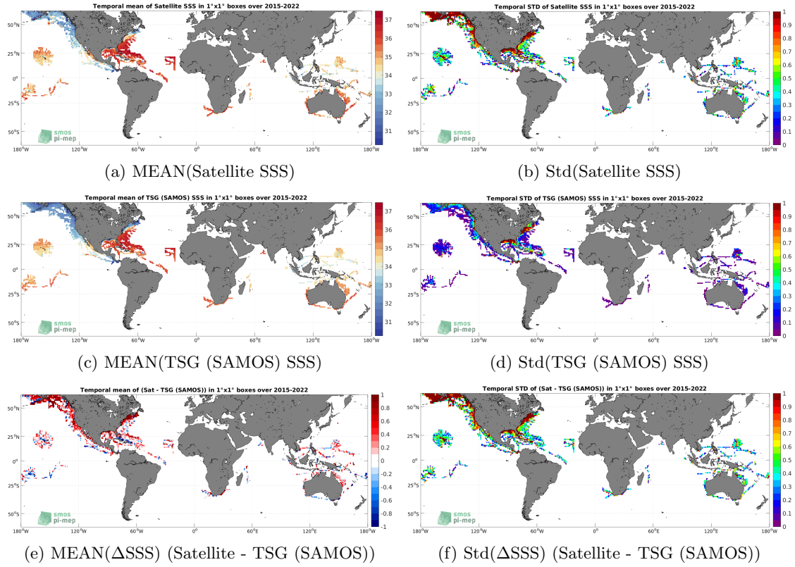
Figure 6: Temporal mean (left) and Std (right) of SSS from SMAP SSS L2 v5.0 (JPL) (top), TSG (SAMOS) (middle), and of \Delta SSS (Satellite - TSG (SAMOS)). Only match-up pairs are used to generate these maps.
