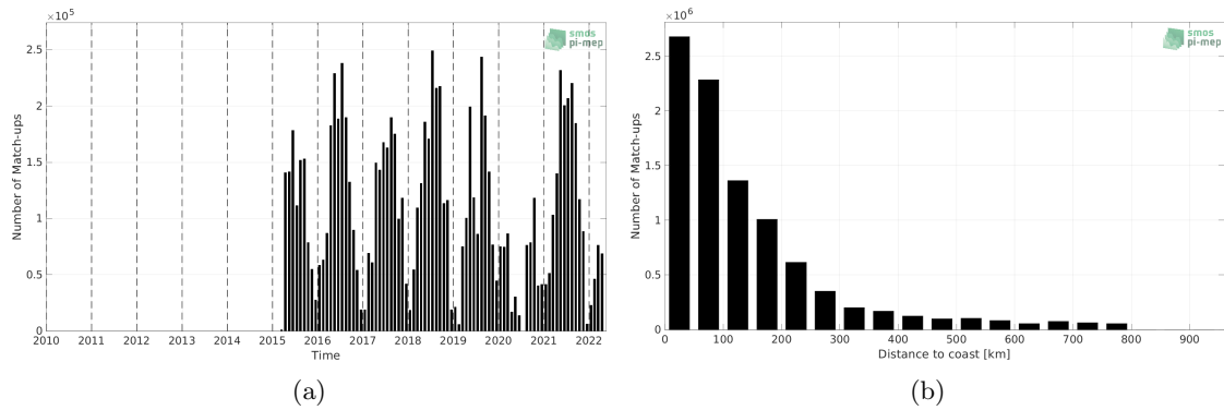
Figure 1: Number of match-ups between TSG (SAMOS) and SMAP SSS L2 v5.0 (JPL) SSS as a function of time (a) and as function of the distance to coast (b) over the SMOS coastal zone (<800km) 60N-60S Pi-MEP region and for the full satellite product period.
