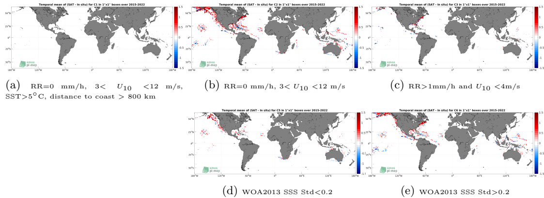
Figure 12: Temporal mean gridded over spatial boxes of size 1^\circ \times 1^\circ of \Delta SSS (SMAP SSS L2 v5.0 (JPL) - TSG (SAMOS)) for 5 different subdatasets corresponding to:RR=0 mm/h, 3 < U_{10} < 12 m/s, SST >5^\circ\text{C} , distance to coast > 800 km (a), RR=0 mm/h, 3 < U_{10} < 12 m/s (b), RR >1 mm/h and U_{10} < 4 m/s (c), WOA2013 SSS Std <0.2 (d), WOA2013 SSS Std >0.2 (e).
