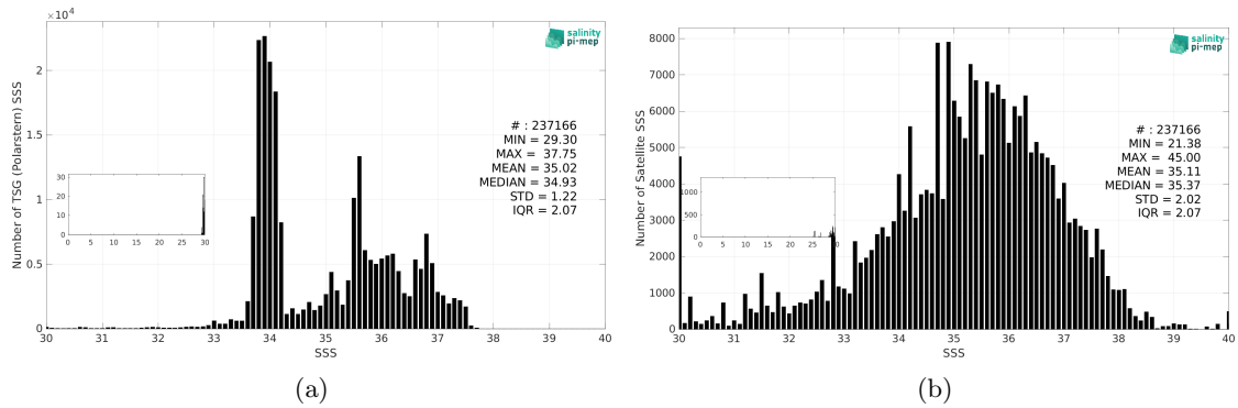
Figure 3: Histograms of SSS from TSG (Polarstern) (a) and SMAP SSS L2 v5.0 (JPL) (b) considering all match-up pairs per bins of 0.1 over the SMOS coastal zone (<800km) 60N-60S Pi-MEP region and for the full satellite product period.
