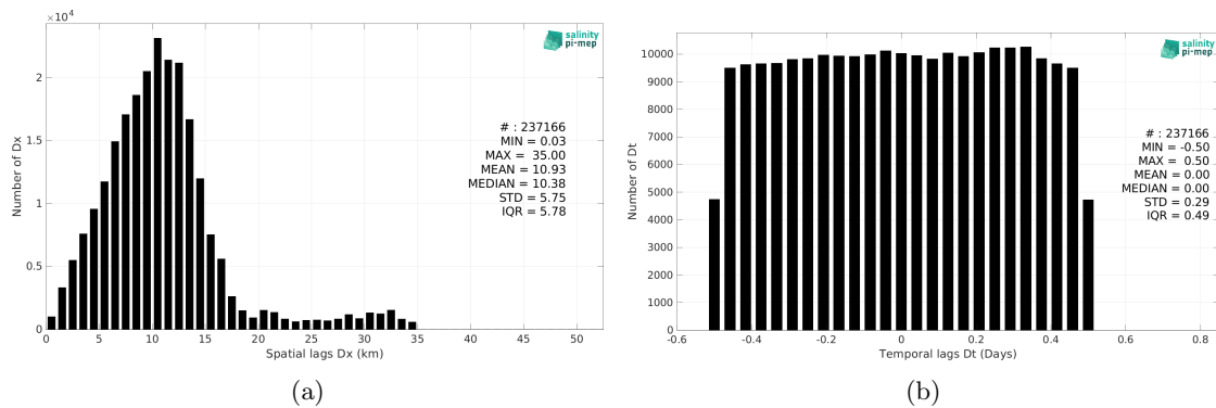
Figure 6: Histograms of the spatial (a) and temporal (b) lags between the location/time of the TSG (Polarstern) measurement and the date of the corresponding SMAP SSS L2 v5.0 (JPL) SSS pixel.
