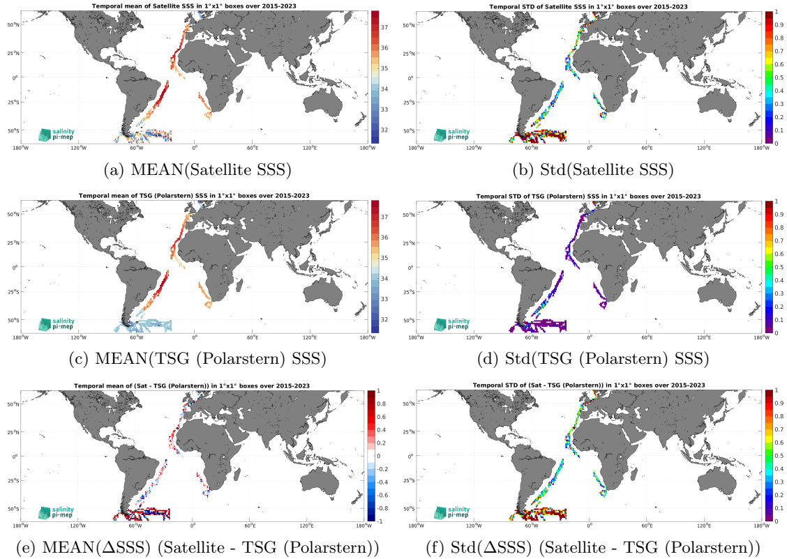
Figure 7: Temporal mean (left) and Std (right) of SSS from SMAP SSS L2 v5.0 (JPL) (top), TSG (Polarstern) (middle), and of \Delta SSS (Satellite - TSG (Polarstern)). Only match-up pairs are used to generate these maps.
