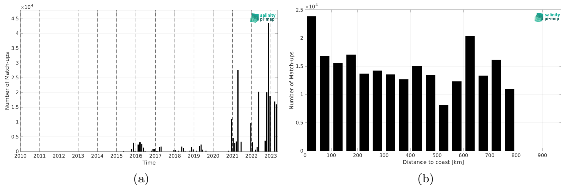
Figure 2: Number of match-ups between TSG (Polarstern) and SMAP SSS L2 v5.0 (JPL) SSS as a function of time (a) and as function of the distance to coast (b) over the SMOS coastal zone (<800km) 60N-60S Pi-MEP region and for the full satellite product period.
