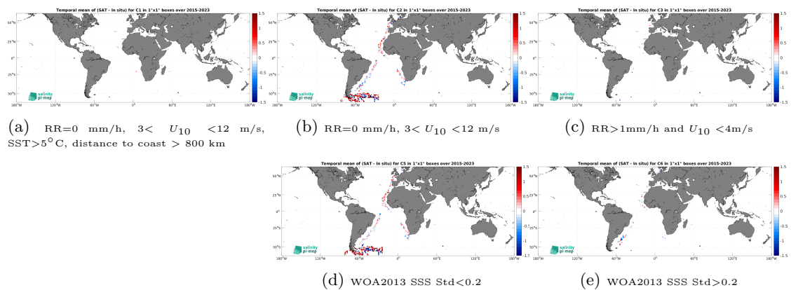
Figure 14: Temporal mean gridded over spatial boxes of size 1^\circ \times 1^\circ of \Delta\text{SSS} (SMAP SSS L2 v5.0 (JPL) - TSG (Polarstern)) for 5 different subdatasets corresponding to:RR=0 mm/h, 3 < U_{10} < 12 m/s, SST >5^\circ\text{C} , distance to coast > 800 km (a), RR=0 mm/h, 3 < U_{10} < 12 m/s (b), RR >1 mm/h and U_{10} < 4 m/s (c), WOA2013 SSS Std <0.2 (d), WOA2013 SSS Std >0.2 (e).
