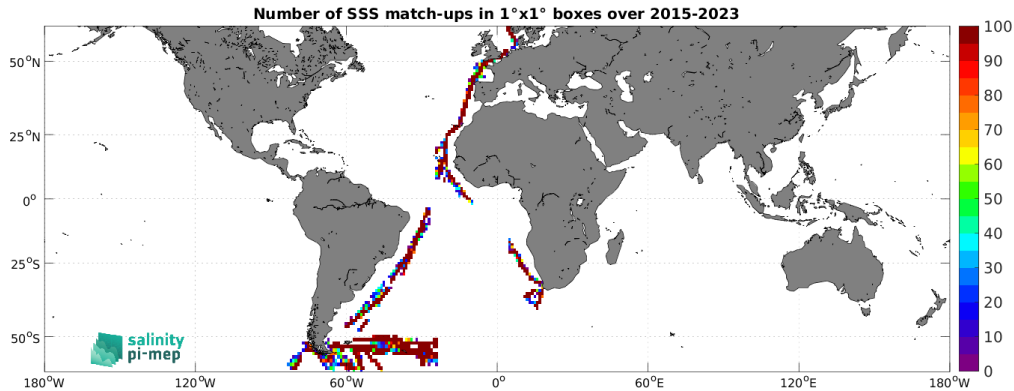
Figure 5: Number of SSS match-ups between TSG (Polarstern) SSS and the SMAP SSS L2 v5.0 (JPL) SSS product for the SMOS coastal zone (<800km) 60N-60S Pi-MEP region over 1^\circ \times 1^\circ boxes and for the full satellite product period.
