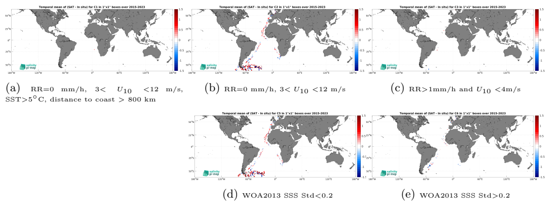
Figure 14: Temporal mean gridded over spatial boxes of size 1^\circ \times 1^\circ of \Delta SSS (SMAP SSS L2 v5.0 (JPL) - TSG (Polarstern)) for 5 different subdatasets corresponding to:RR=0 mm/h, 3 < U_{10} < 12 m/s, SST >5^\circ\text{C} , distance to coast > 800 km (a), RR=0 mm/h, 3 < U_{10} < 12 m/s (b), RR >1 mm/h and U_{10} < 4 m/s (c), WOA2013 SSS Std <0.2 (d), WOA2013 SSS Std >0.2 (e).
