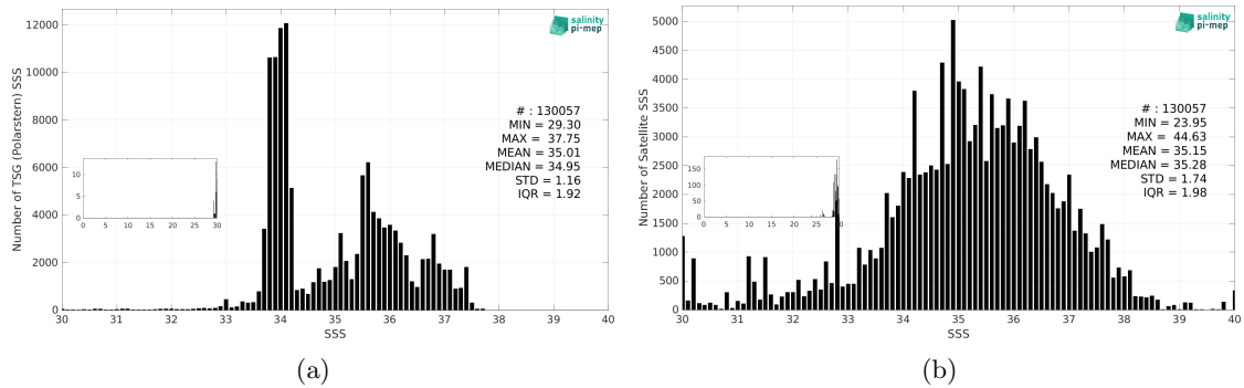
Figure 3: Histograms of SSS from TSG (Polarstern) (a) and SMAP SSS L2 v5.0 (JPL) (b) considering all match-up pairs per bins of 0.1 over the SMOS coastal zone (<800km) 60N-60S Pi-MEP region and for the full satellite product period.
