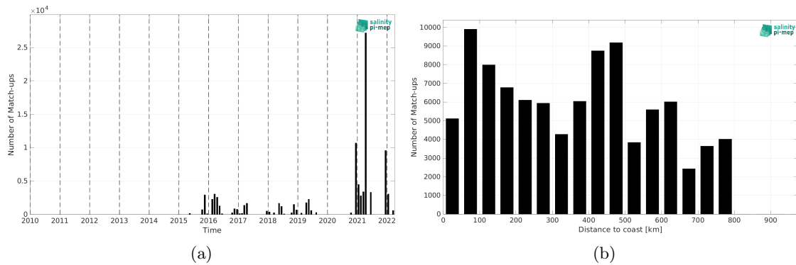
Figure 1: Number of match-ups between TSG (Polarstern) and SMAP SSS L2 v5.0 (JPL) SSS as a function of time (a) and as function of the distance to coast (b) over the SMOS coastal zone (<800km) 60N-60S Pi-MEP region and for the full satellite product period.
