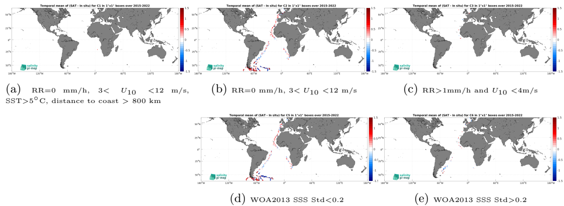
Figure 12: Temporal mean gridded over spatial boxes of size 1^\circ \times 1^\circ of \Delta\text{SSS} (SMAP SSS L2 v5.0 (JPL) - TSG (Polarstern)) for 5 different subdatasets corresponding to:RR=0 mm/h, 3 < U_{10} < 12 m/s, SST >5^\circ\text{C} , distance to coast > 800 km (a), RR=0 mm/h, 3 < U_{10} < 12 m/s (b), RR >1 mm/h and U_{10} < 4 m/s (c), WOA2013 SSS Std <0.2 (d), WOA2013 SSS Std >0.2 (e).
